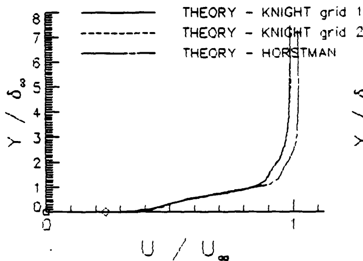
Fig. 19 Computed Velocity in x-direction at x = 11\delta_\infty , z-z_{fin} = 6\delta_\infty
