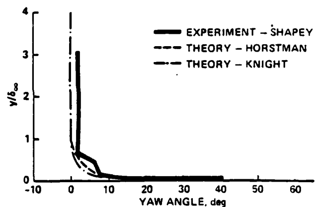
Fig. 11 Yaw Angle at Station 3
