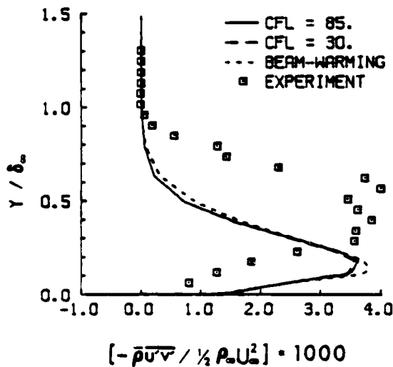
Fig. 16 - Reynolds shear stress at X/\delta_\infty = 5.4 for Mach 2.83 flow over 16 deg ramp.
