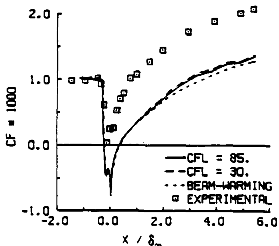
Fig. 6 - Skin friction for Mach 2.83 flow over 16 deg ramp.
