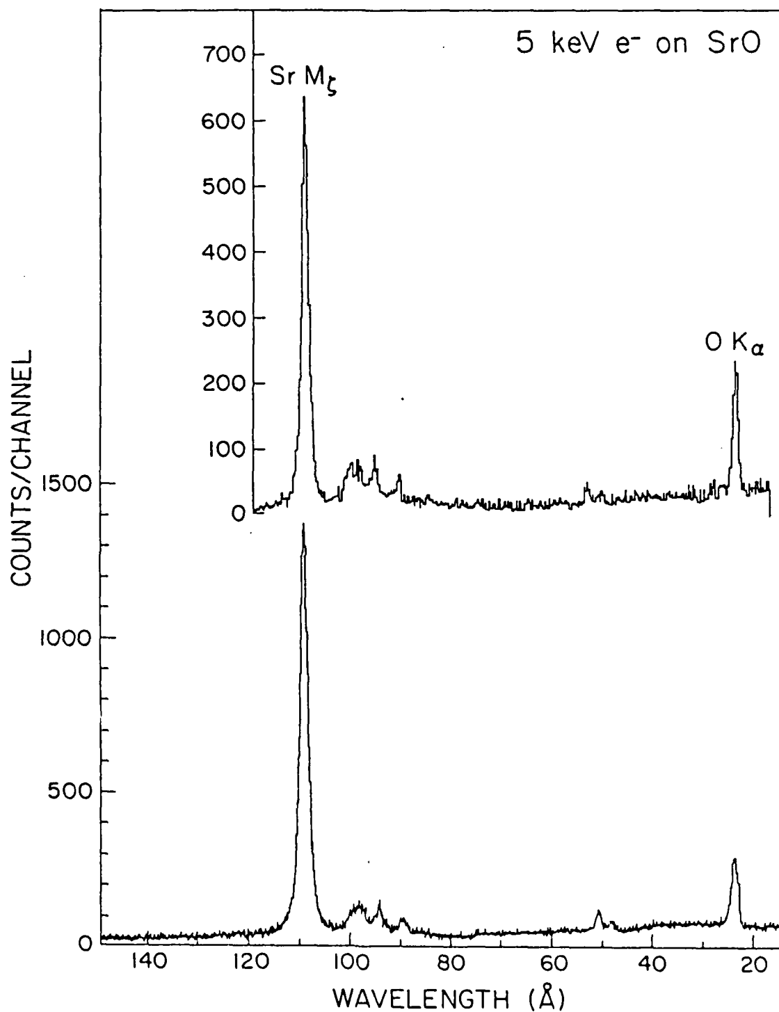
Fig. 22. Comparison of a SrO M \xi spectrum acquired with a CEM detector over 70 minutes (upper spectrum) with a composite of two MCP spectra of 7 minutes each (lower spectrum).
