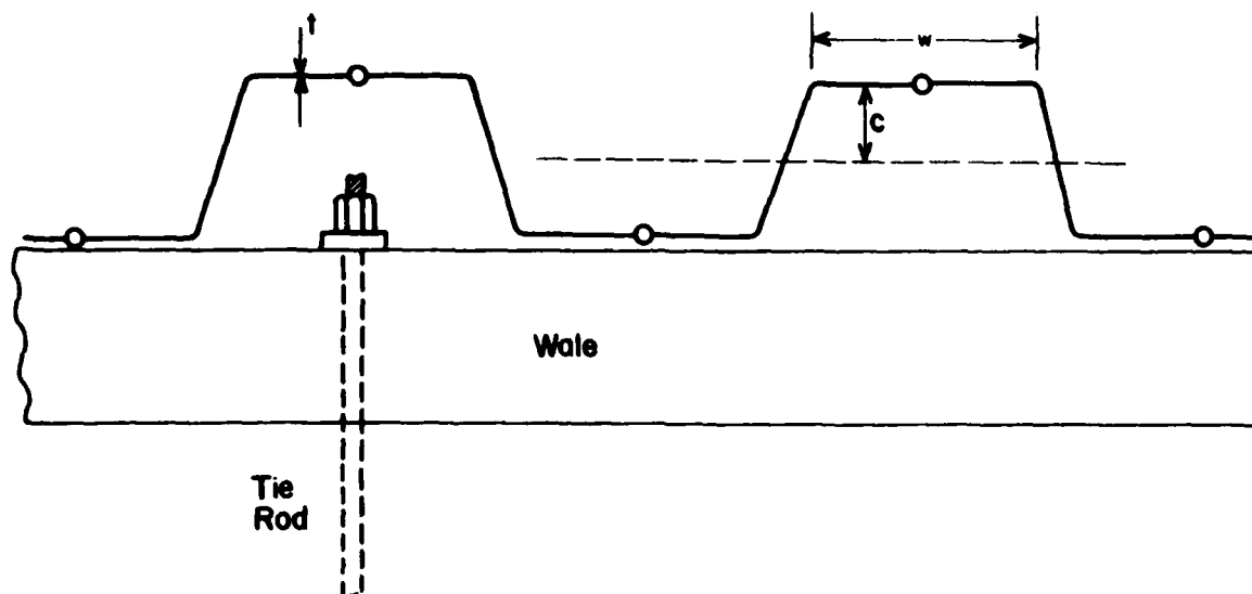
Figure 28. Horizontal section of sheet piling guide wall.
