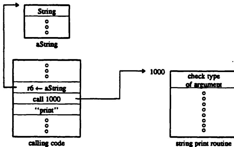
Figure 3.9: Caching the target address in the instruction stream. The next time the call is executed, control goes directly to the string print routine. A prologue checks that the current argument's type matches the contents of the word following the call instruction. This word contains the type that the argument had the previous time the call was executed. If the types match, control falls through to the string print routine, otherwise another table lookup is needed.
