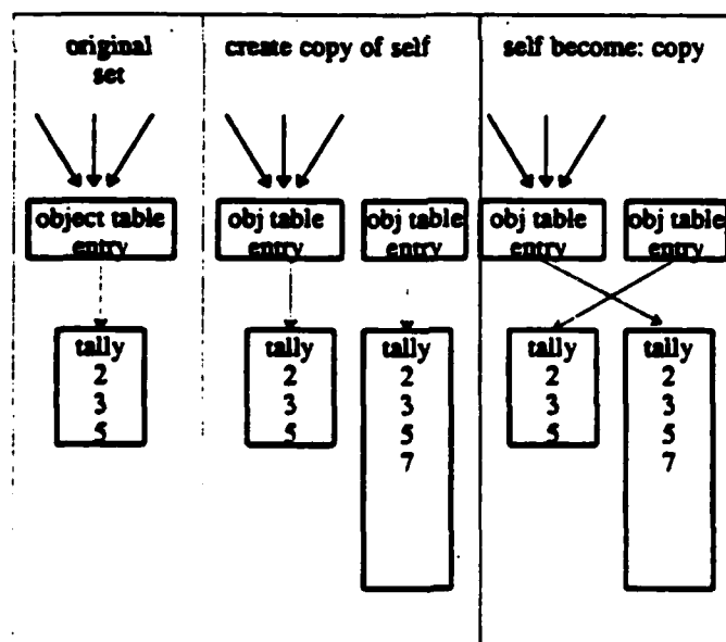
Figure 5.9: Growing with become. The sequence above illustrates how a Smalltalk-80 set employs become to grow. Initially, the set is {2, 3, 5} and we attempt to add 7 to it. The set creates a larger copy of itself and uses become to replace the original set with the larger version.
