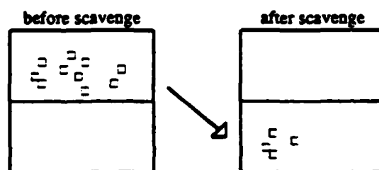
Figure 5.4: Baker semispaces. The Baker storage reclamation algorithm divides memory into semispaces. When one fills up, the live objects in it are copied to the other semispaces.
