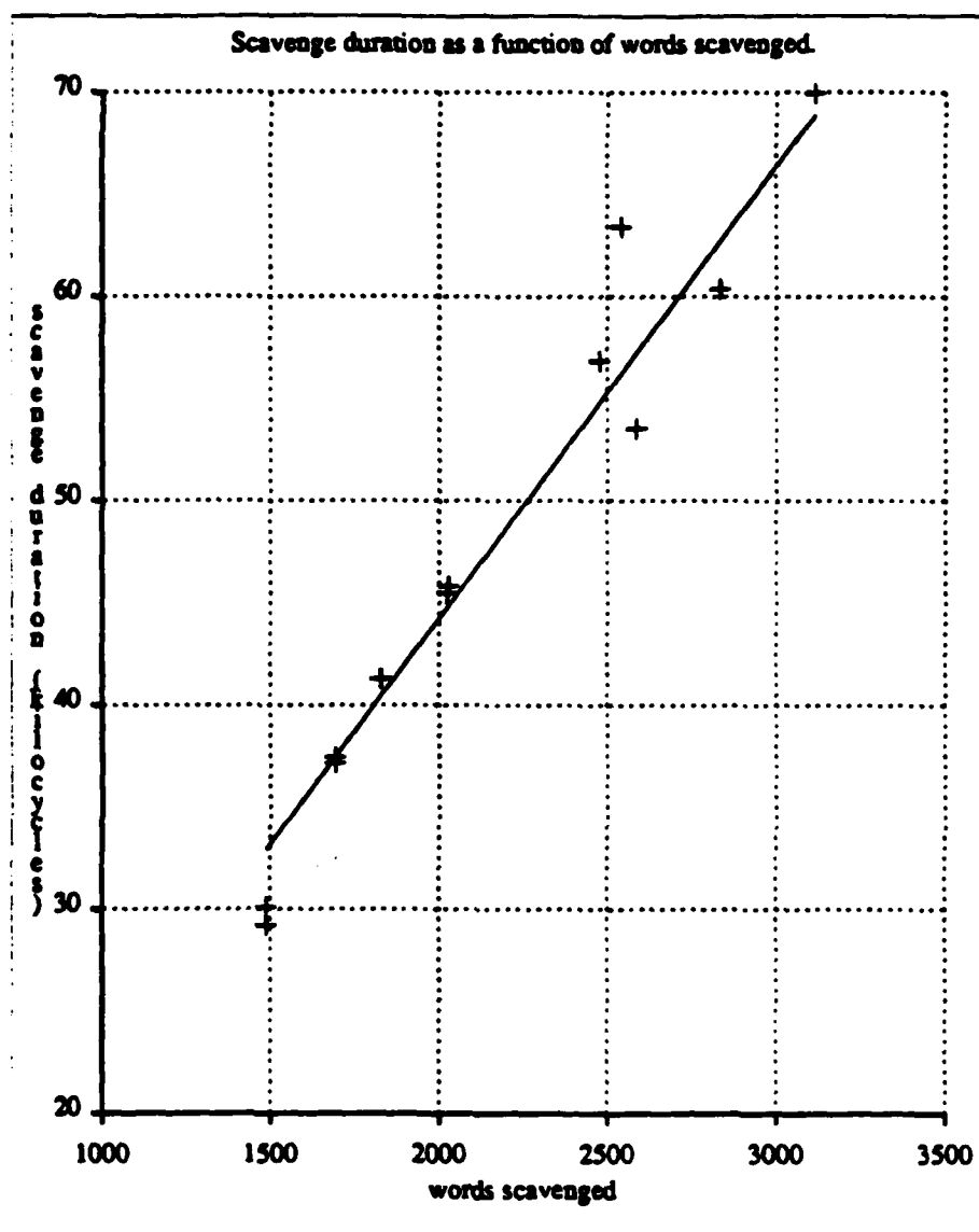
Figure 5.8: Predicting the duration of a scavenge. This graph shows that scavenge duration can be predicted from the number of words scavenged.
