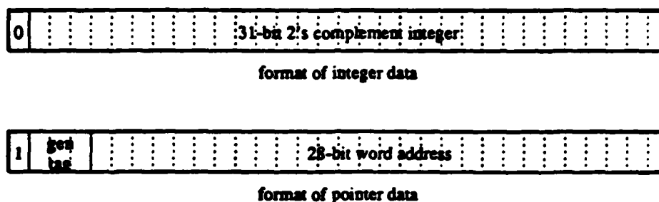
Figure 3.1: SOAR tagged data types. SOAR supports two data types, 31-bit signed integers and 28-bit pointers. Pointers include a generation tag (as explained in Section 3.5.1). SOAR words could have contained 32 bits of data plus one bit of tag for a total of 33 bits. The scarcity of 33-bit tape drives, disk drives, and memory boards led us to shorten our words to a total of 32 bits including the tag (31 bits of data).
