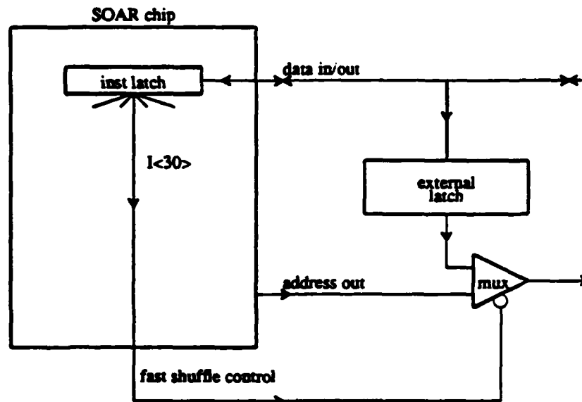
Figure 3.10: Fast Shuffle logic. When a call or jump is fetched from memory, the next instruction is prefetched based on the external address latch instead of the PC.
