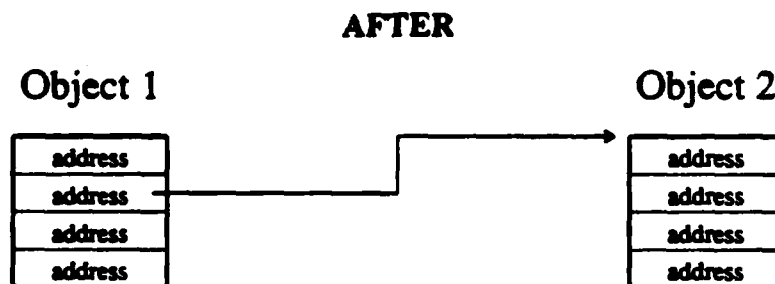
Figure 3.12: Direct addressing. A SOAR pointer contains the virtual address of the target object. This is the fastest way to follow pointers.
