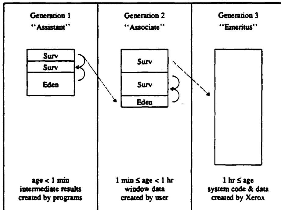
Figure 6.2: Diagram of a system with a middle generation. Objects are created in the Eden area of the Assistant generation. If an object lives through several scavenges in the Assistant survivor areas, it gets promoted into the Associate Eden area. If it then survives scavenges between the Associate survivor areas, the object receives tenure into the Emeritus area, where it is exempt from online reclamation. Ideally, the parameters would be set to keep short-lived objects representing intermediate results in Generation 1, medium-lifetime objects used by windows in Generation 2, and long-lived objects like the square root routine in the Old generation.
