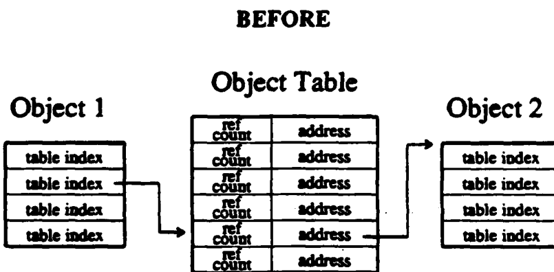
Figure 3.11: Indirect addressing. In traditional Smalltalk-80 systems, each pointer is really a table index. The table entry contains the target's reference count and memory address. This indirection required previous Smalltalk-80 systems to dedicate base registers to frequently accessed objects. The overhead to update these registers slowed each procedure call and return.
