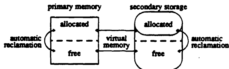
Figure 5.1: Virtual memory vs. automatic storage reclamation.
