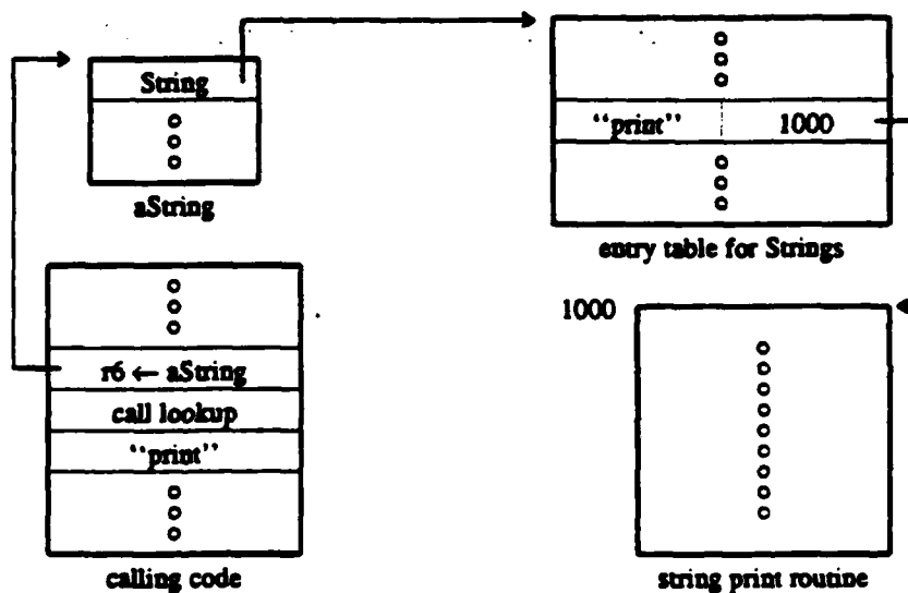
Figure 3.8: Caching the target address in the instruction stream. In this example, the print routine is called with an argument that is a string. (The argument is passed in r6 .) The first time the call instruction is executed, the call contains the address of a lookup routine and the word after the call contains a pointer to the name "print" . The lookup routine follows the pointers to the entry table for strings, and finds the entry for "print" . It then overwrites the call instruction with a call to that routine and replaces the word after the call with the type of the argument (string).
