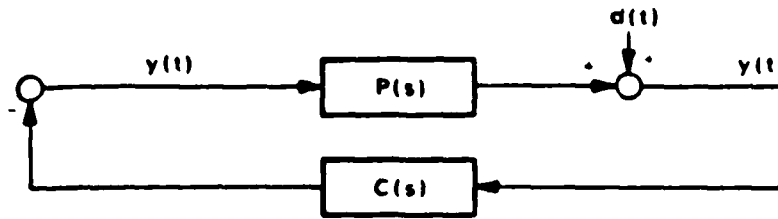
Figure 6: Vibration Suppression Control System.
