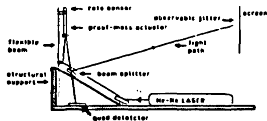
Fig. 4 Laser pointing and jitter control experimental apparatus.
