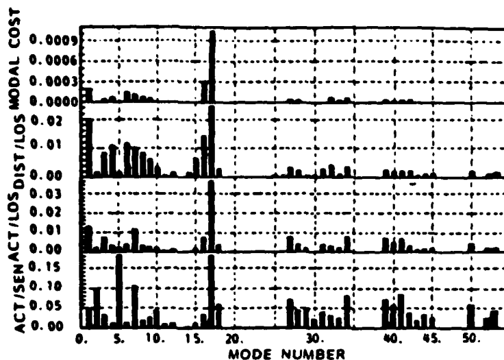
Figure 9: Open Loop Modal Analysis.
