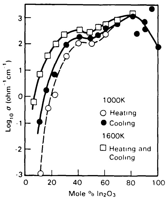
Figure 4.20 \log(\sigma) at 1000 and 1600K as a Function of In_2O_3 Content
