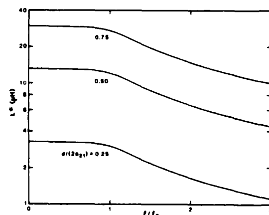
FIG. 3. Dependence of L^* upon cylinder length and diameter. The pickup coil parameters are: a_{21} = 11.9 \text{ mm} , a_{22} = 13.3 \text{ mm} , l_2 = 127 \text{ mm} , N_2 = 6042 , z_s = 0 .
