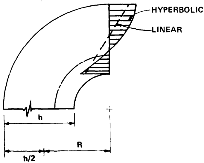
Figure 2. Comparison of stress calculations, with and without consideration for curvature
