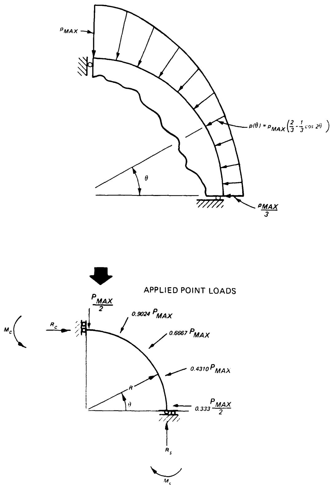
Figure 15. 1-D idealization of RC conduit
