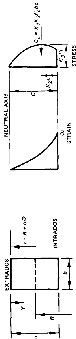
b. NEGATIVE-MOMENT SECTION
