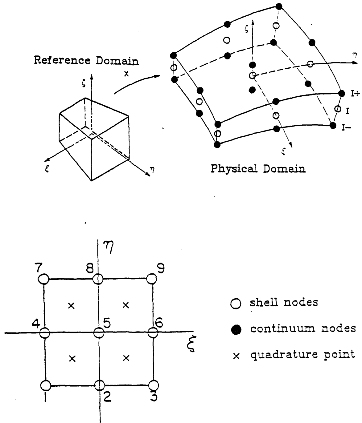
Figure A1. Shell element nomenclature.
