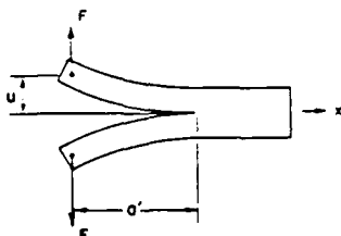
Figure 2. Double-cantilever beam (DCB) for delamination fracture studies.
