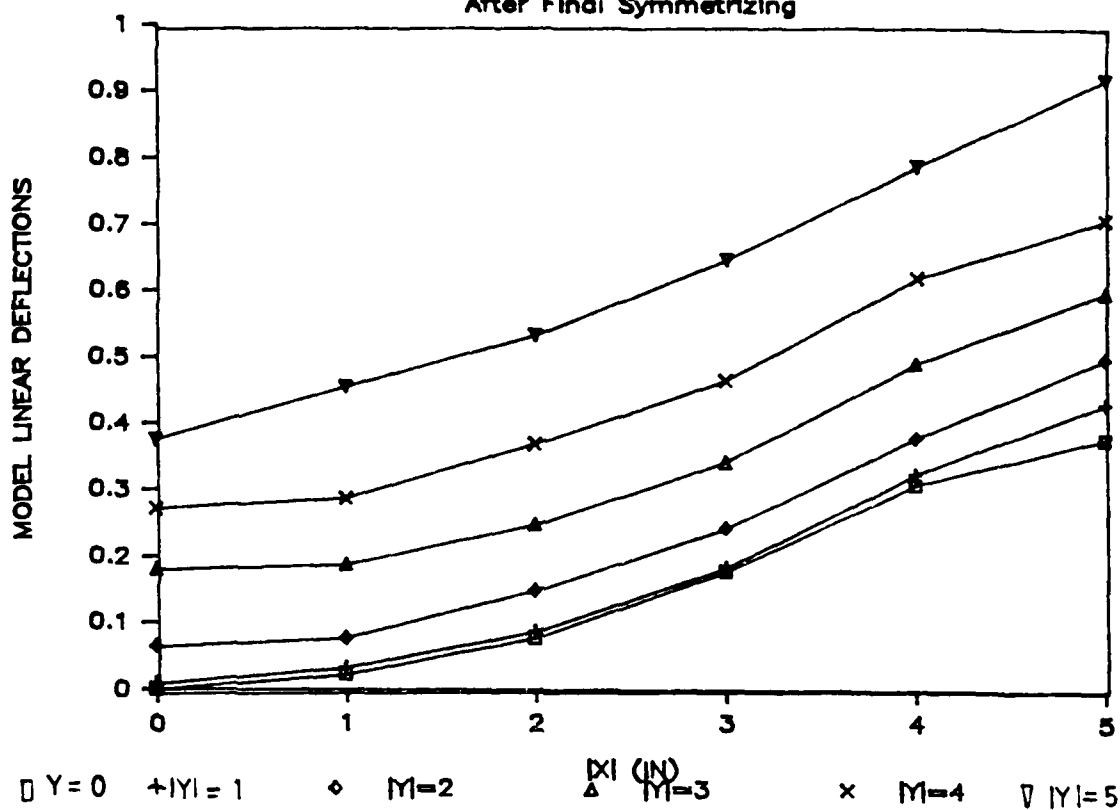
Figure 5.3.1-5: Model Deflections
