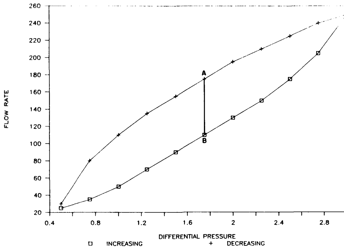
Figure 9. Hysteresis example.
