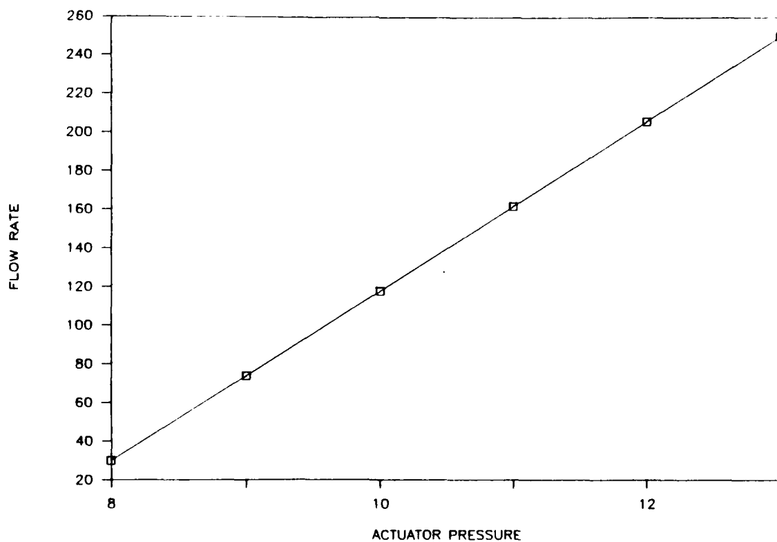
Figure 8. Ideal linearity.
