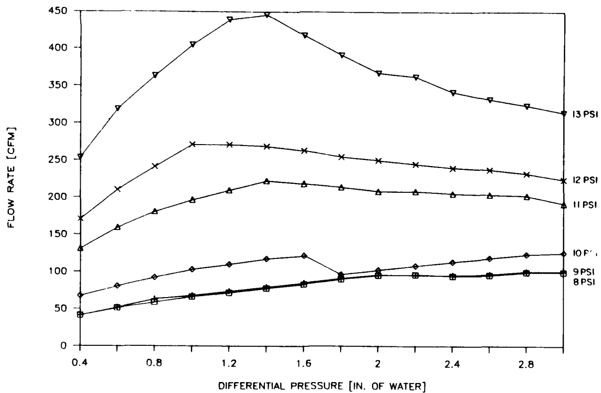
Figure 10. Pressure independence, manufacturer A.
