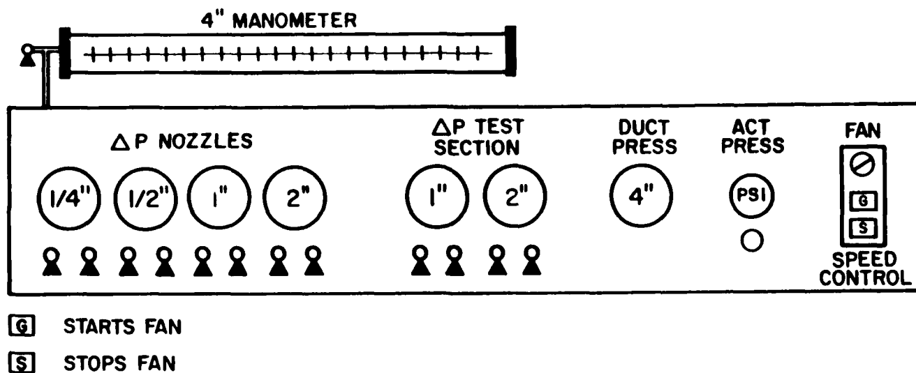
Figure 7. Testing apparatus control panel.
