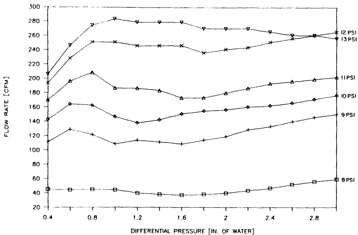
Figure 12. Pressure independence, manufacturer C.
