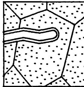
MEDIUM STRESS INTENSITY QUASI-CLEAVAGE
