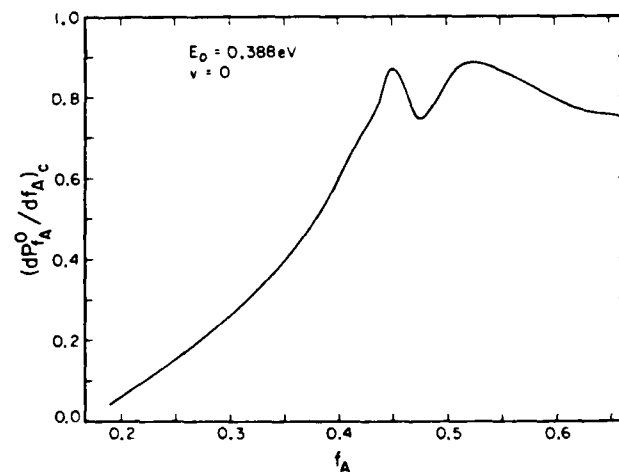
FIG. 18. Partitioning probability (dP_A^0/df_A) , (see Sec. II) as a function of energy fraction f_A of atom A for dissociation in collisions of ground state molecules at a reagent translational energy E_0 of 0.388 eV.
