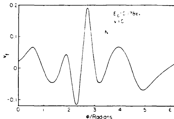
FIG. 10. Final action v_f as a function of initial phase \Phi for a collision involving ground state molecules at a reagent translational energy E_i of 0.178 eV. All markings are as in Fig. 7. Note the expanded scale of the ordinate.
