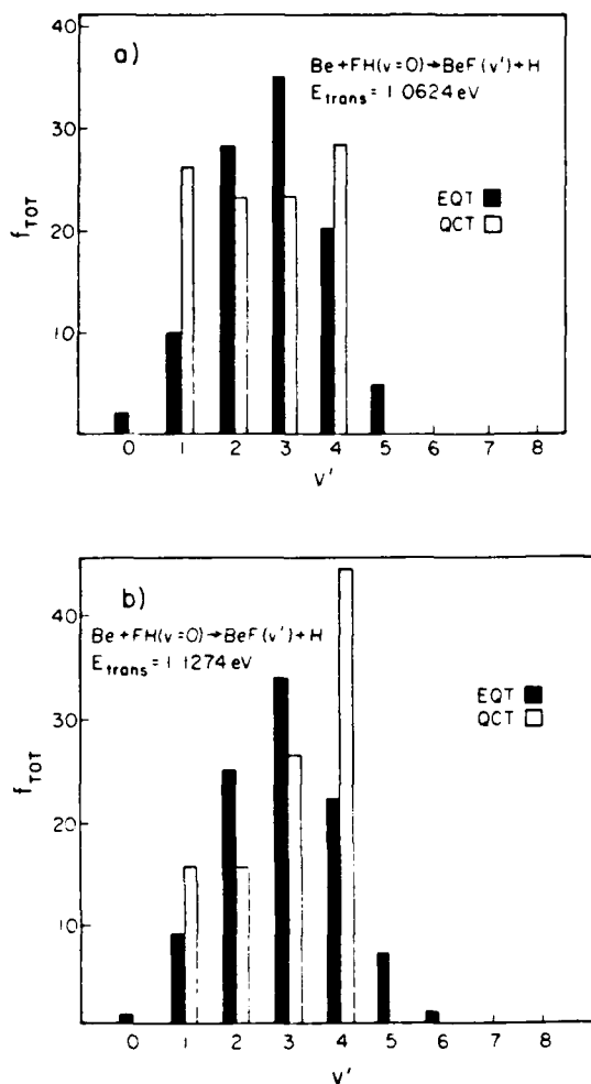
Fig. 3. Product vibrational state distribution of BeF formed in the reaction \text{Be} + \text{FH}(v=0) \rightarrow \text{BeF}(v') + \text{H} for energies shown. Open bars are quasi-classical trajectory values taken from the results of Schor et al. [11], while solid bars are from the quantum-mechanical calculations.
