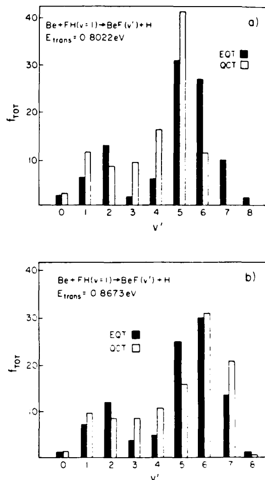
Fig. 4. Product vibrational state distribution of BeF formed in the reaction \text{Be} + \text{FH}(v=1) \rightarrow \text{BeF}(v') + \text{H} for energies shown. Symbols are as in fig. 3.
