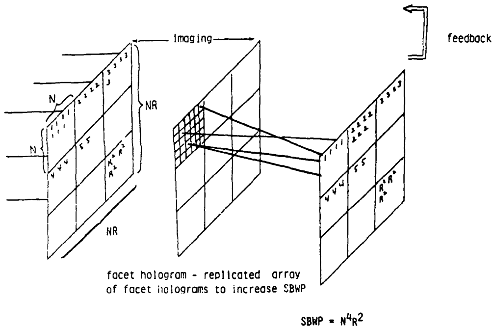
Fig. 2.4-3. Block mode cellular logic interconnection.
