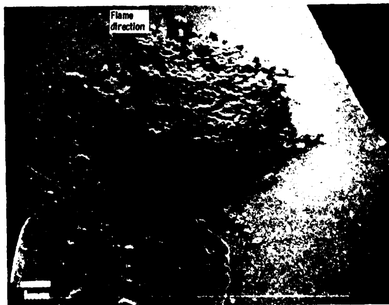
Figure 4. - SEM micrograph of single crystal \text{SiC} surface after 1 hr oxidation at 1375^\circ\text{C} in the Mach 1 burner rig.
