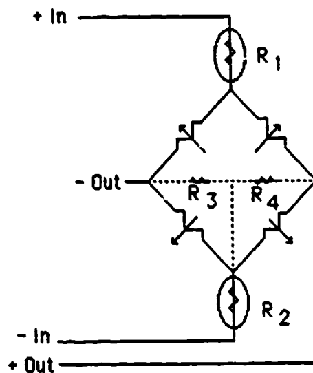
Figure 3.2: Schematic Diagram of the 4-Arm Bridge of the Sensors.
