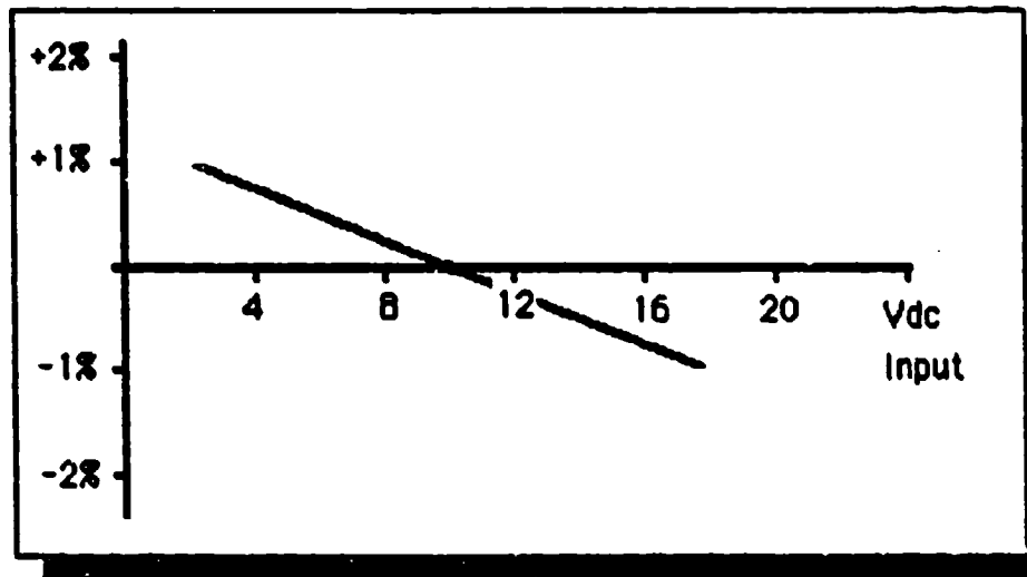
Figure 3.3: Typical Transducer Sensitivity Shift (mV/Pa/Input Volt) Due to Varying Supply Voltage.
