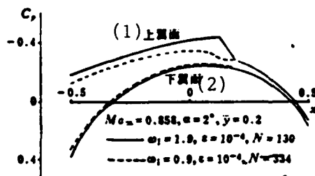
Fig. 4. Influence of relaxation parameters on computed results Key: (1) upper wing surface; (2) lower wing surface.
