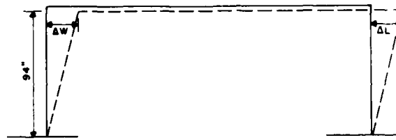
DEFLECTIONS RECORDED, SYSTEM A
