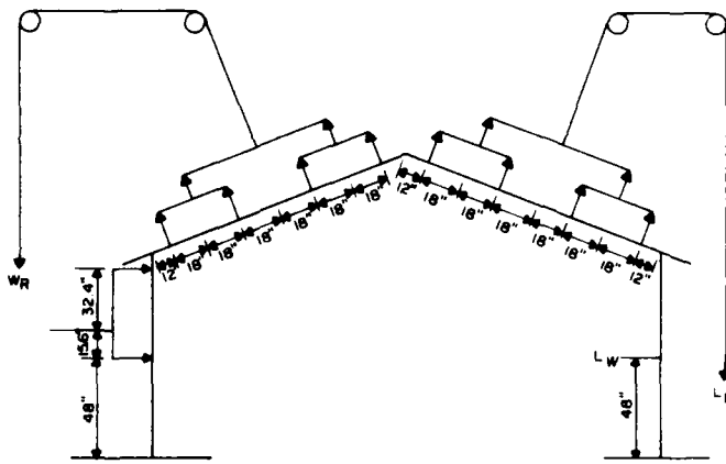
TEST LOADING, SYSTEMS B AND C
