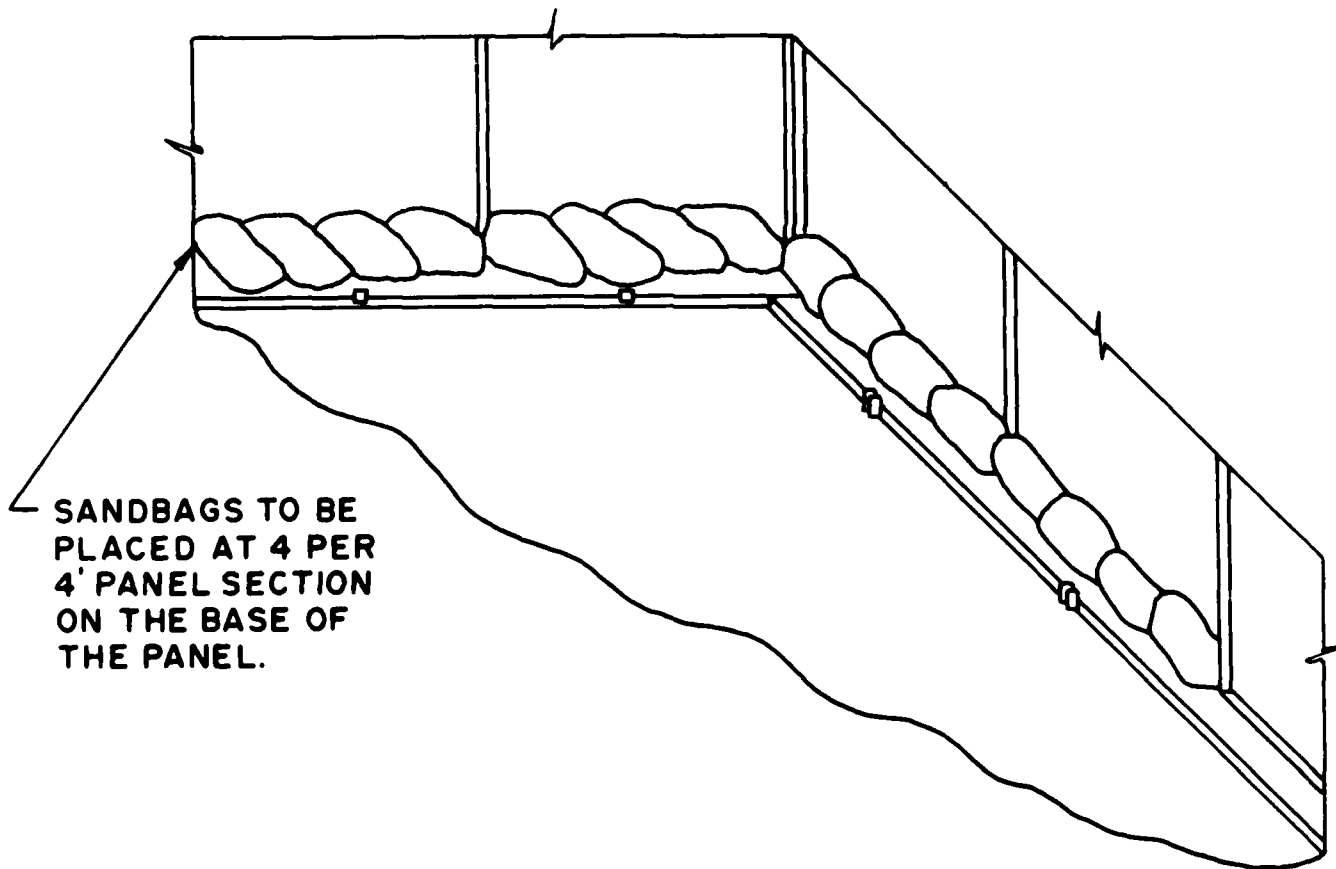
Figure 39. Sandbag foundation.
