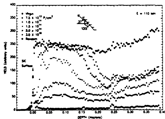
Fig. 1a. 2.5 MeV He RBS/channeling spectra for RT P-implanted \beta -SiC showing the accumulation of damage along the \langle 110 \rangle axial direction with an increasing P dose.
