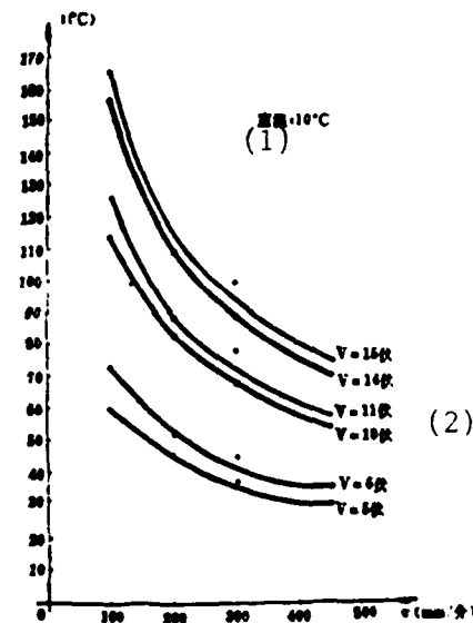
Fig. 7. No. 2 propellant outer surface t \sim v relationship curves Key: (1) Room temperature: 10^{\circ}\text{C} ; (2) volt.
