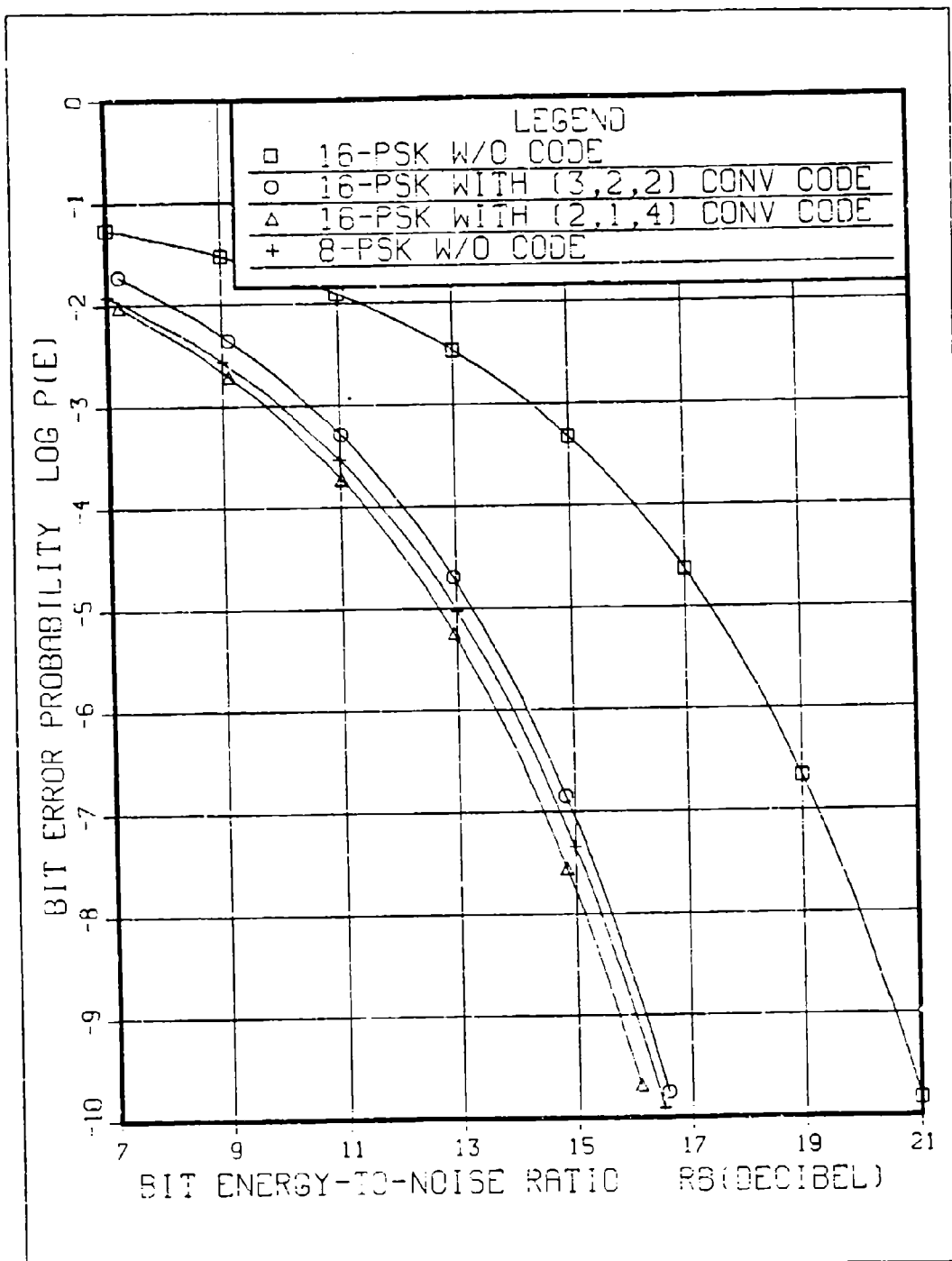
Figure 4.7 Bit error rates of 16-PSK with and without convolutional codes Q = 8
