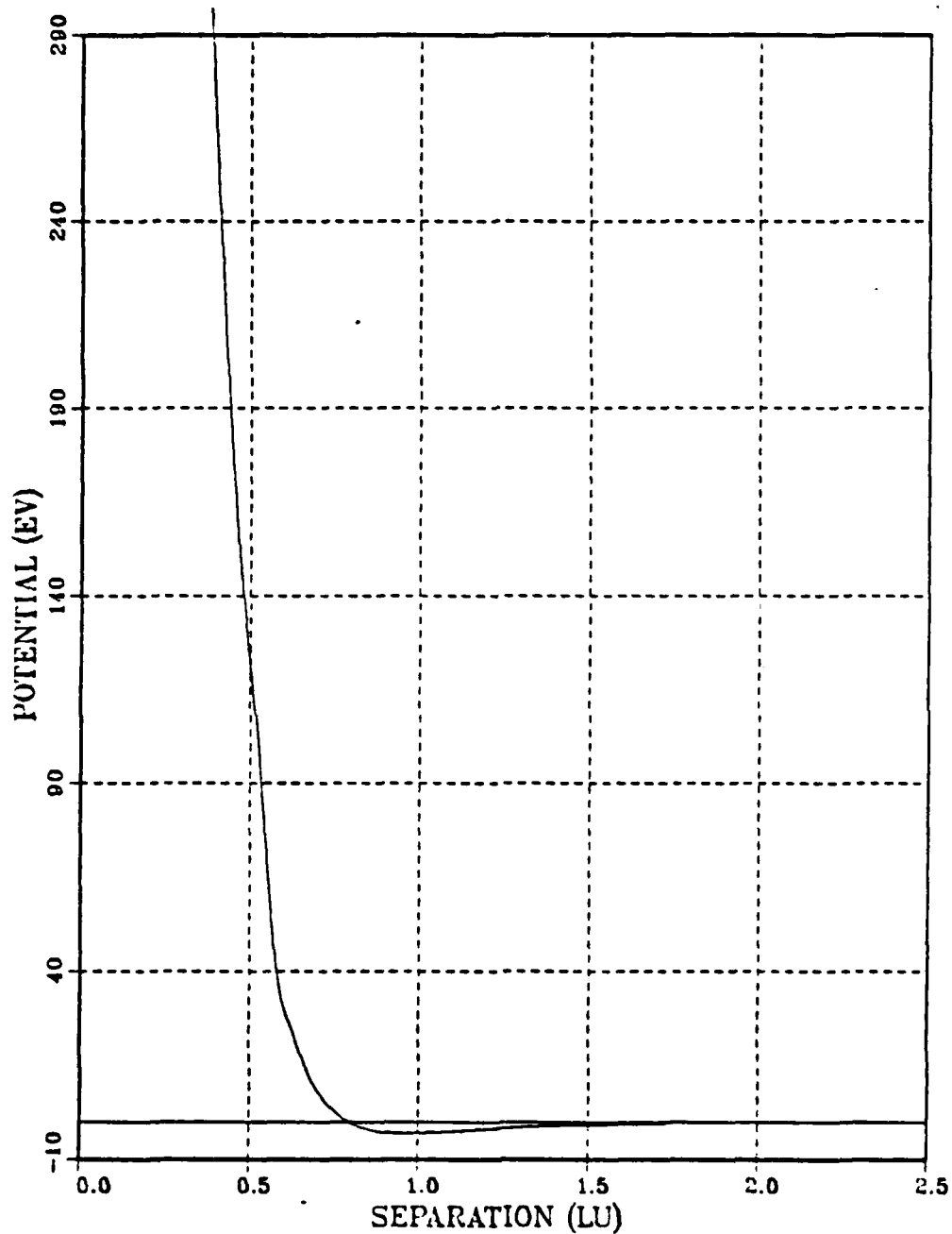
Fig. 7. Molybdenum-Nirtogen potential function
