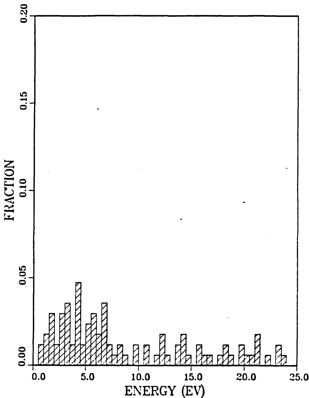
Fig. 22. Ejected nitrogen atom energy distribution from a tungsten target assuming Argon energy of 2 keV and adatom location of -0.05 LU
