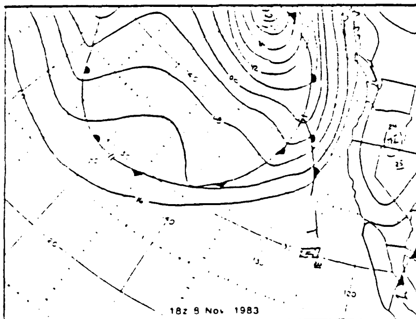
Fig. 3.31 8 November 1983 Surface Charts a) 1200GMT (top), b) 1800GMT (bottom).
