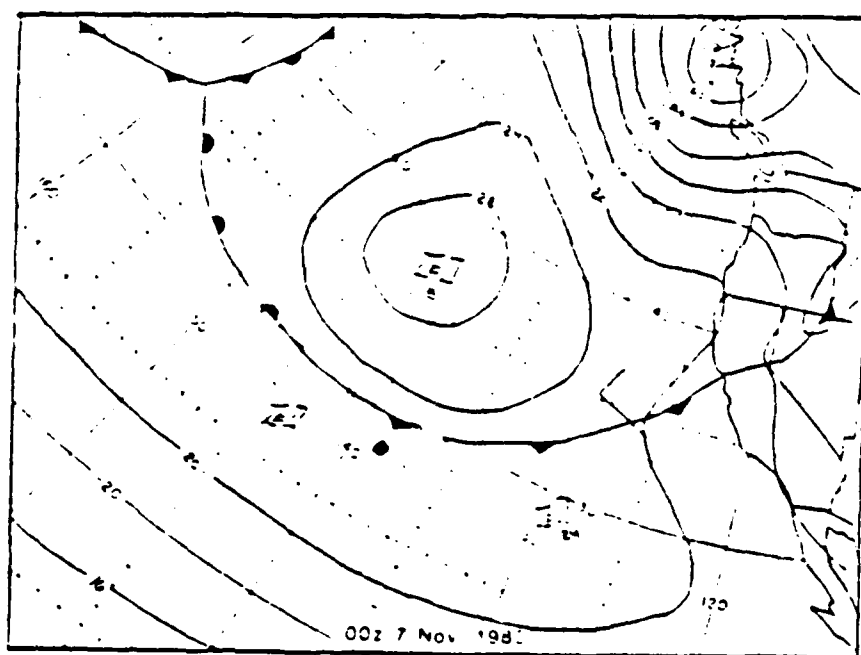
Fig. 3.28 6 - 7 November 1983 Surface Charts a) 6/1800GMT (top), b) 7/0000GMT (bottom).
