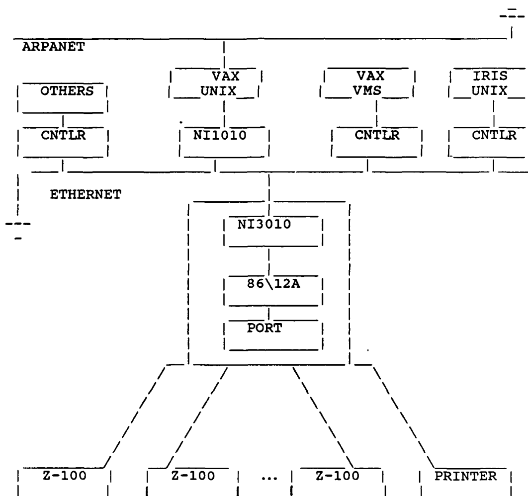
Figure 1.1 System Network Configuration
