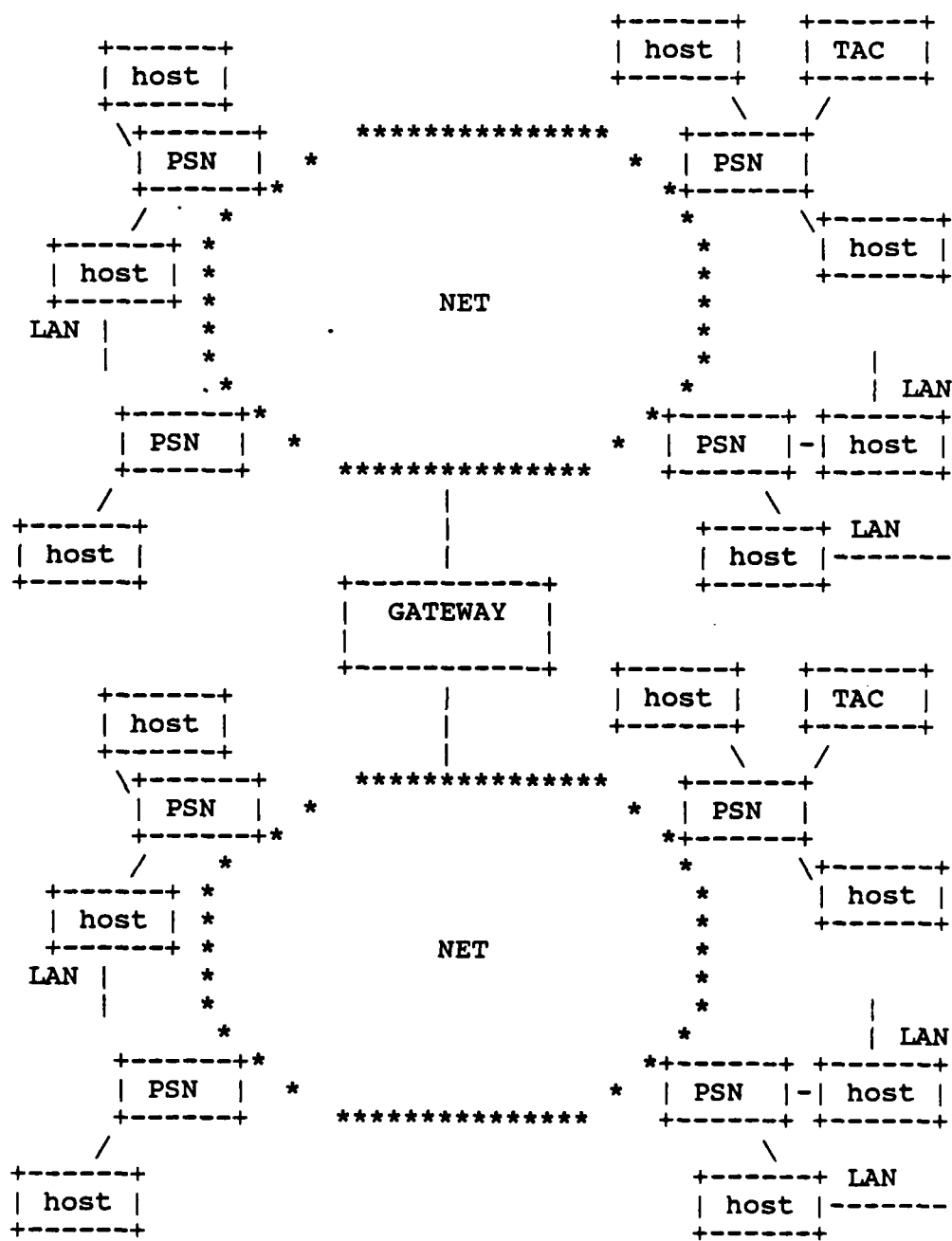
FIGURE 2.1 DDN ARCHITECTURE
