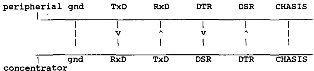
Figure 6.1 Serial Port Cable Pin Connections
