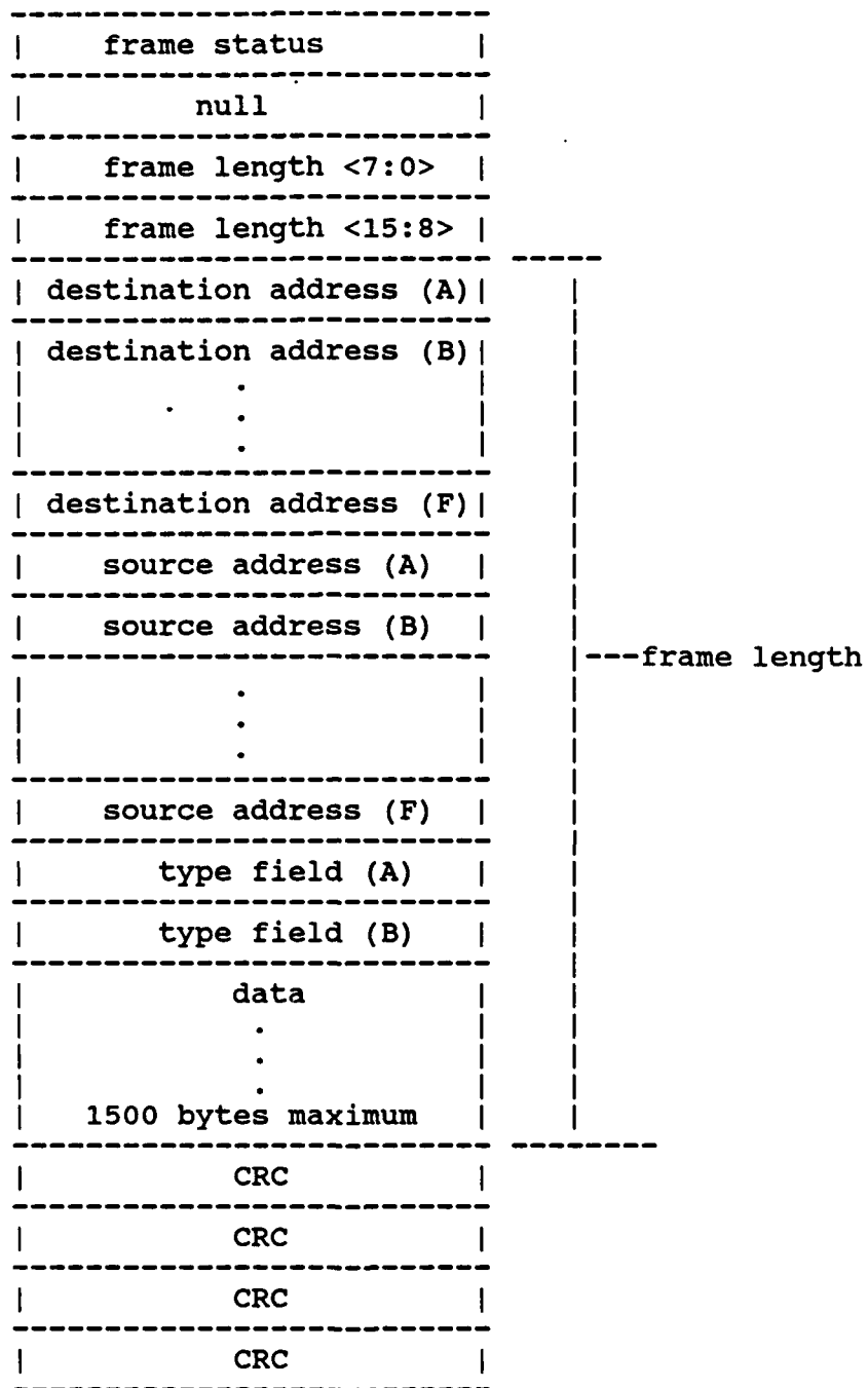
Figure 2.7 Receive Data Block in MULTIBUS Memory
