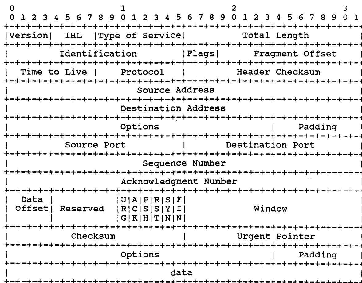
Figure 3.1 TCP/IP protocol headers
