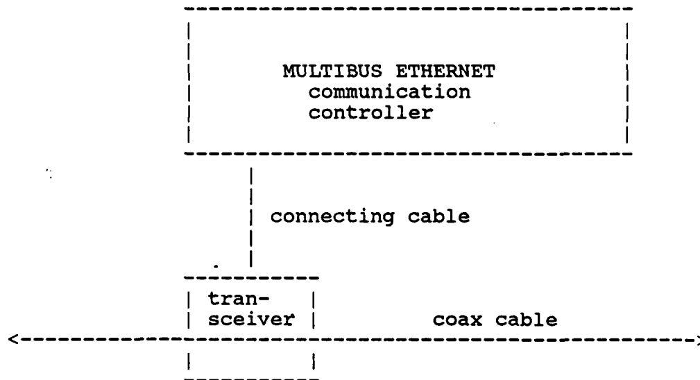
Figure 2.5 MULTIBUS/ETHERNET Connection
