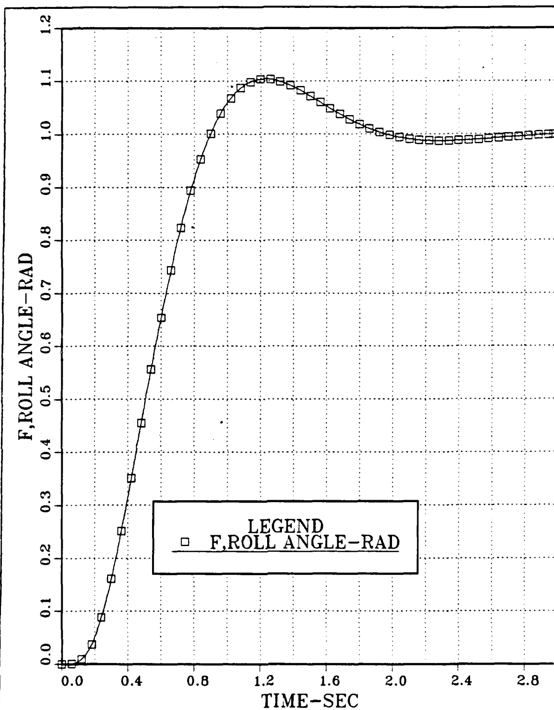
Figure 4.28 Roll Angle vs. Time; Uncoupled Modified Roll Channel with \delta_1 , \delta_2 and \delta_3 Centered; Continuous Open Loop System; Step Input: \psi_c = 1 rad and \delta_1, \delta_2, \delta_3, \delta_4 = 0 ; a_0 = 0 .
