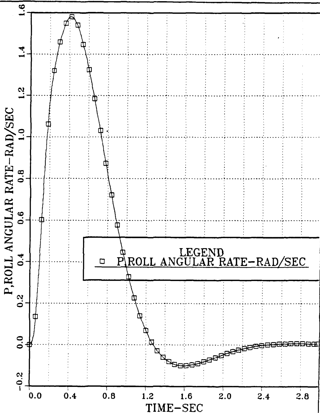
Figure 4.21 Roll Angular Rate vs. Time; Uncoupled Modified Roll Channel with \delta_1 Centered; Continuous Open Loop System; Step Input: \psi_c = 1 rad and \delta_{1c}\delta_{2c}\delta_{3c}\delta_{4c} = 0 ; a_0 = 0 .
