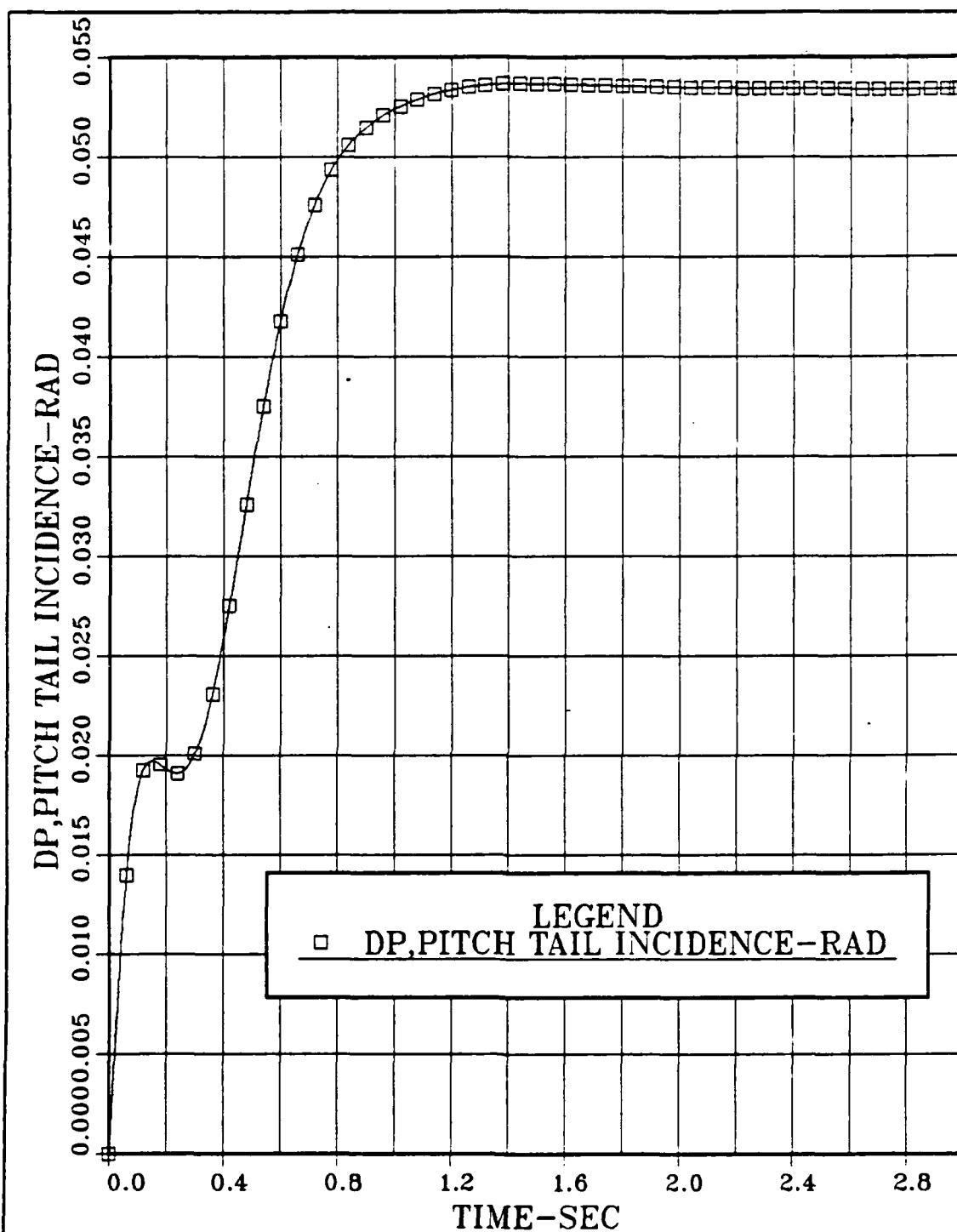
Figure 3.24 Pitch Tail Incidence vs Time; Inoperative \delta_1 Control Surface; a_g=0 ; Step input: n_{zc} = 1 gee, \delta_{1c} = 0.2 , \delta_{2c} , \delta_{3c} , \delta_{4c} = 0 rad.
