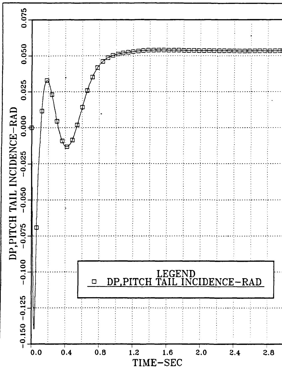
Figure 3.16 Pitch Tail Incidence vs. Time; Hard Over \delta_1 Control Surface; a_e=0 ; Step Input: n_{zc}=1 gee, \delta_{1c}=0.2 rad, \delta_{2c} \delta_{3c} \delta_{4c}=0 .
