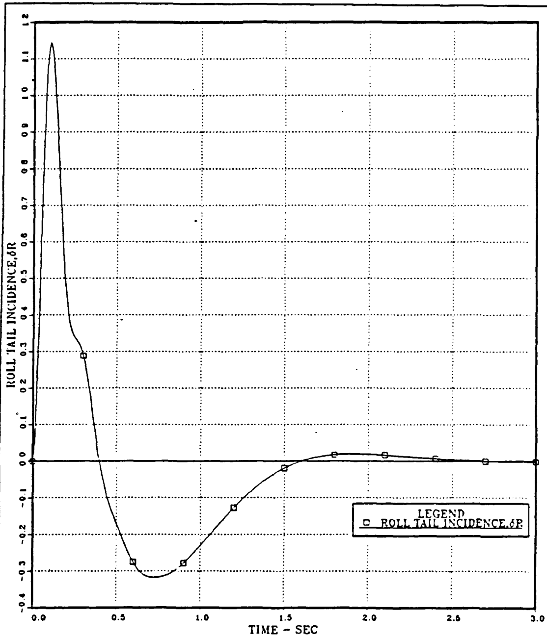
Figure 4.11 Roll Tail Incidence vs. Time; Uncoupled Roll Channel; Continuous Open Loop System; Circular Airframe; Step Input \psi_c = 1 rad; a_n = 0 .
