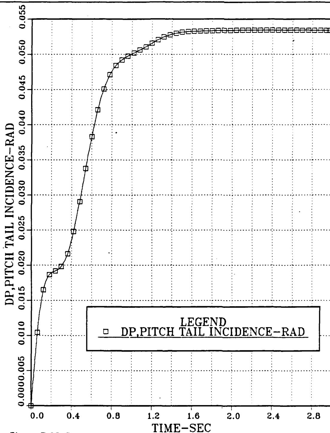
Figure 3.28 Pitch Tail Incidence vs Time; Inoperative \delta_1 and \delta_2 Control Surfaces; a_0=0 ; Step input: n_{zc} = 1 gee, \delta_{1c} = 0.2 , \delta_{2c} = \delta_{3c} = \delta_{4c} = 0 rad.
