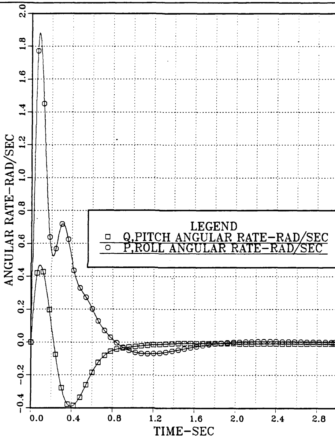
Figure 5.14 Hard Over \delta , Type of Impairment: Pitch and Roll Angular Rate vs. Time; Combined Pitch and Roll Channels; Continuous Open Loop System; Step Inputs: \delta_{1c}=0.2\text{rad} , \delta_{2c} , \delta_{3c} , \delta_{4c}=0 and N_{2c}=1\text{ gee} , \psi_c=1\text{ rad} ; \delta_e=0 .
