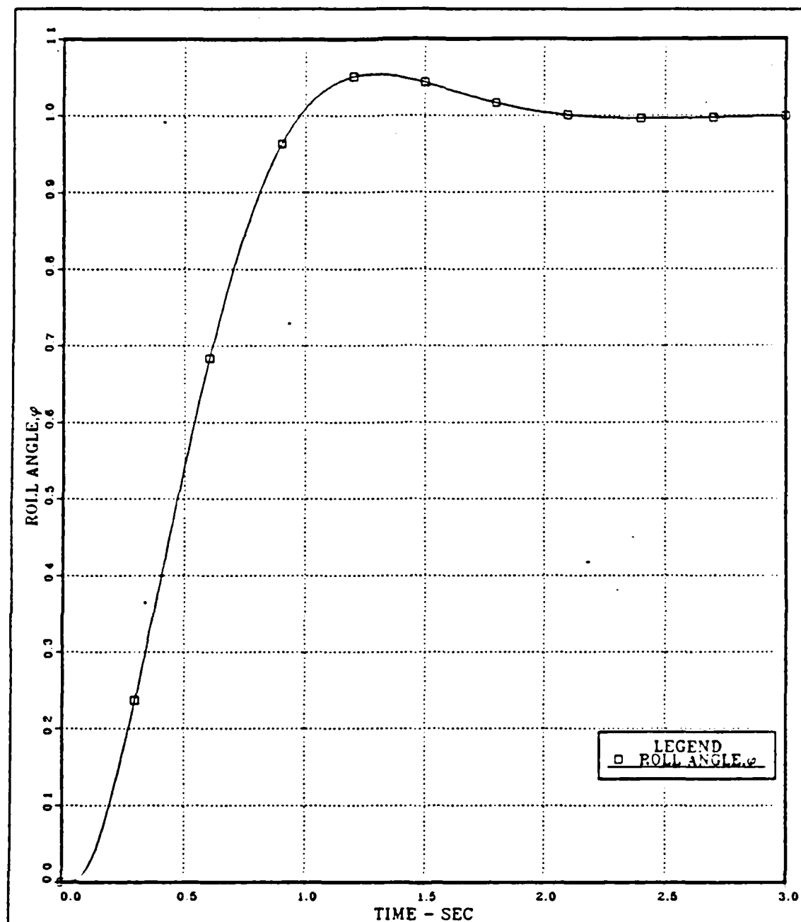
Figure 4.10 Roll Angle vs. Time; Uncoupled Roll Channel; Continuous Open Loop System; Circular Airframe; Step Input \phi_c = 1 rad; a_n = 0 .
