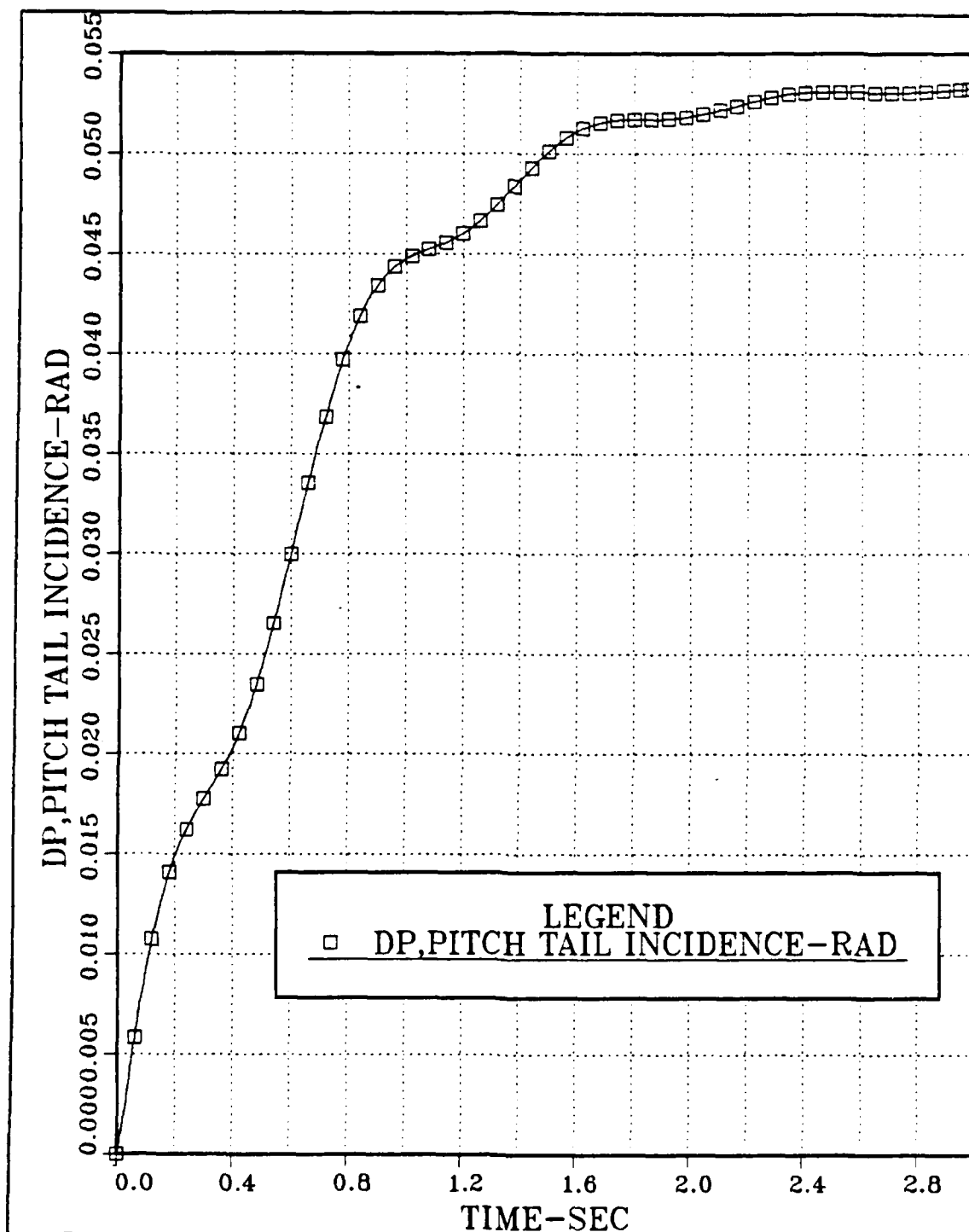
Figure 3.32 Pitch Tail Incidence vs Time; Inoperative \delta_1 , \delta_2 and \delta_3 Control Surfaces; a_0=0 ; Step input: n_{zc} = 1 gee, \delta_{1c} = 0.2 , \delta_{2c} , \delta_{3c} , \delta_{4c} = 0 rad.
