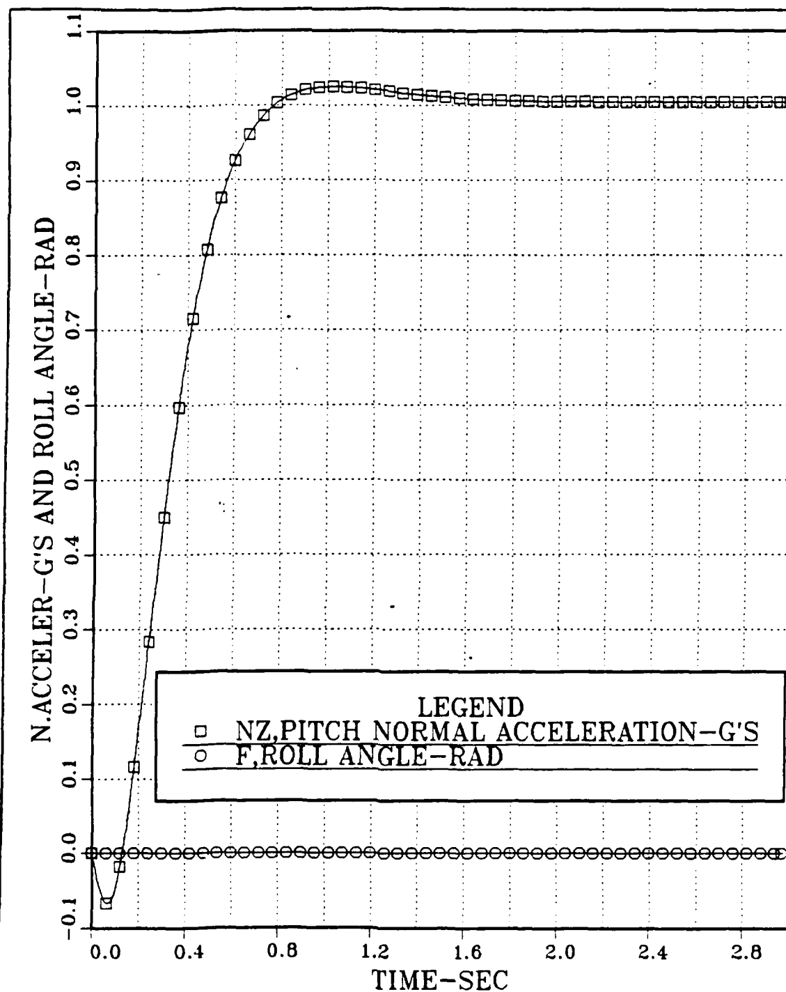
Figure 5.5 Normal Acceleration and Roll Angle vs. Time; Combined Pitch and Roll Channels; Continuous Open Loop System; Step Inputs: \delta_{1c} \delta_{2c} \delta_{3c} \delta_{4c} = 0 and N_{2c} = 1 gee, \psi_c = 0 rad; a_g = 0 .
