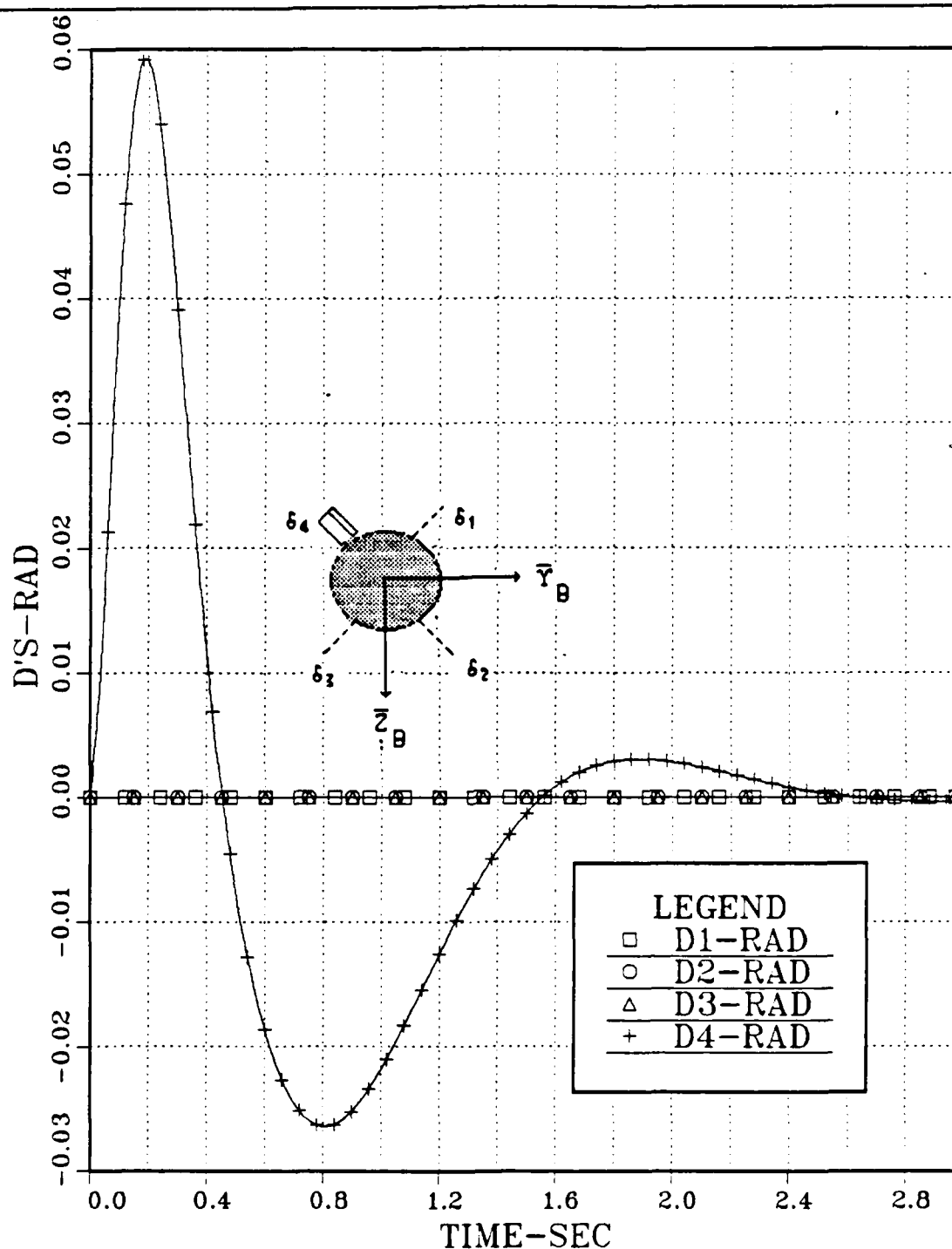
Figure 4.31 Control Surfaces deflections vs. Time; Uncoupled Modified Roll Channel : \delta_1, \delta_2, \delta_3 Centered; Continuous OpenLoop System; Step Input: \psi_C = 1 rad and \delta_1, \delta_2, \delta_3, \delta_4 = 0 ; a_B = 0 .
