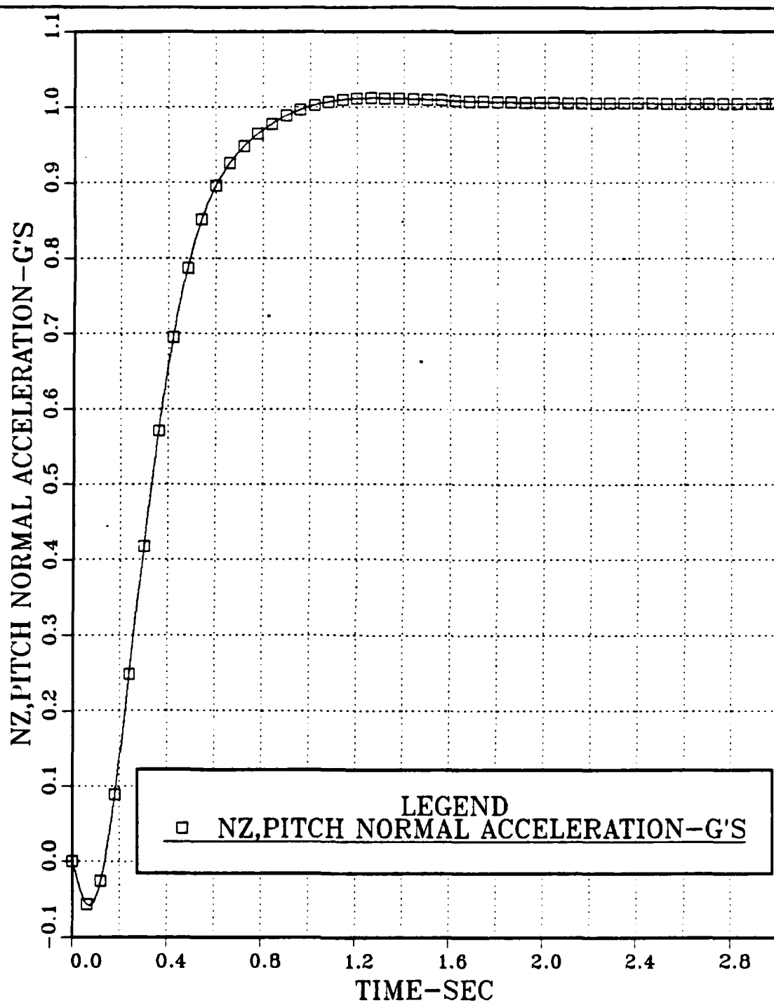
Figure 3.22 Pitch Normal Acceleration vs. Time; Inoperative \delta_1 Control Surface; a_e=0 ; Step input: n_{zc}=1 gee, \delta_{1c}=0.2 , \delta_{2c} \delta_{3c} \delta_{4c}=0 rad.
