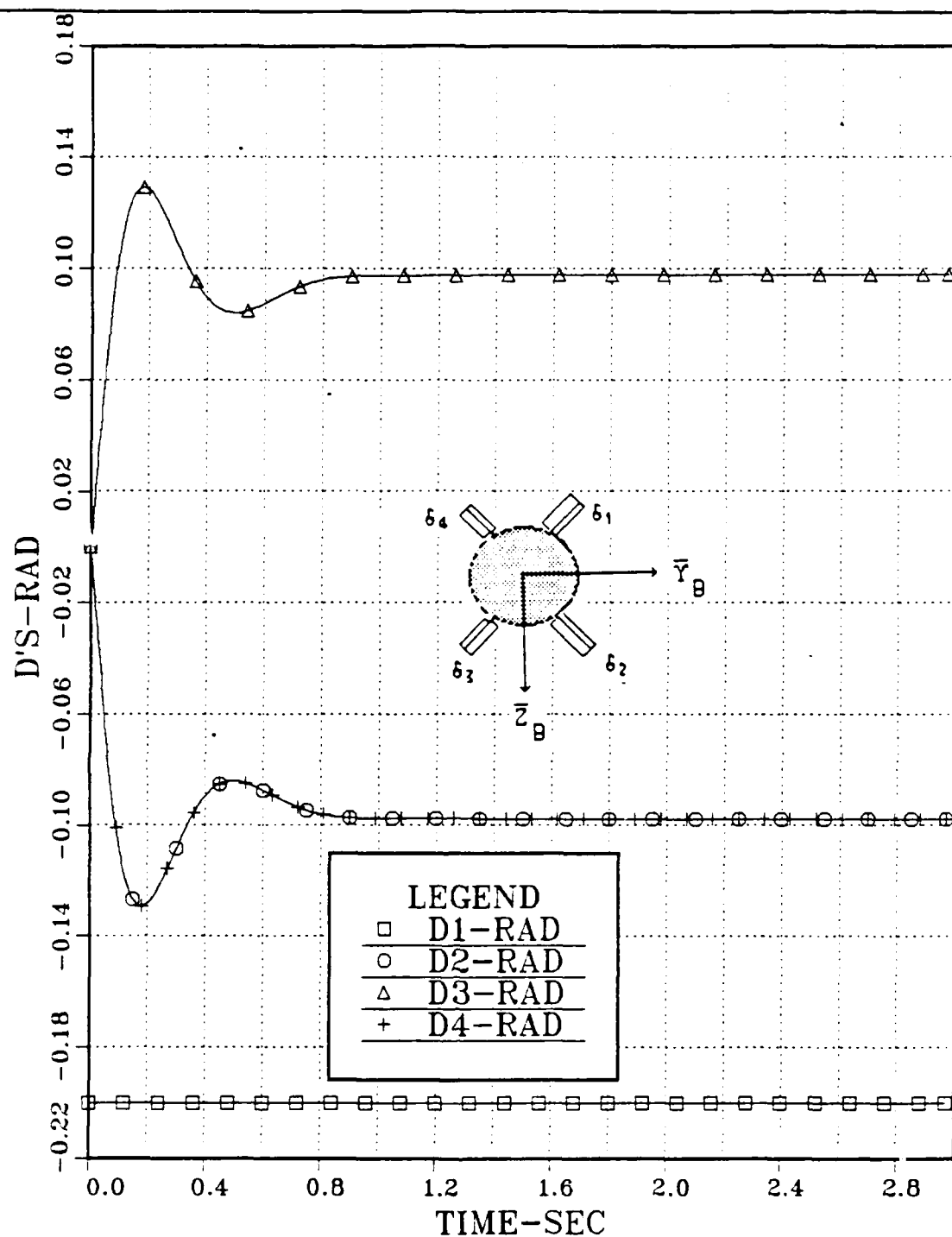
Figure 3.21 Control Surfaces Deflections vs. Time; Hard Over \delta_1 Control Surface; a_0=0 ; Step Input: n_{zc}=1 gee, \delta_{1c}=-0.2 rad, \delta_2, \delta_3, \delta_4=0 .
