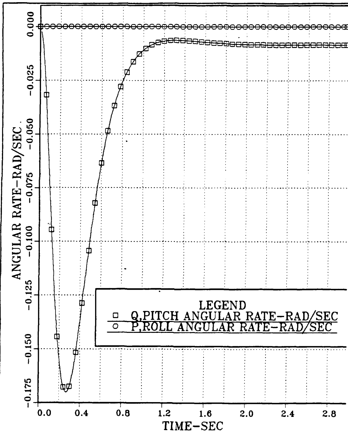
Figure 5.6 Pitch and Roll Angular Rate vs. Time; Combined Pitch and Roll Channels; Continuous Open Loop System; Step Inputs: \delta_{1c} \delta_{2c} \delta_{3c} \delta_{4c} = 0 and N_{zc} = 1 \text{ gee} , \psi_c = 0 \text{ rad} ; a_\theta = 0 .
