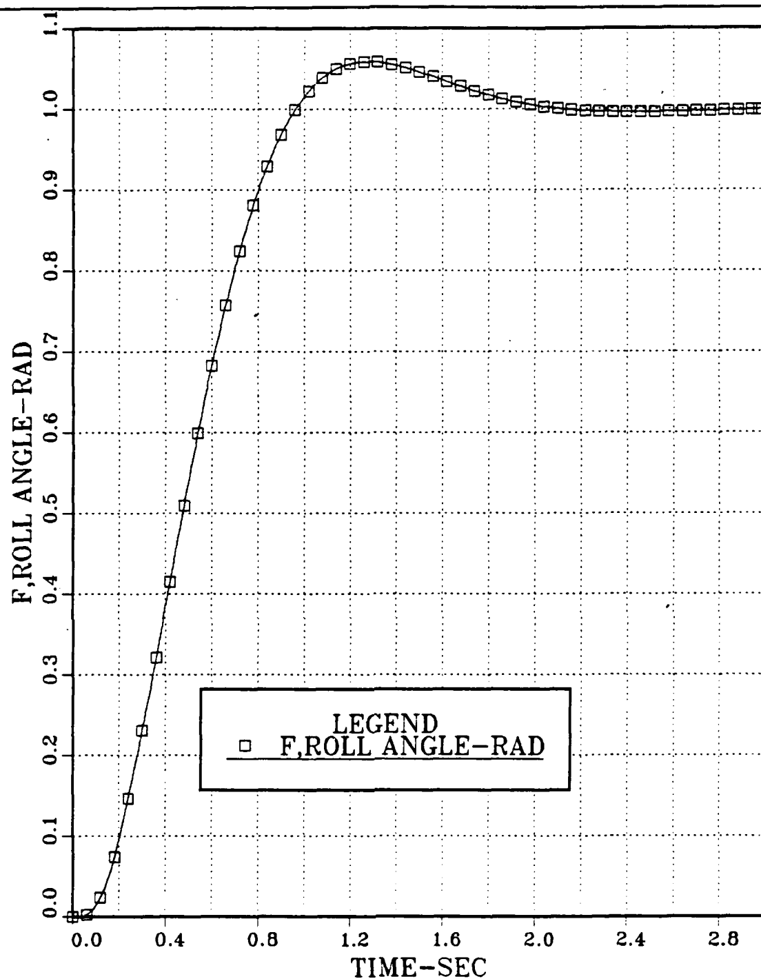
Figure 4.20 Roll Angle vs. Time; Uncoupled Modified Roll Channel with \delta_1 Centered; Continuous Open Loop System; Step Input: \psi_C = 1 rad and \delta_{1C} \delta_{2C} \delta_{3C} \delta_{4C} = 0 ; a_0 = 0 .
