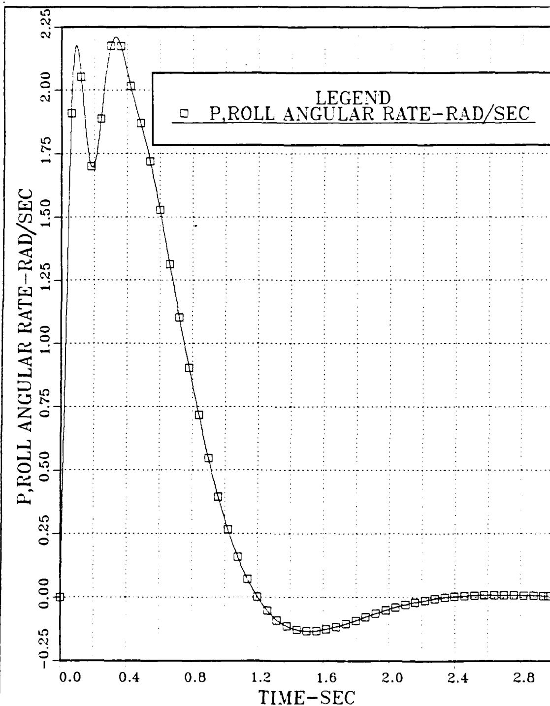
Figure 4.17 Roll Angular Rate vs. Time; Uncoupled Modified Roll Channel with \delta_1 Hard Over; Continuous Open Loop System; Step Inputs: \delta_1=0.2 rad; \delta_2, \delta_3, \delta_4=0 ; \psi_c=1 rad and a_g=0 .
