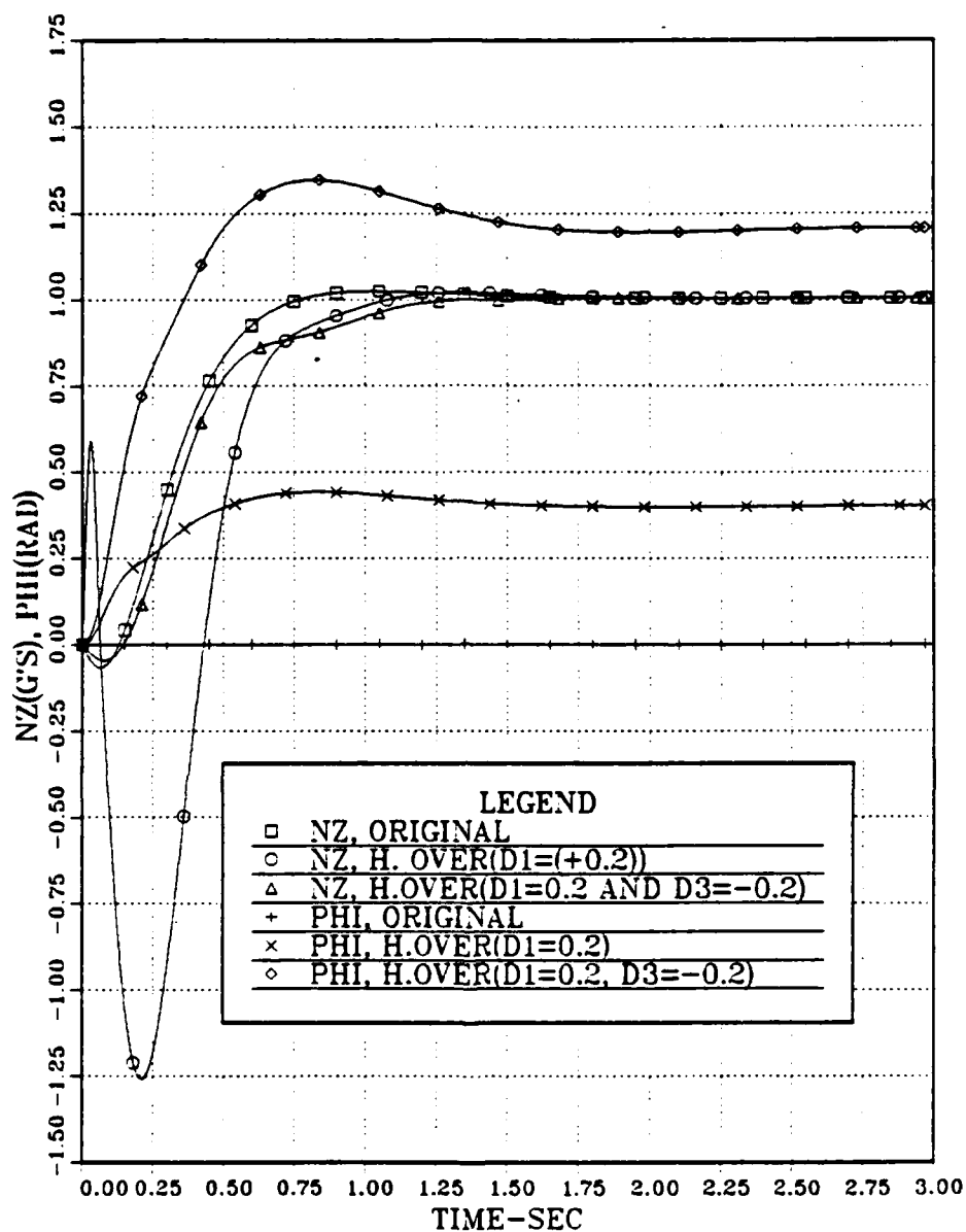
Figure 5.18 Second Corrective Action and Comparison of the Pitch Normal Acceleration (NZ) and the Roll Angle ( \phi ), between Three Different Effectors Configuration.
