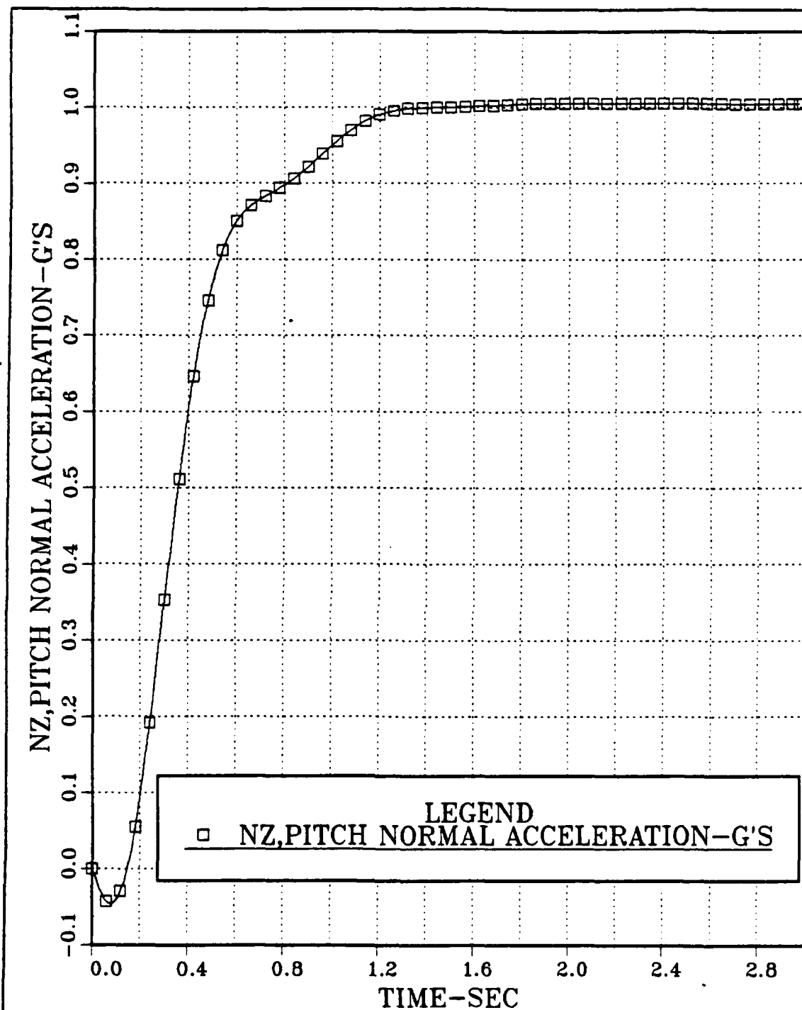
Figure 3.26 Pitch Normal Acceleration vs. Time; Inoperative \delta_1 and \delta_2 Control Surfaces; a_g=0 ; Step input: n_{zc} = 1 gee, \delta_{1c} = 0.2 , \delta_{2c} , \delta_{3c} , \delta_{4c} = 0 rad.
