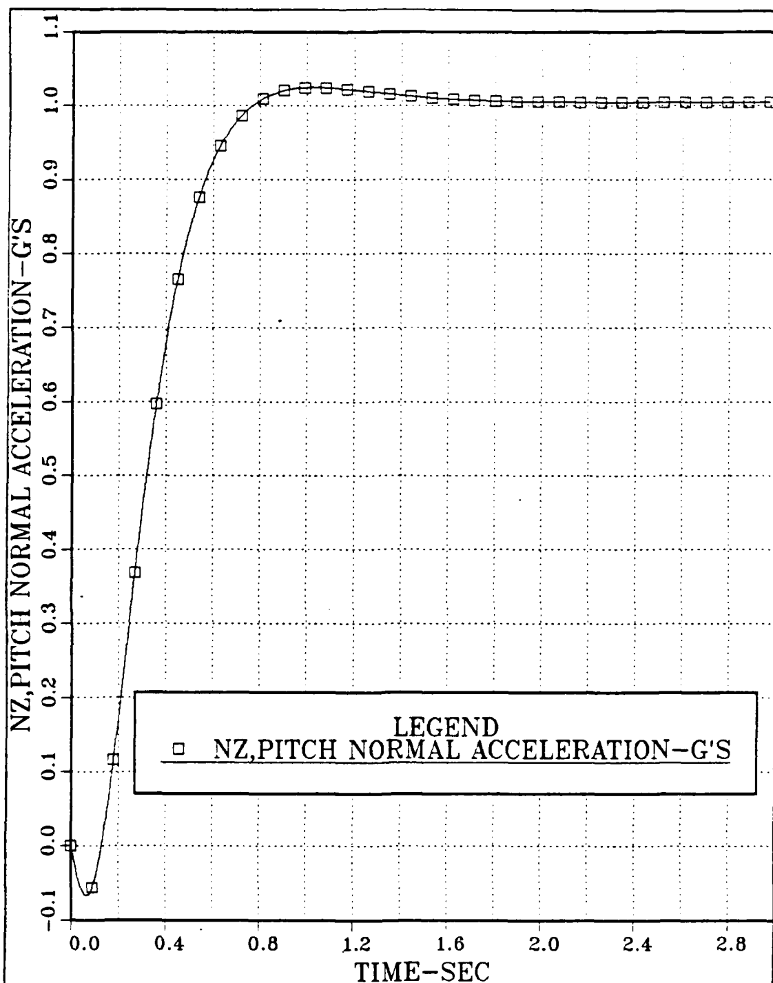
Figure 3.10 Pitch Normal Acceleration vs. Time; Uncoupled Pitch Channel; Unimpaired Open Loop System; a_e=0 ; Step Input: n_{zo}=1 g's and \delta_{1c} \delta_{2c} \delta_{3c} \delta_{4c} = 0 degrees.
