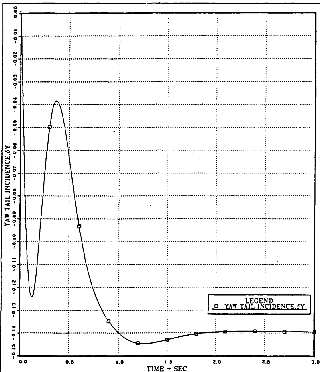
Figure 4.6 Yaw Tail Incidence vs. Time; Uncoupled Yaw Channel Autopilot; Continuous Open Loop System; Elliptical Airframe; Step Input H_Y = 1 gee; a_n = 0 .
