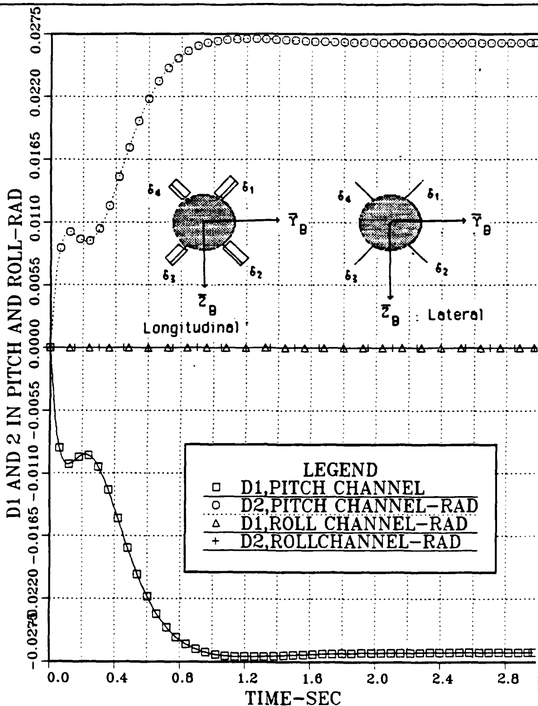
Figure 5.8 Pitch and Roll Deflections vs. Time; Combined Pitch and Roll Channels; Continuous Open Loop System; Step Inputs: \delta_{1c} \delta_{2c} \delta_{3c} \delta_{4c} = 0 and N_{2c} = 1 gee, \psi_c = 0 rad; a_g = 0 .
