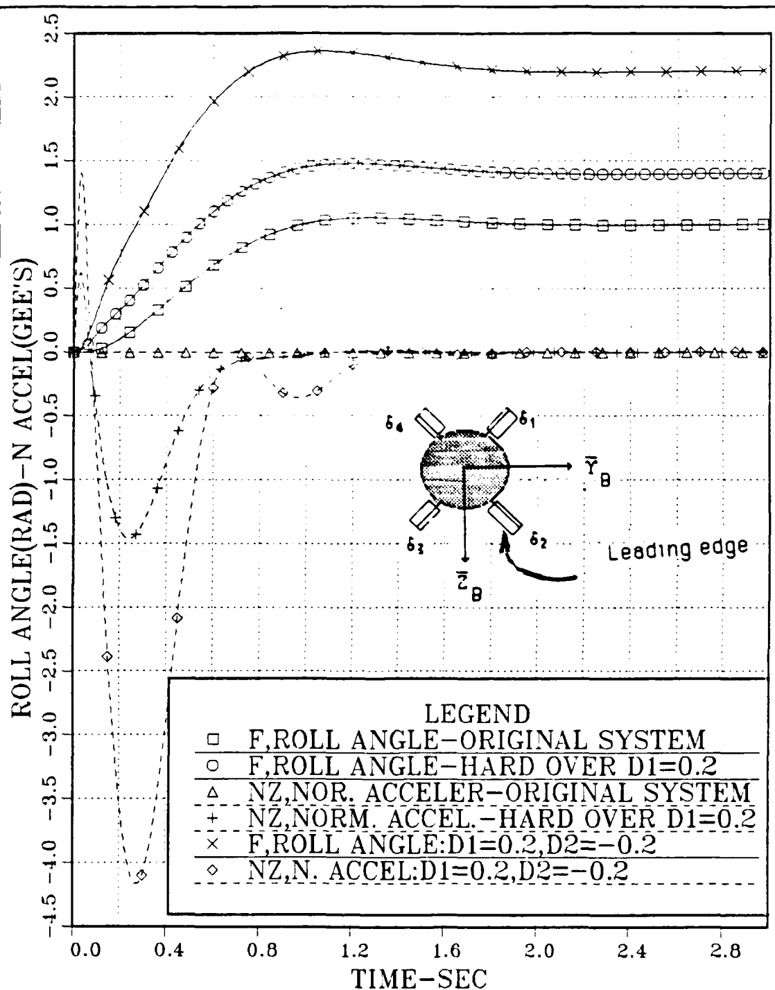
Figure 5.24 First Corrective Action and Comparison of the Pitch Normal Acceleration ( N_z ) and the Roll Angle ( \phi ), between Three Different Effectors Configuration.
