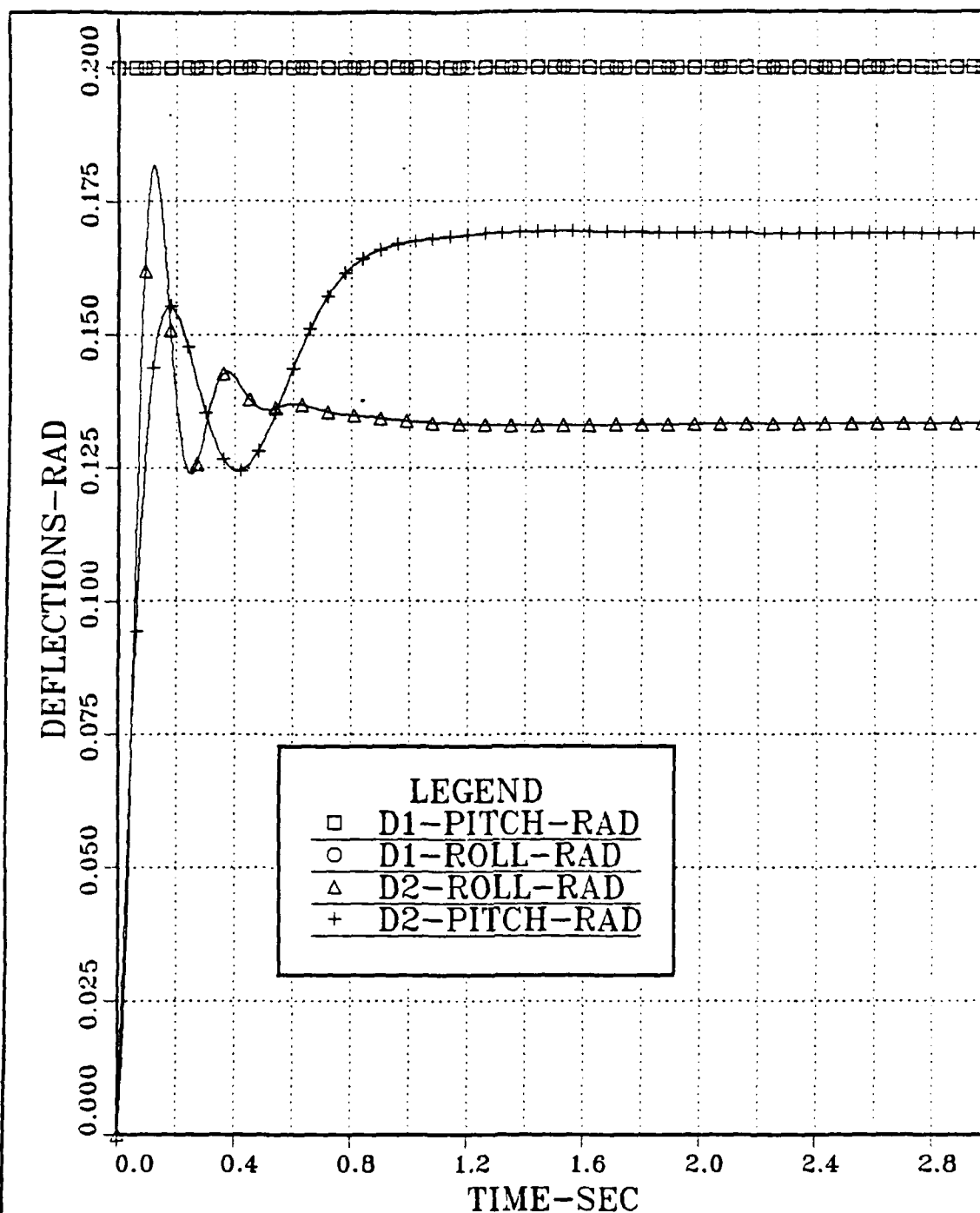
Figure 5.16 Hard Over \delta_1 Type of Impairment: Pitch and Roll Deflections vs. Time; Combined Pitch and Roll Channels; Continuous Open Loop System; Step Inputs: \delta_{1c}=0.2\text{rad} , \delta_{2c} , \delta_{3c} , \delta_{4c} = 0 and N_{zc} = 1 \text{ gee} , \psi_c = 0 \text{ rad} ; a_e = 0 .
