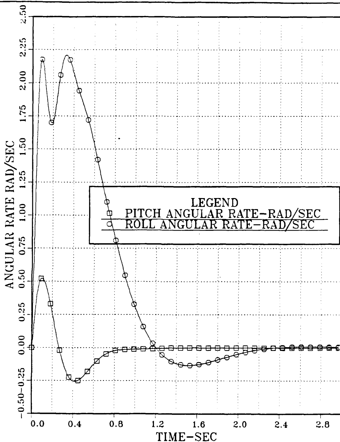
Figure 5.21 Hard Over \delta_1 Type of Impairment: Pitch and Roll Angular Rate vs. Time; Combined Pitch and Roll Channels; Continuous Open Loop System; Step Inputs: \delta_{1c}=0.2\text{rad} , \delta_{2c} , \delta_{3c} , \delta_{4c} = 0 and N_{zc} = 0 gee, \psi_c = 1 rad; a_p = 0 .
