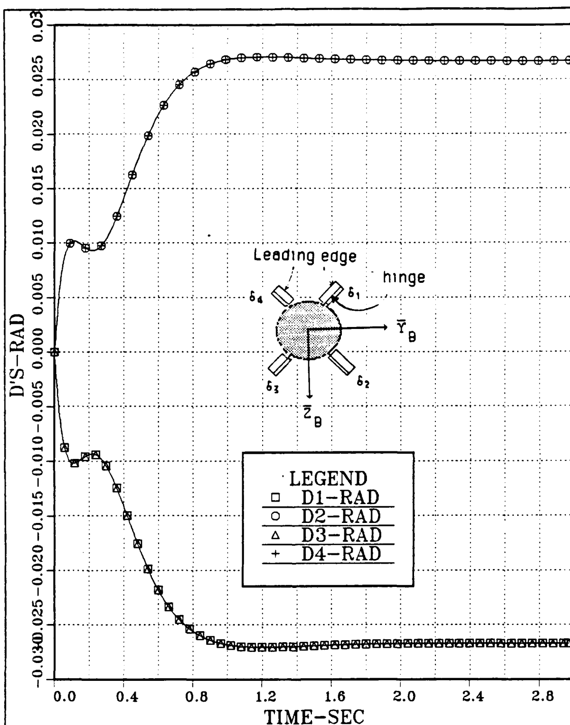
Figure 3.13 Control Surfaces Deflections vs. Time; Uncoupled Pitch Channel; Unimpaired Open Loop System; a_p=0 ; Step Input: n_{zc}=1 g's and \delta_{1c} \delta_{2c} \delta_{3c} \delta_{4c} = 0 degrees.
