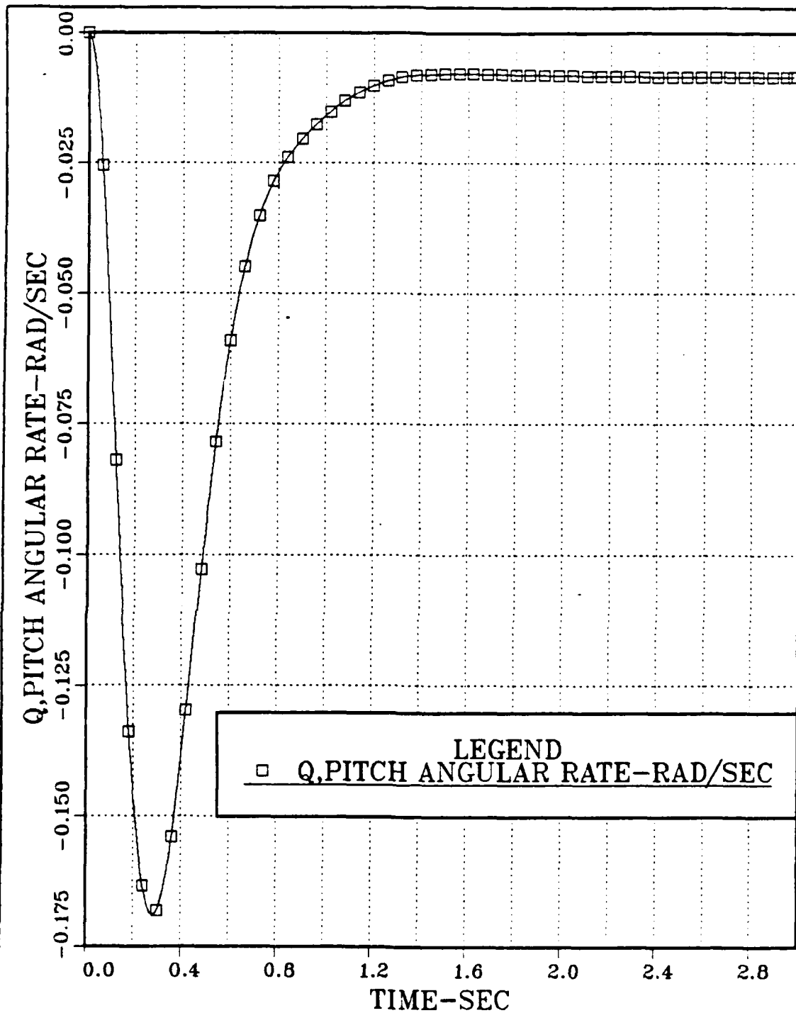
Figure 3.23 Pitch Angular Rate vs Time; Inoperative \delta_1 Control Surface; \delta_2=0 ; Step input: n_{zc} = 1 gee, \delta_{1c} = 0.2 , \delta_{2c} , \delta_{3c} , \delta_{4c} = 0 rad.
