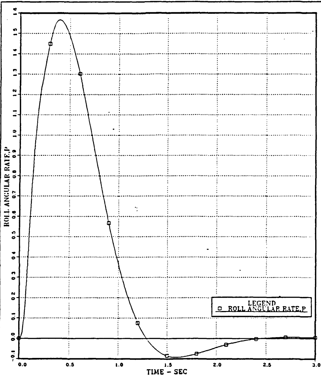
Figure 4.9 Roll Angular Rate vs. Time; Uncoupled Roll Channel; Continuous Open Loop System; Circular Airframe; Step Input \psi_c = 1 rad; a_n = 0 .
