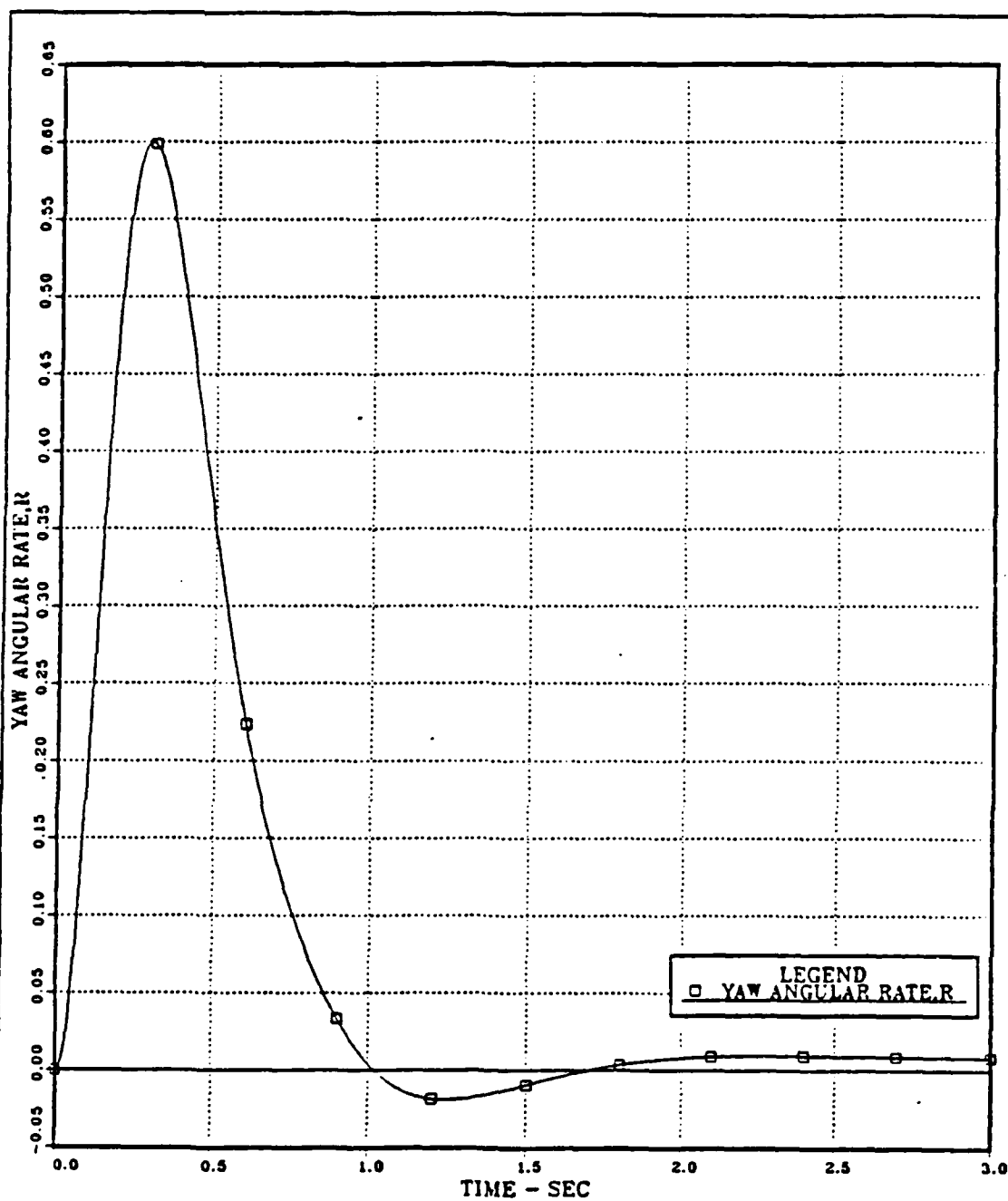
Figure 4.5 Yaw Angular Rate vs. Time; Uncoupled Yaw Channel Autopilot; Continuous Open Loop System; Elliptical Airframe; Step Input H_Y = 1 gee; a_0 = 0 .
