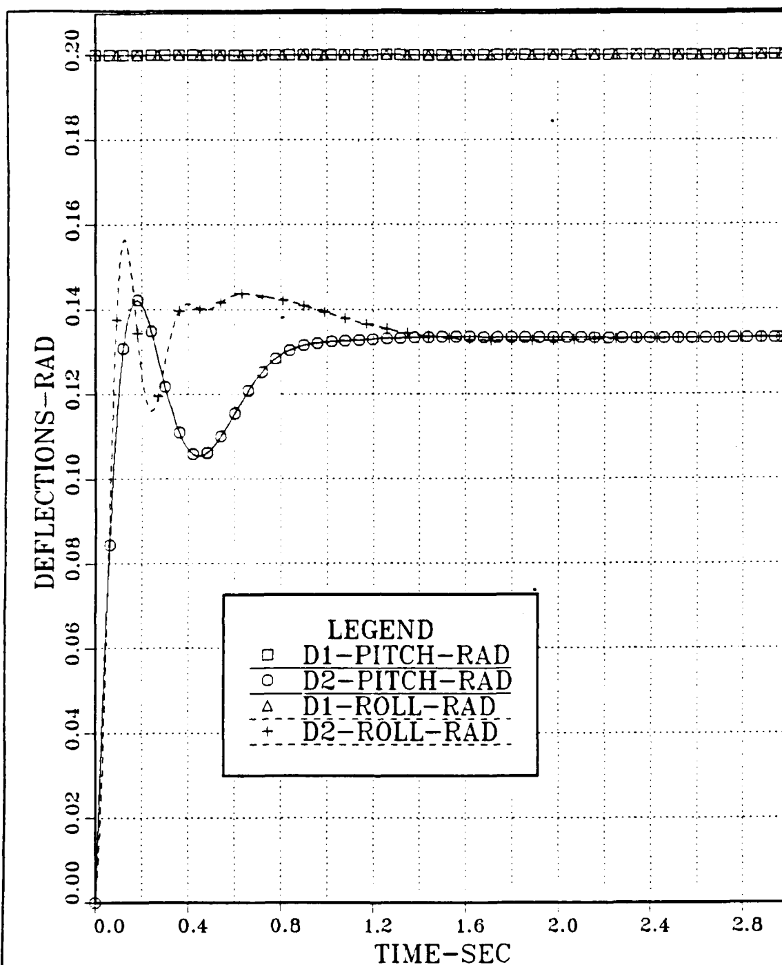
Figure 5.23 Hard Over \delta_1 Type of Impairment: Pitch and Roll Deflections vs. Time; Combined Pitch and Roll Channels; Continuous Open Loop System; Step Inputs: \delta_{1c}=0.2\text{rad} , \delta_{2c} , \delta_{3c} , \delta_{4c} = 0 and N_{2c} = 0 gee, \psi_c = 1 rad; a_\theta = 0 .
