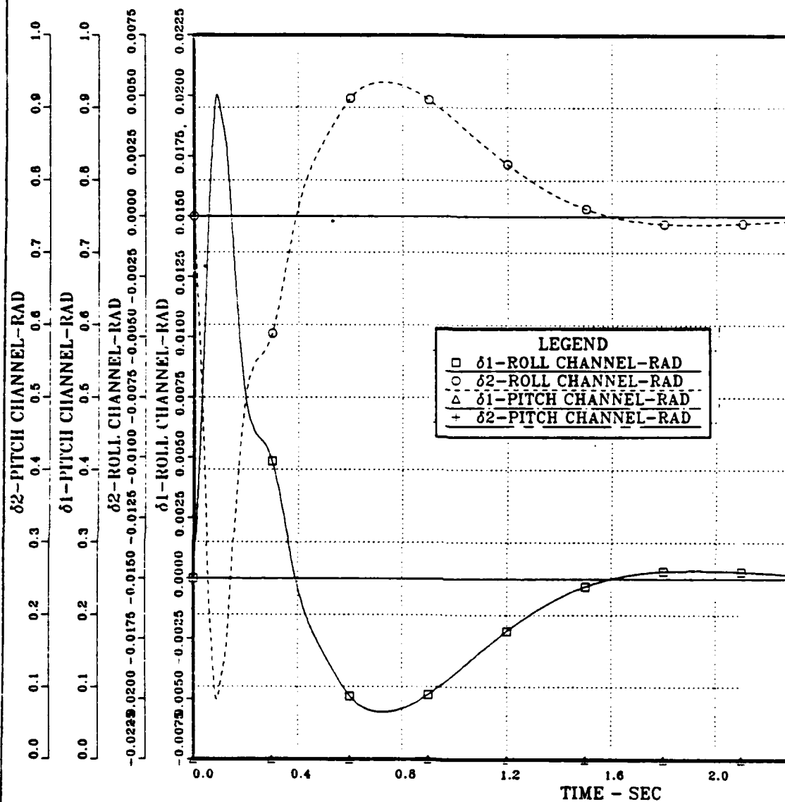
Figure 5.12 Pitch and Roll Deflections vs. Time; Combined Pitch and Roll Channels; Continuous Open Loop System; Step Inputs: \delta_{1c} \delta_{2c} \delta_{3c} \delta_{4c} = 0 and N_{2c} = 0 gee, \psi_c = 1 rad; a_g = 0 .
