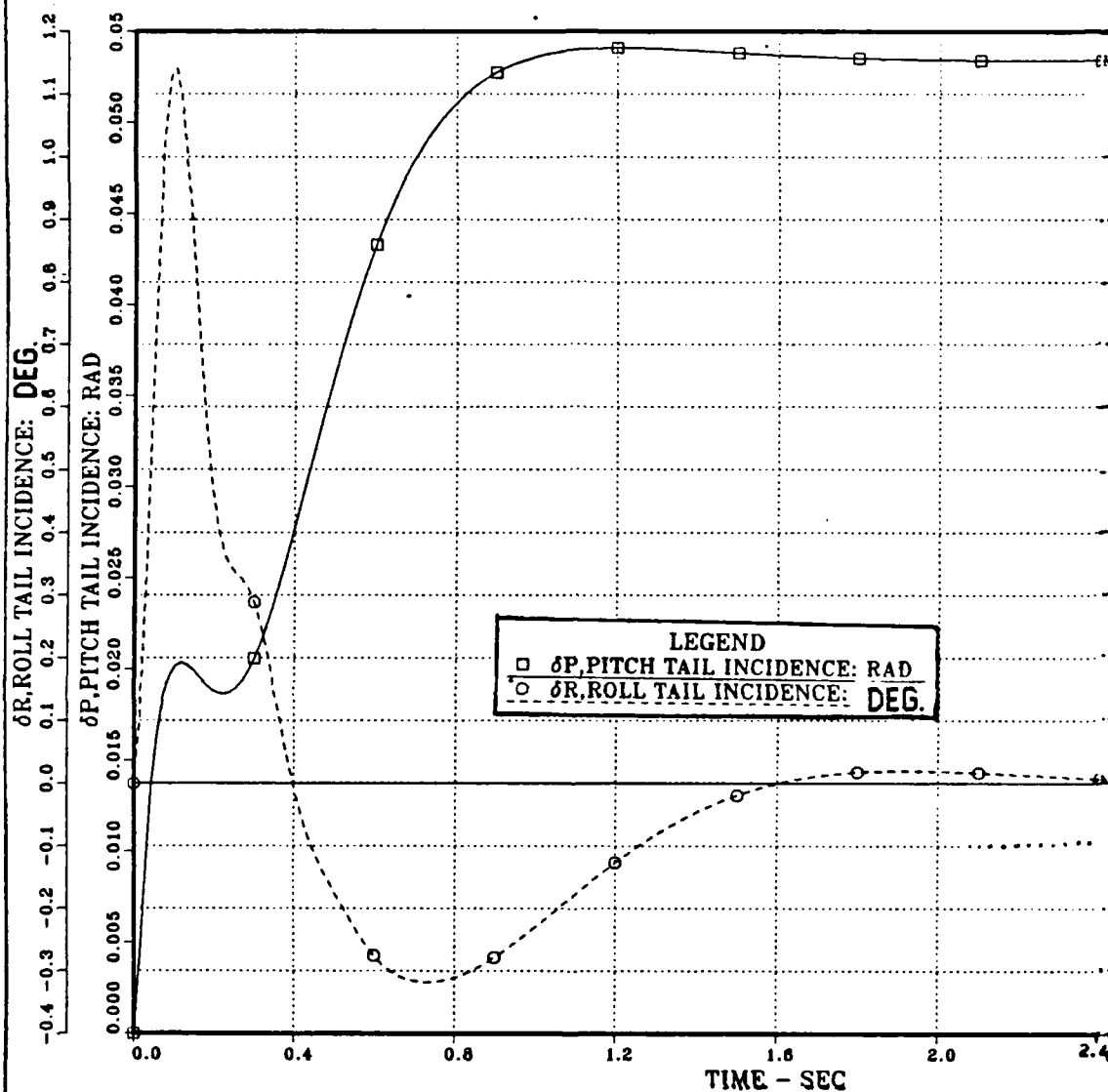
Figure 5.3 Pitch and Roll Tail Incidence vs. Time; Combined Pitch and Roll Channels; Continuous Open Loop System; Step Inputs: \delta_{10} \delta_{20} \delta_{30} \delta_{40} = 0 and N_{2c} = 1 \text{ gee} , \psi_c = 1 \text{ rad} ; a_g = 0 .
