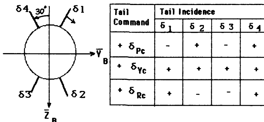
Figure 2.2 B.T.T Aerodynamic Sign Convention.
