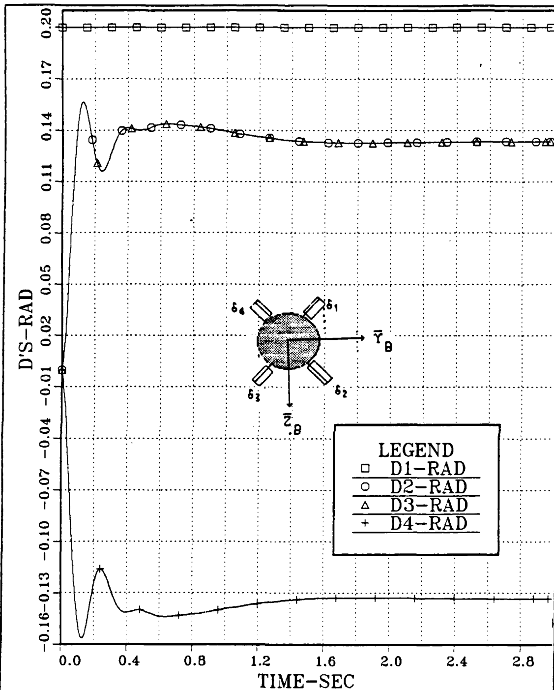
Figure 4.19 Control Surfaces deflections vs.time; Uncoupled Modified Roll Channel with \delta_1 Hard Over ; Continuous Open Loop System; Step Inputs: \delta_1=0.2 rad; \delta_2, \delta_3, \delta_4=0 ; \psi_C=1 rad and a_\theta = 0 .
