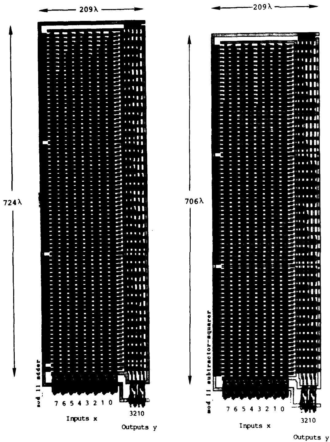
Figure 4.14. PLAs for Mod 11 Subtractor-Squarer and Adder
