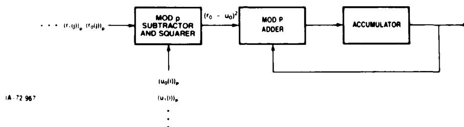
Figure 4.13. Local Distortion Computation Mod P
