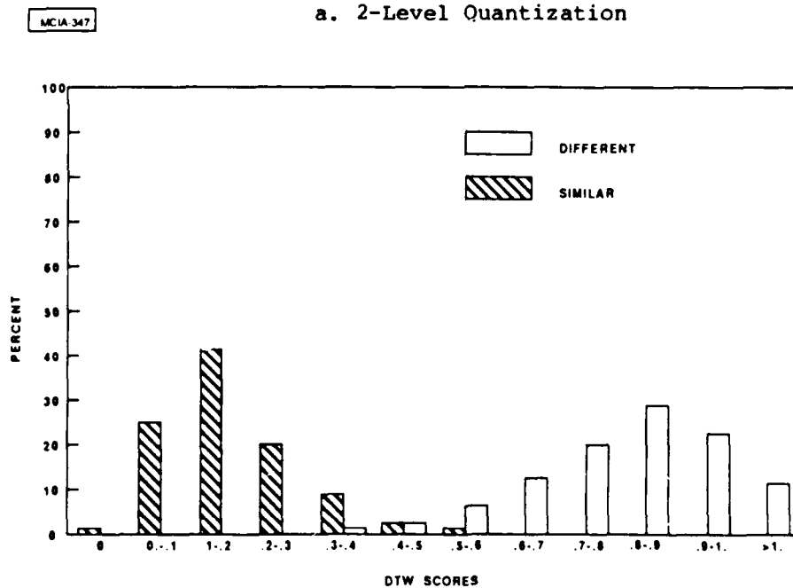
Figure 3.33b. HISTOGRAM OF DTW SCORES WITH PRE-EMPHASIS: \mu = .95
