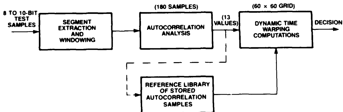
Figure 1.1. RNS-Based Word Recognition
