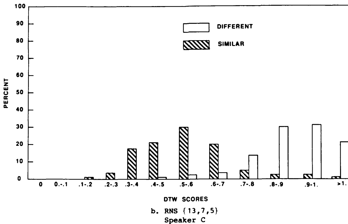
Figure 3.29. DTW Scores with Pre-Emphasis: \mu = .95 , Global = 18
