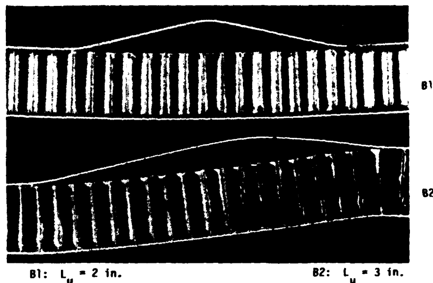
B. CLOSE-UP VIEW OF UNBONDED REGION (OPPOSITE SIDE OF BEAM)
