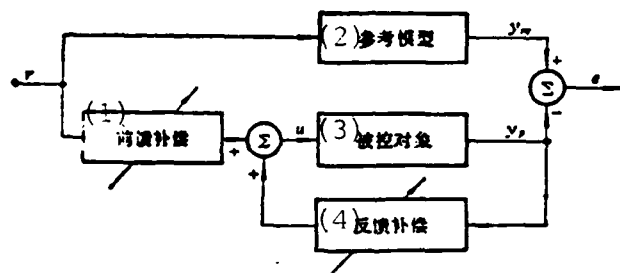
Fig. 2. Model reference adaptive control system
