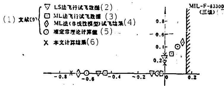
Fig. 3. Comparison of characteristic root results. Key: (1) Reference [9]; (2) flight-test data of LS method; (3) flight-test data of ML method; (4) flight-test data of ML method (nonlinear model); (5) quasi-steady theory computed values; (6) computed results of this paper; (7) third class.
