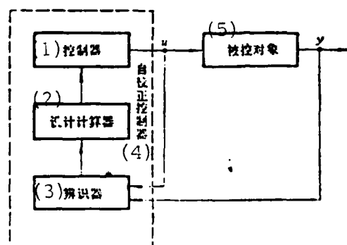
Fig. 3. Self tuning regulator
