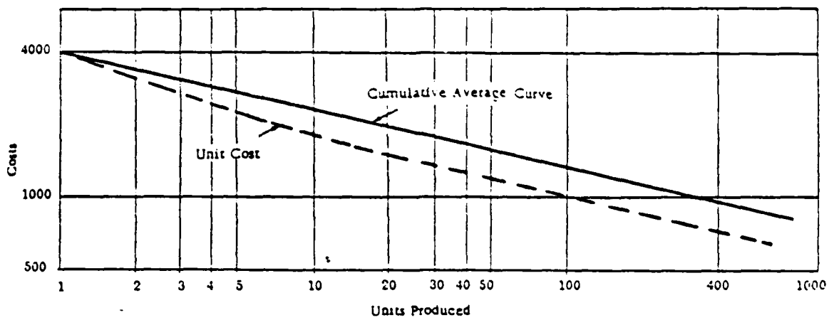
Figure 7.1 LOG-LINEAR CUMULATIVE AVERAGE CURVE.
