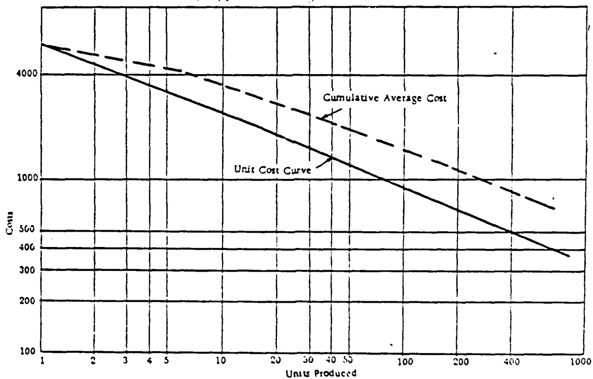
Figure 7.2 LOG-LINEAR UNIT COST CURVE.
