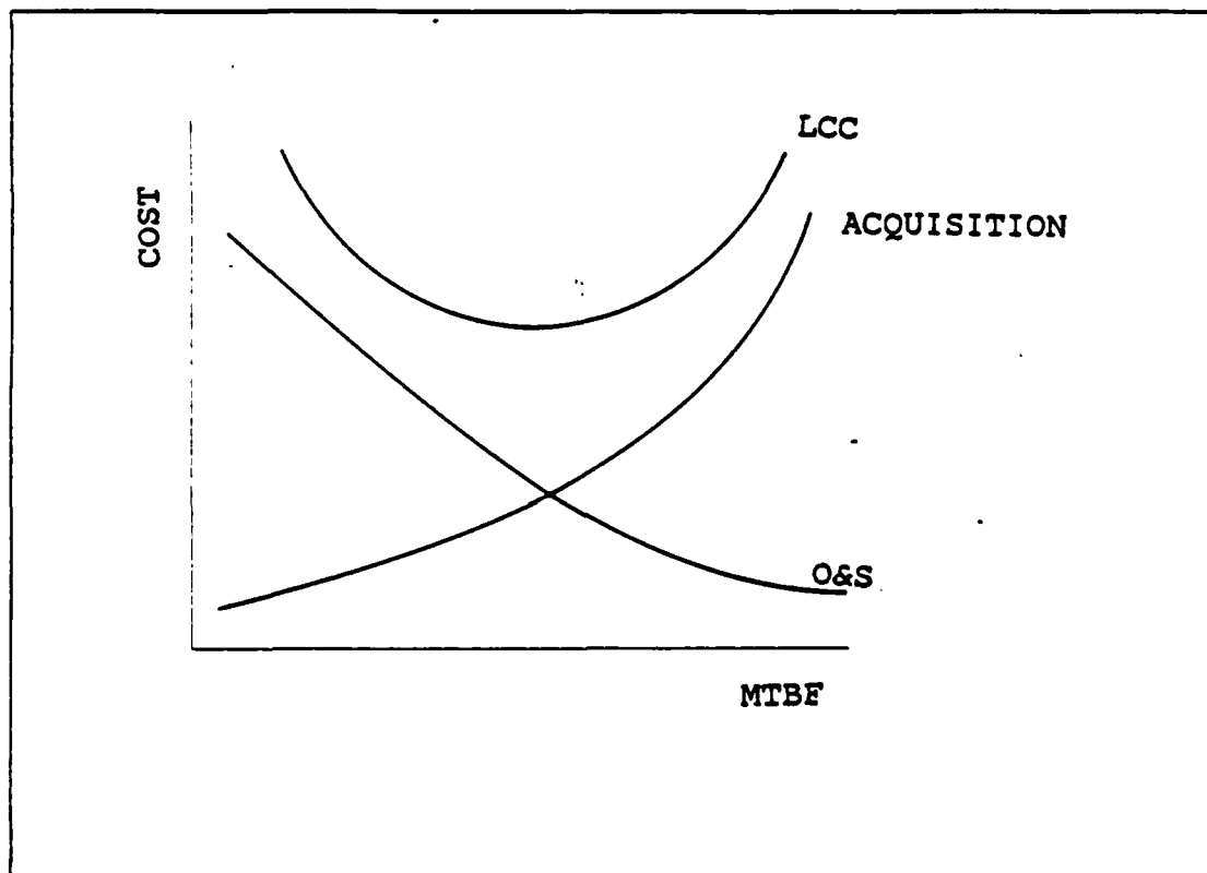
Figure 4.1 LCC / RELIABILITY RELATIONSHIP.
