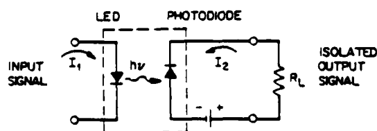
Figure 1. An Opto-isolator Circuit [Ref.3]
