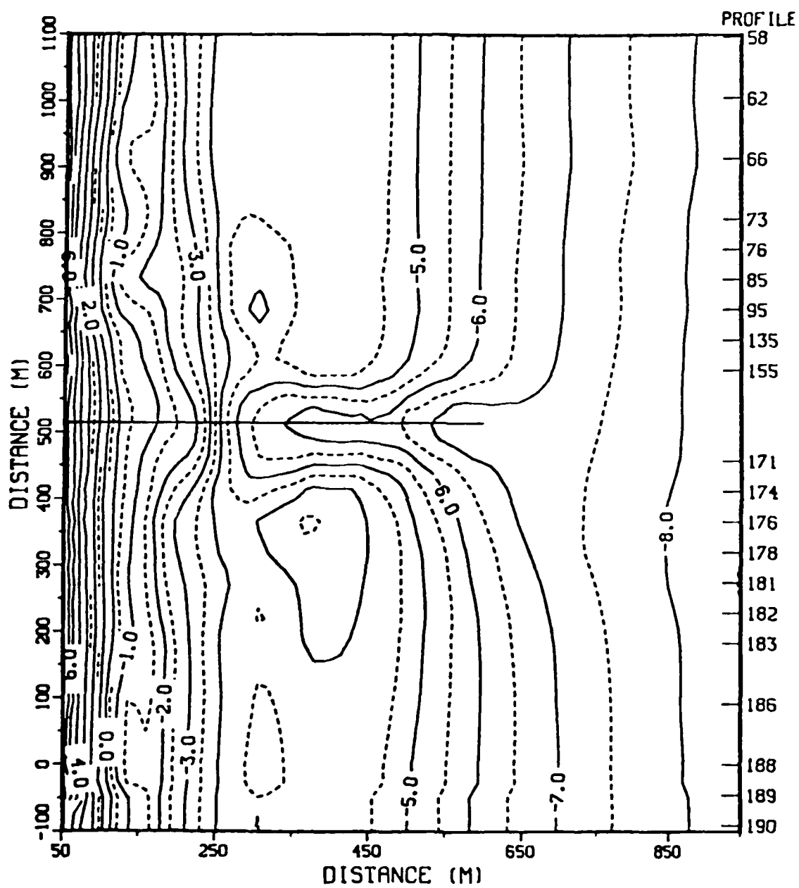
Figure C6. FRF bathymetry, 12 July 1983 (contours in metres)
