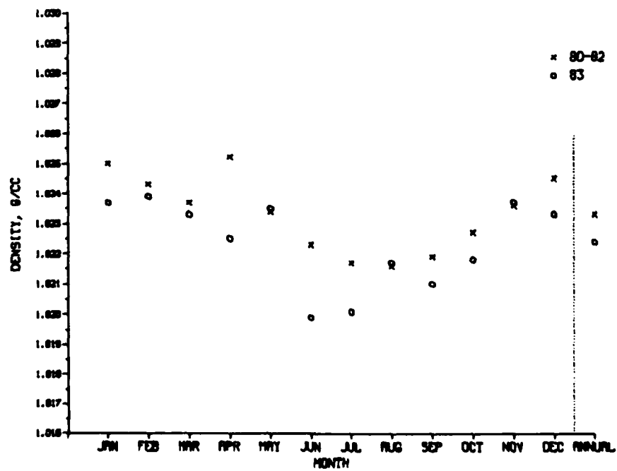
Figure 40. Comparison of mean sea-surface water density
