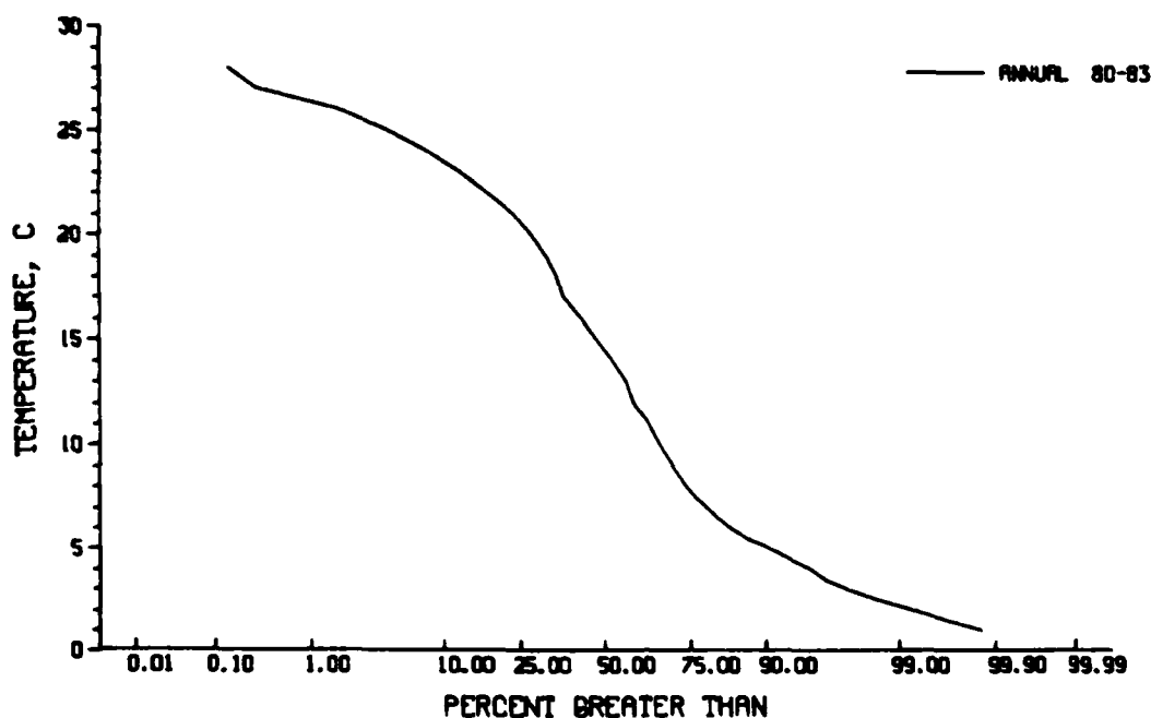
Figure 35. Distribution of surface water temperatures for 1980 through 1983
