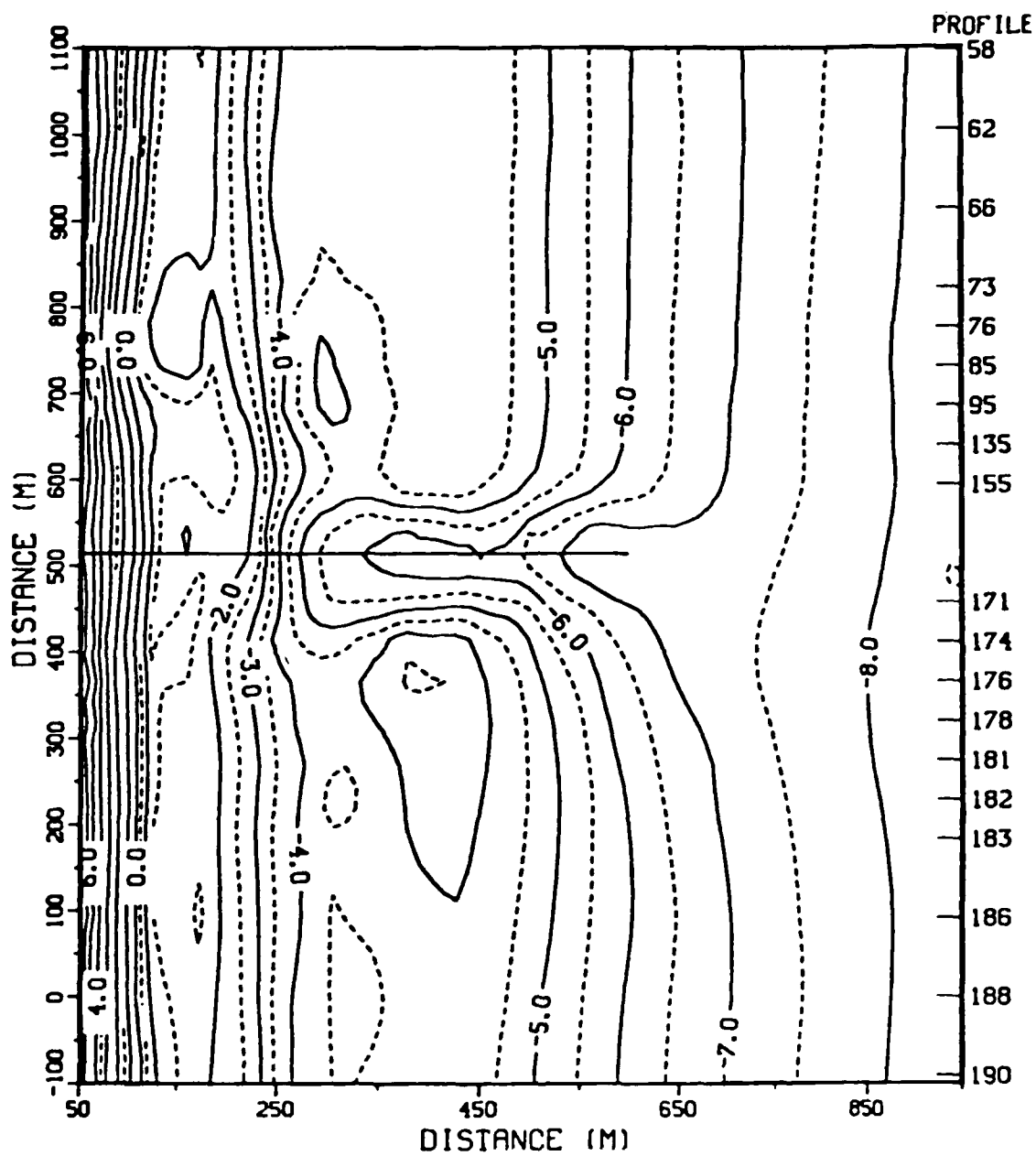
Figure C4. FRF bathymetry, 5 May 1983 (contours in metres)
