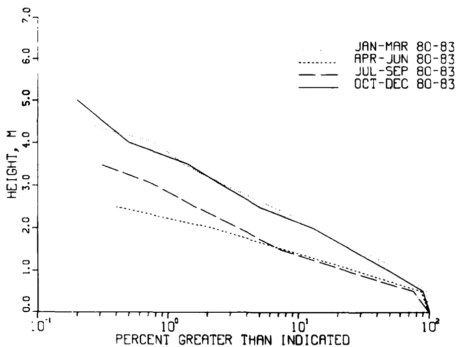
Figure B29. 1980 through 1983 seasonal cumulative distribution of H_{m0} for gage 620
