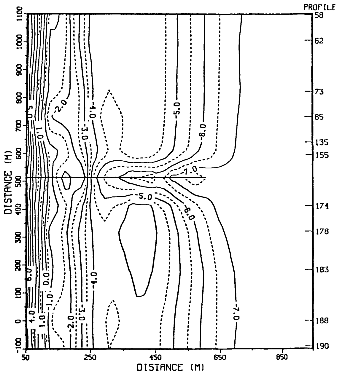
Figure C5. FRF bathymetry, 14 June 1983 (contours in metres)
