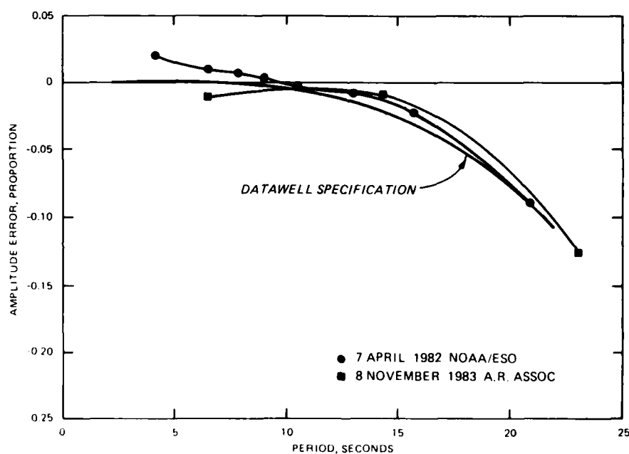
Figure A1. Waverider 66966 predeployment and postdeployment calibrations
