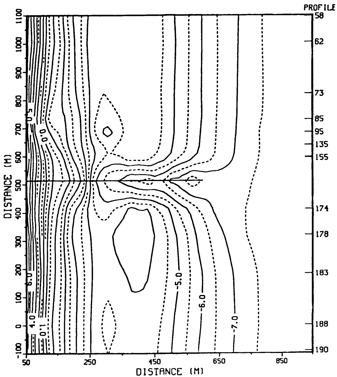
Figure C7. FRF bathymetry, 8 August 1983 (contours in metres)
