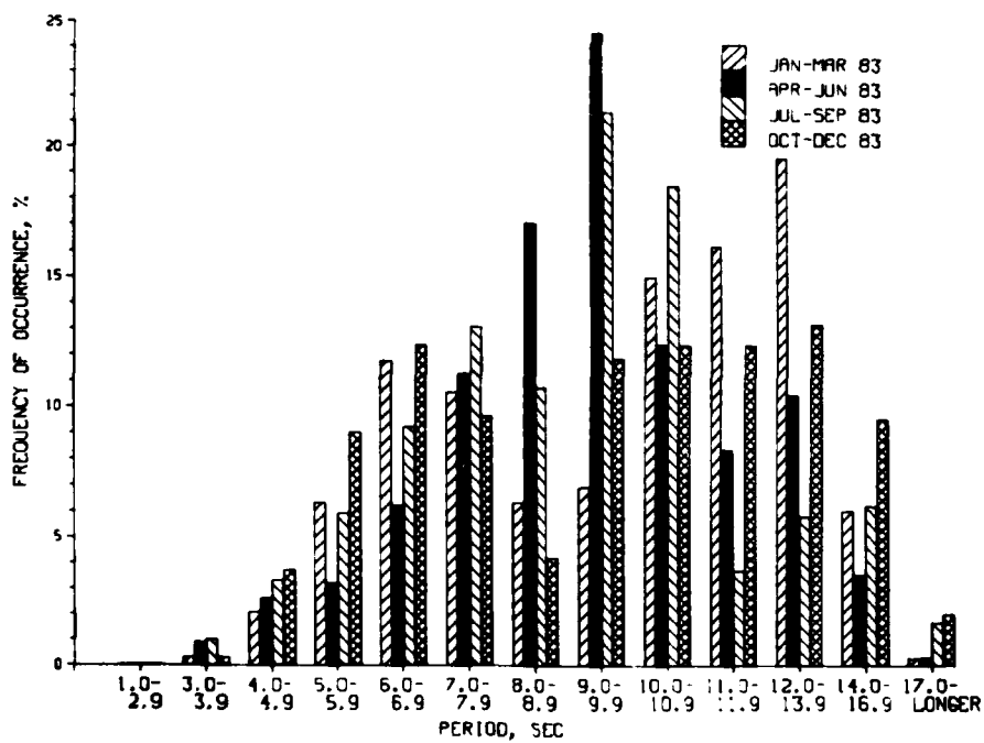
Figure 15. 1983 seasonal wave period distributions for gage 625
