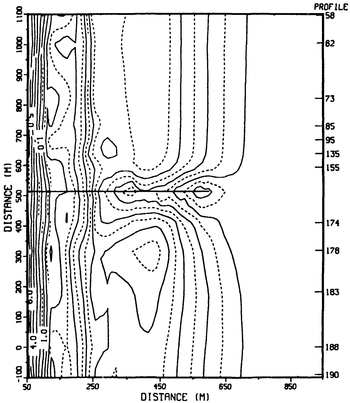
Figure C9. FRF bathymetry, 1 October 1983 (contours in metres)
