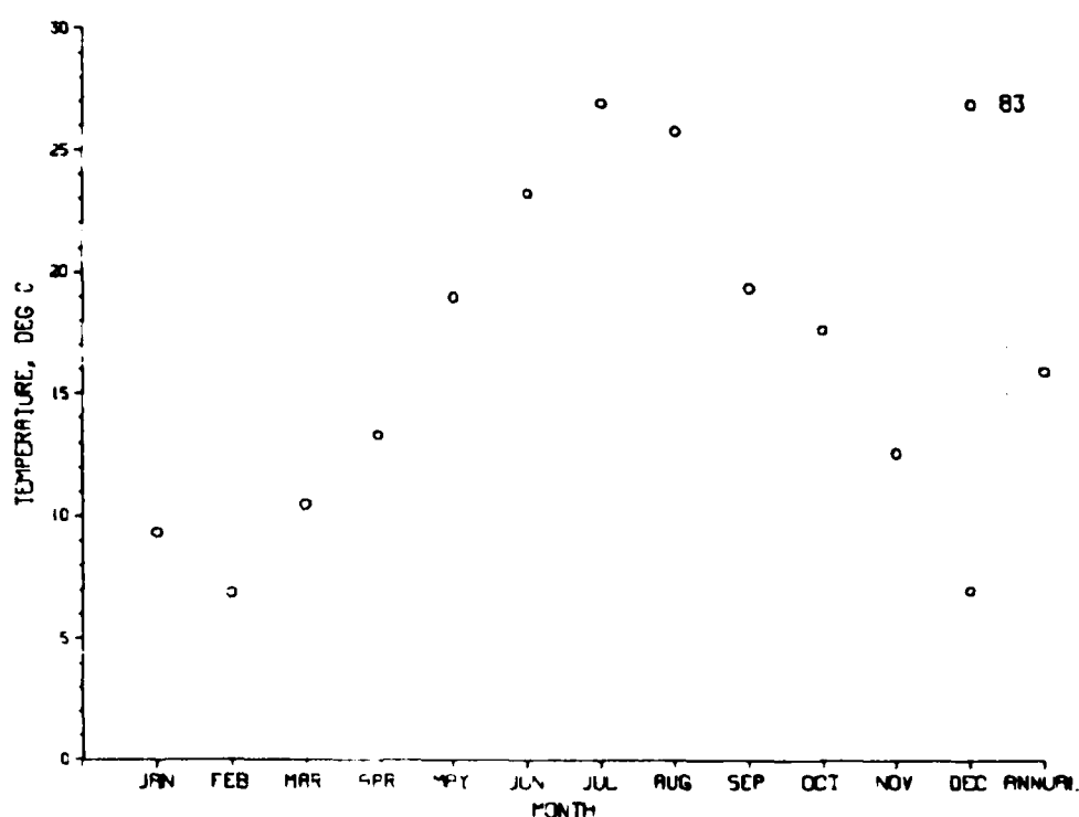
Figure 4. Mean monthly air temperatures, 1983
