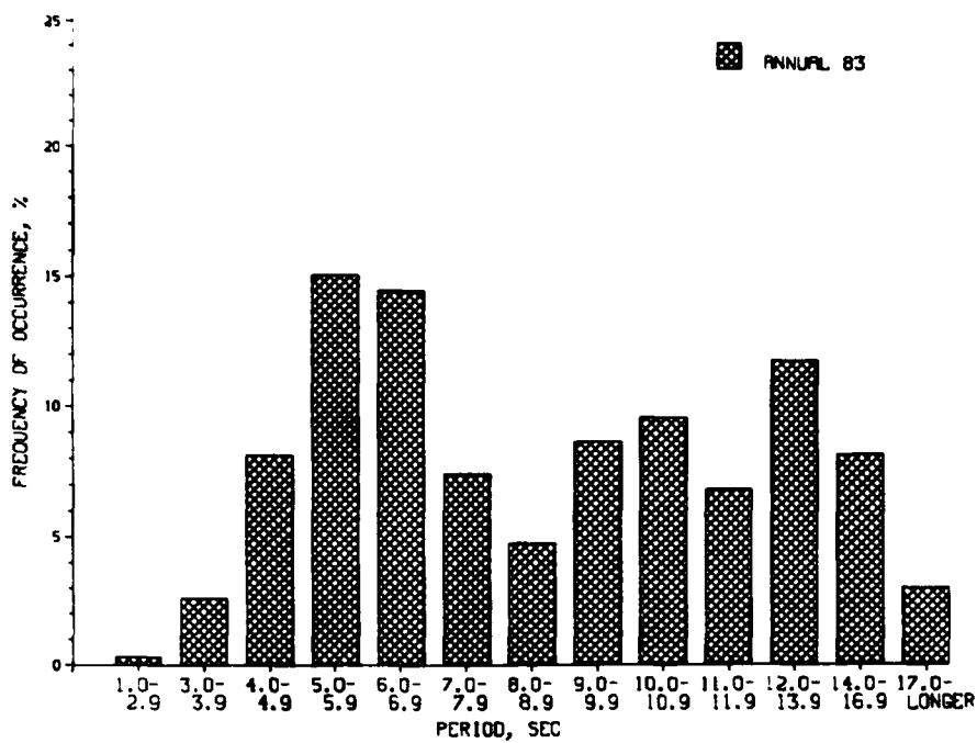
Figure B38. 1983 annual distribution of T_p for gage 615
