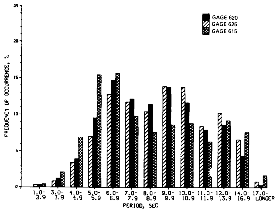
Figure 21. Wave period distributions, 1980 through 1983
