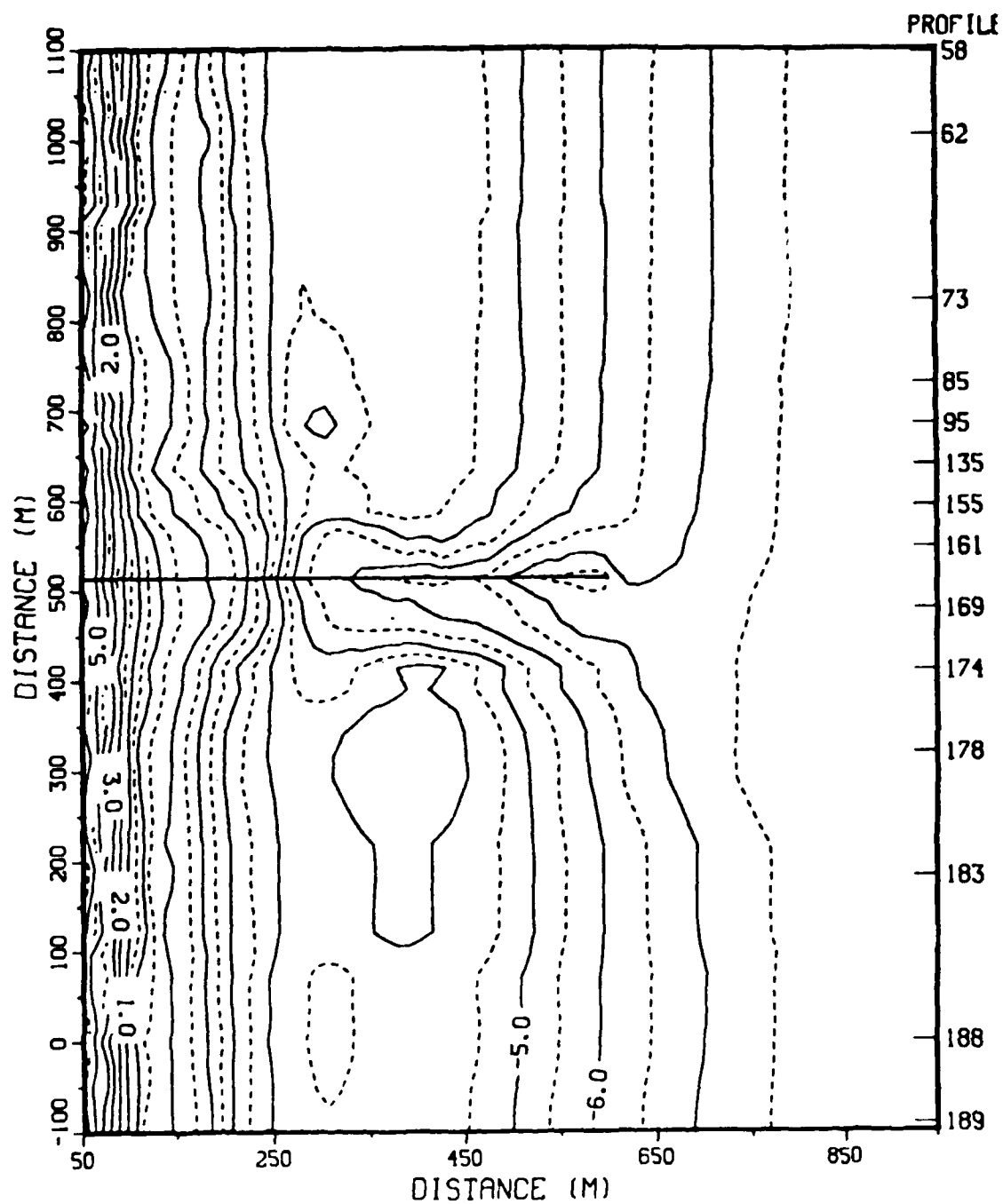
Figure C8. FRF bathymetry, 6 September 1983 (contours in metres)
