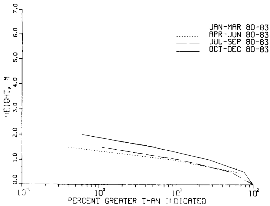
Figure B42. 1980 through 1983 seasonal cumulative distribution of H_{m0} for gage 615
