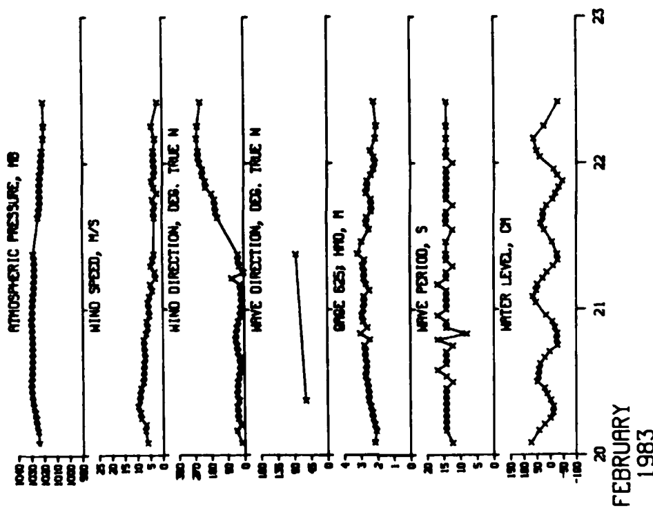
Figure D8. Storm data for 20-22 February 1983
