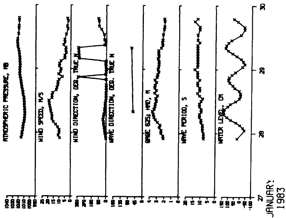
Figure D4. Storm data for 27-29 January 1983
