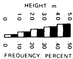
Figure 16. Comparison of annual wave roses for 1983 versus 1980-1982
