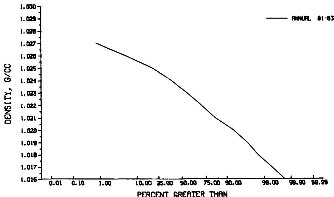
Figure 41. Distribution of surface water density for 1981 through 1983
