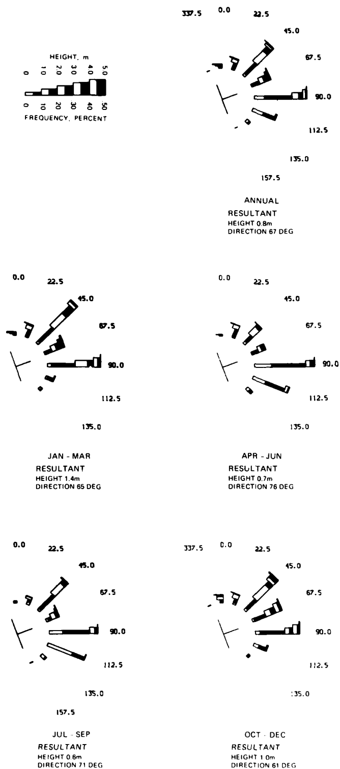
Figure B18. 1980 through 1983 annual and seasonal wave roses
