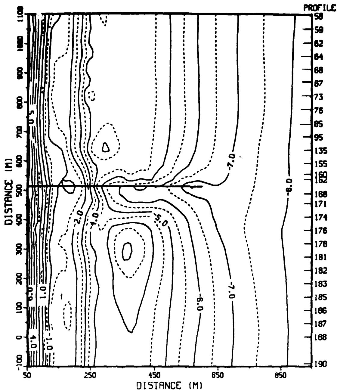
Figure C10. FRF bathymetry, 21 November 1983 (contours in metres)
