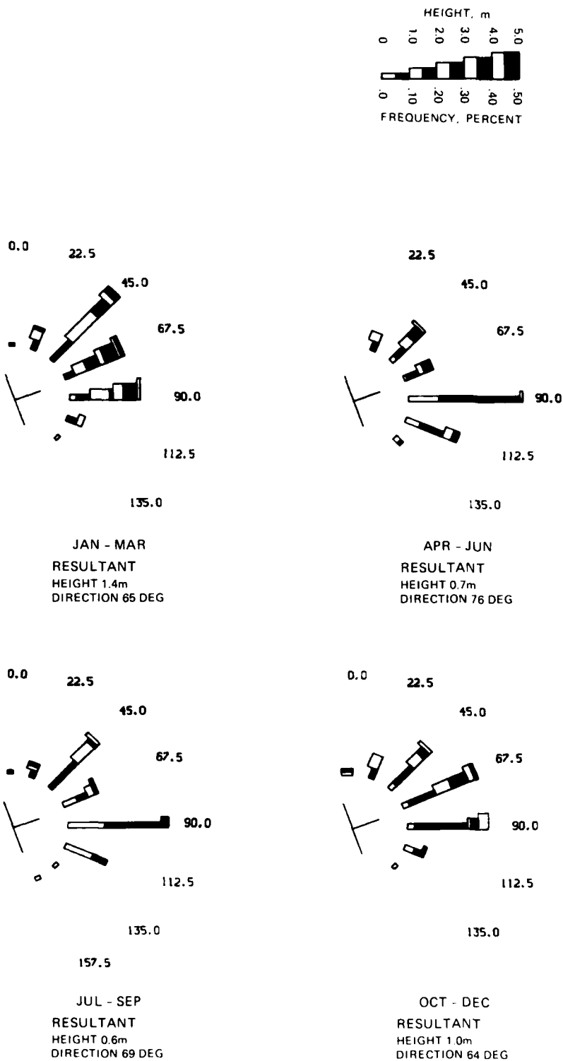
Figure 17. Seasonal variation of wave direction distributions for 1983
