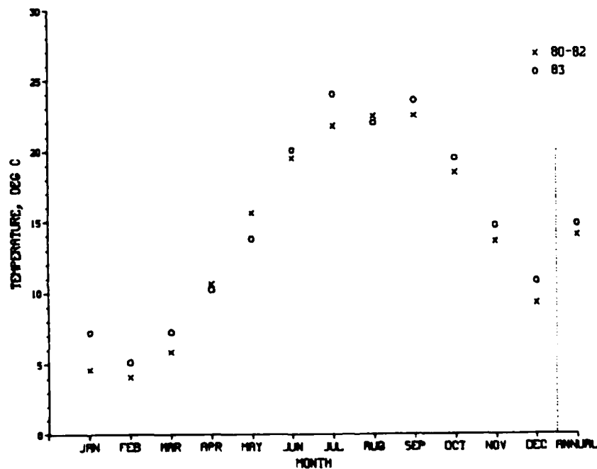
Figure 34. Comparison of mean surface water temperatures
