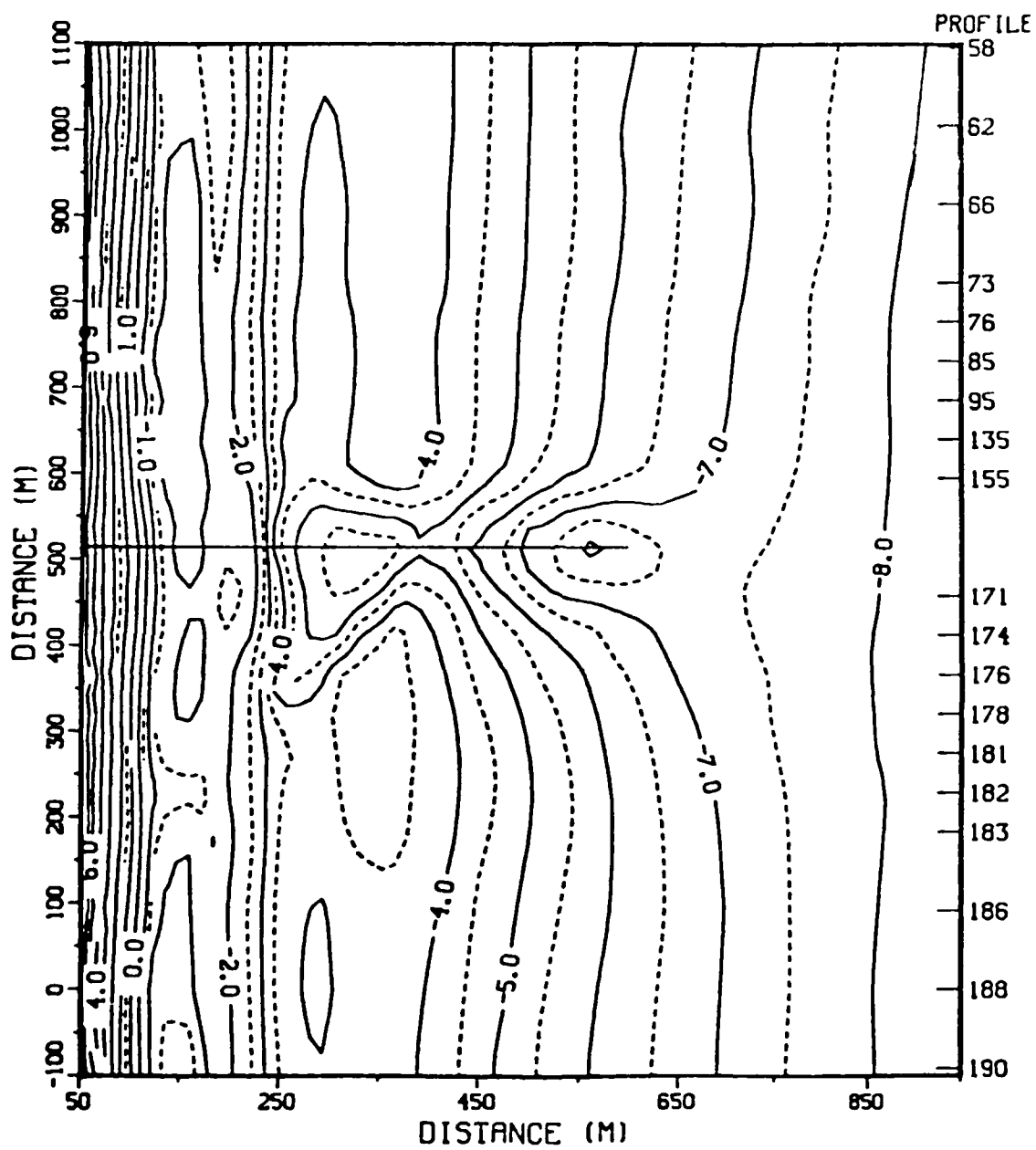
Figure C1. FRF bathymetry, 13 January 1983 (contours in metres)
