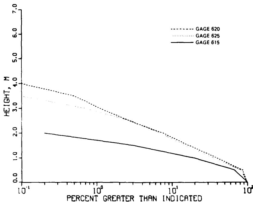
Figure 20. Wave height distributions, 1980 through 1983
