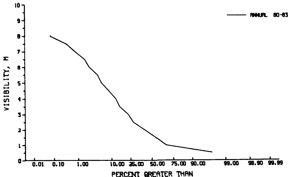
Figure 38. Distribution of surface water visibility for 1980 through 1983
