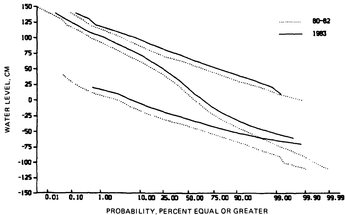
Figure 31. Comparison of hourly tide heights and daily high/low water level distributions
