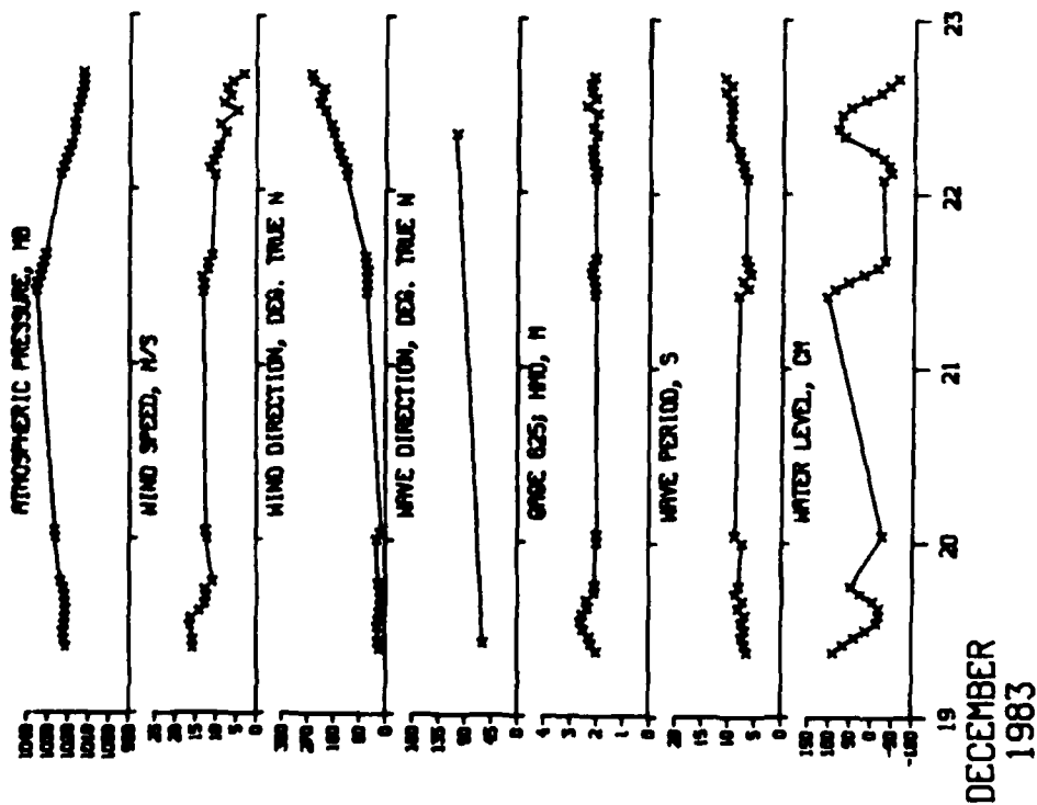
Figure D23. Storm data for 19-22 December 1983
