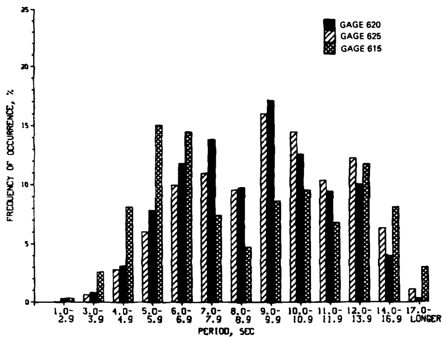
Figure 11. Annual wave period distributions for 1983
