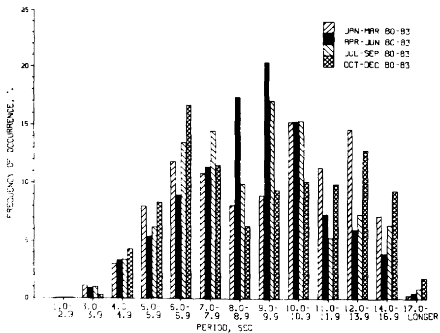
Figure 23. 1980 through 1983 seasonal wave period distributions for gage 625
