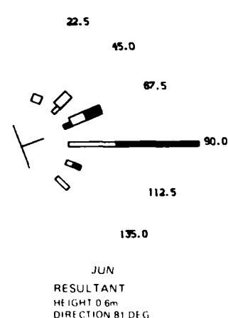
Figure B19. 1980 through 1983 monthly wave roses (Continued)
