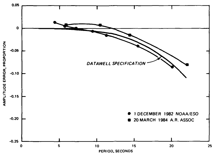
Figure A2. Waverider 67715-7 predeployment and postdeployment calibrations
