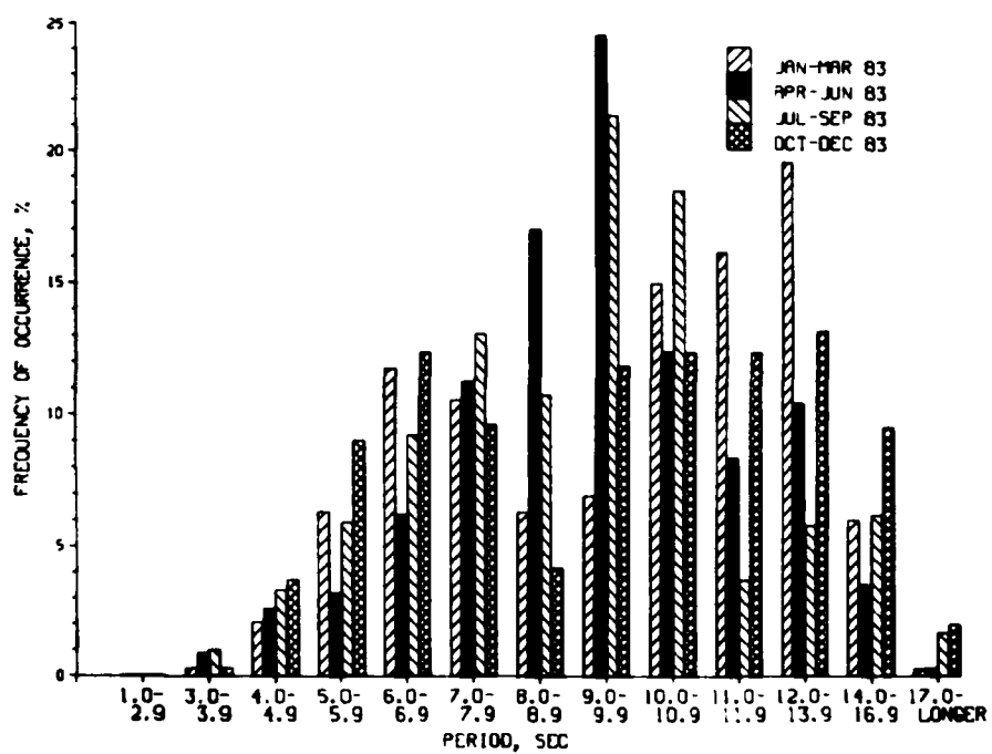
Figure B7. 1983 seasonal distribution of T_p for gage 625
