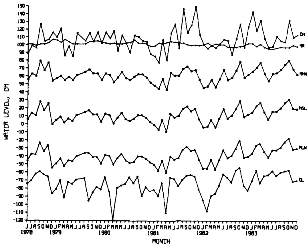
Figure 30. Monthly tide and water level statistics for 1978 through 1983
