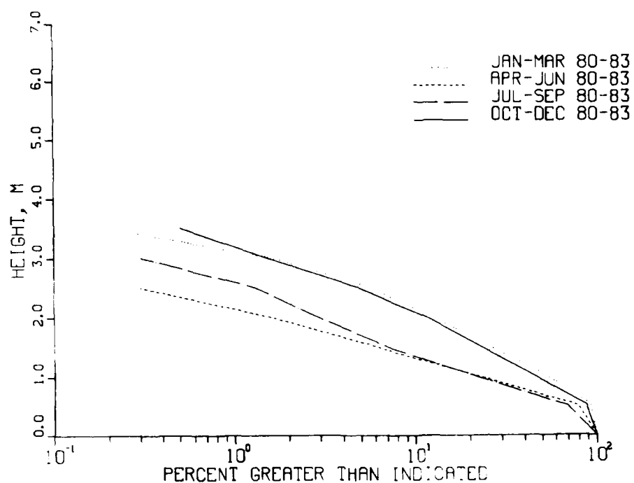
Figure 22. 1980 through 1983 seasonal wave height distributions for gage 625
