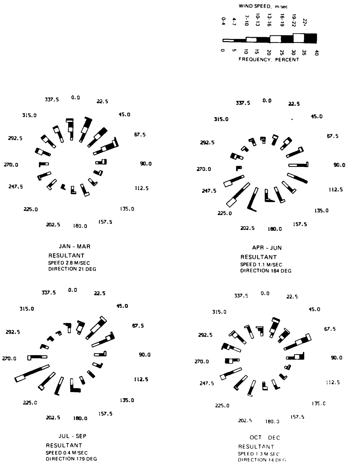
Figure 8. Seasonal wind roses for 1983
