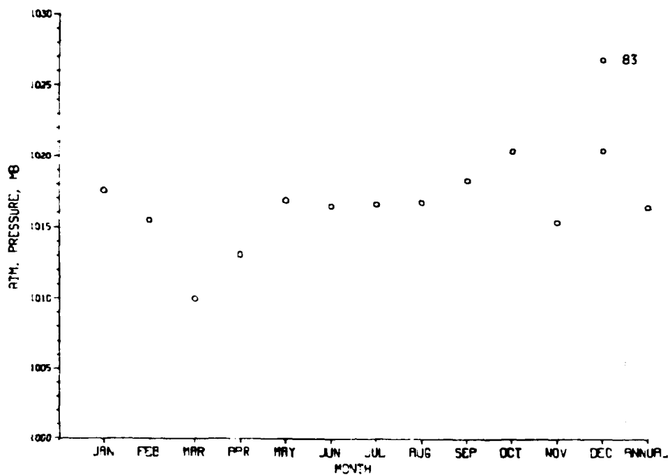
Figure 5. Atmospheric pressure, 1983
