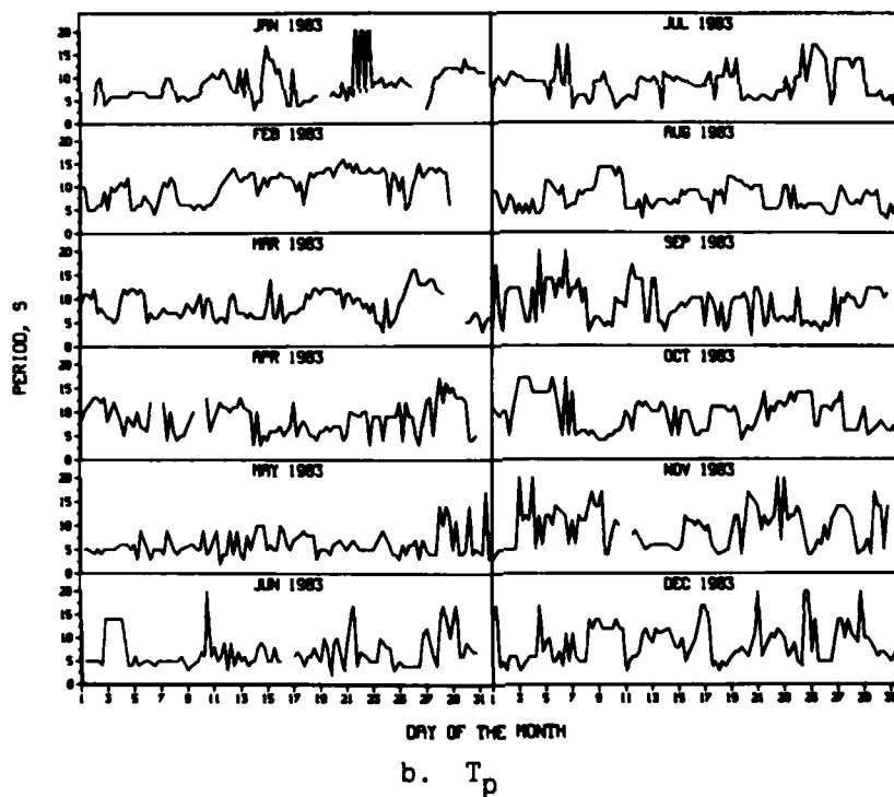
Figure B33. Time-history of H_{m0} and T_p for gage 615
