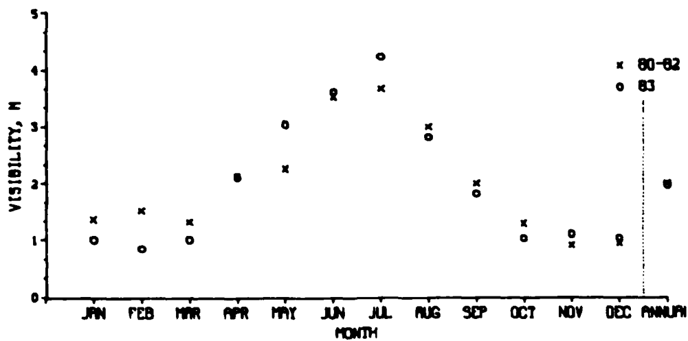
Figure 37. Comparison of mean surface water visibility
