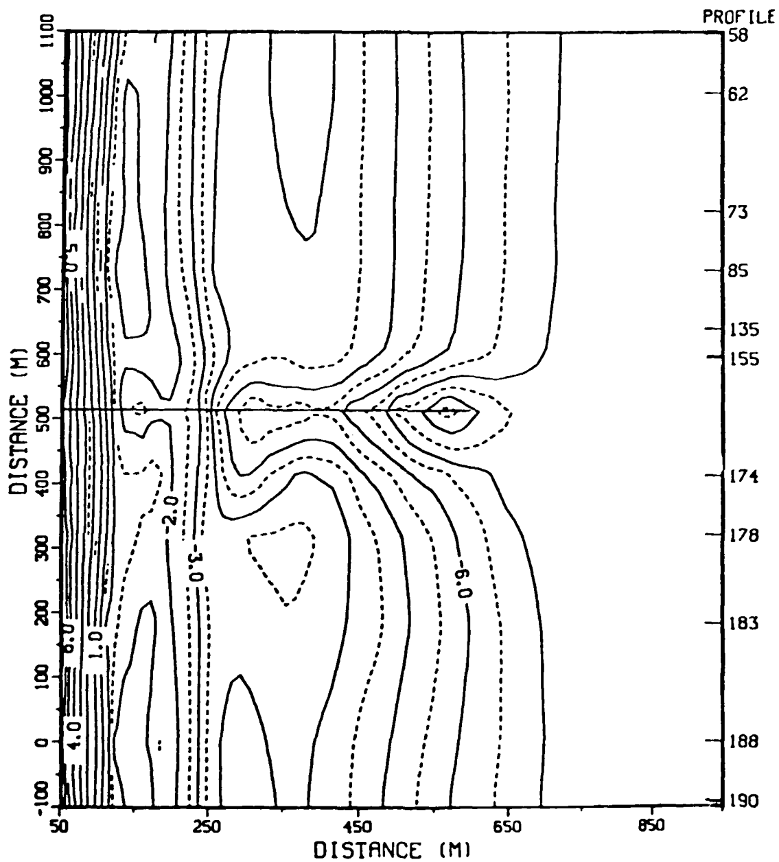
Figure C2. FRF bathymetry, 8 February 1983 (contours in metres)
