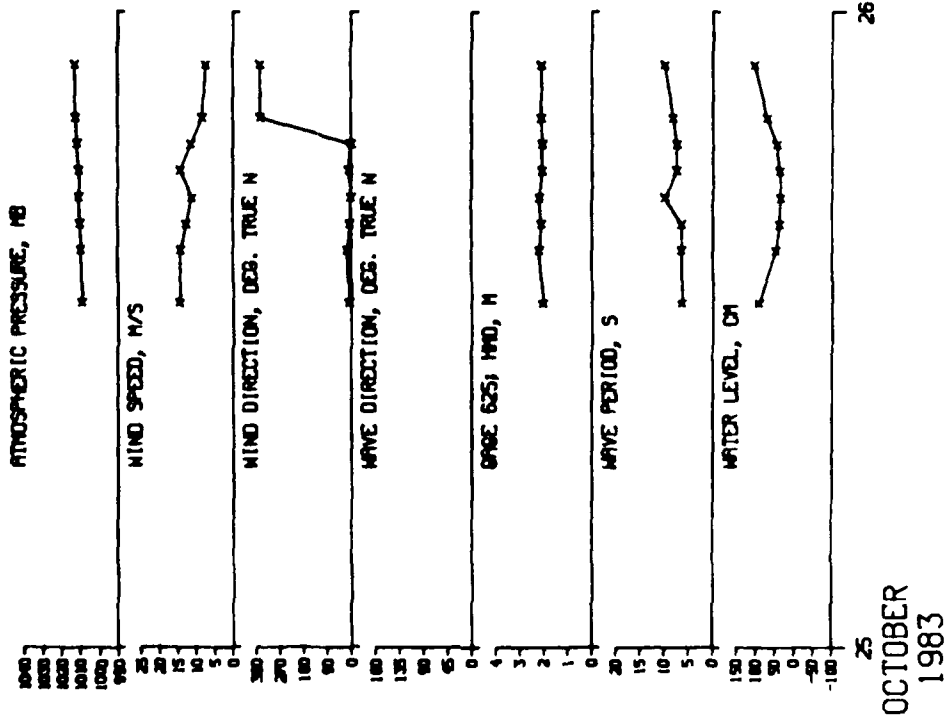
Figure D21. Storm data for 25 October 1983
