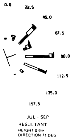
Figure 24. Annual and seasonal wave direction distributions, 1980 through 1983
