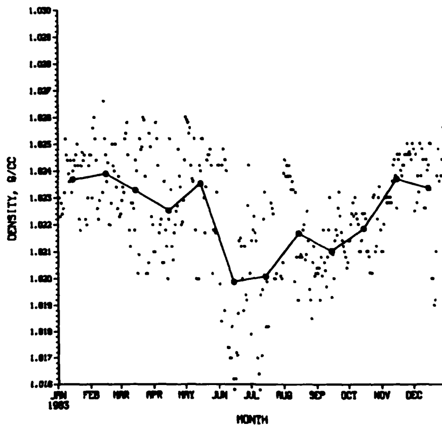
Figure 39. Daily sea-surface water density for 1983
