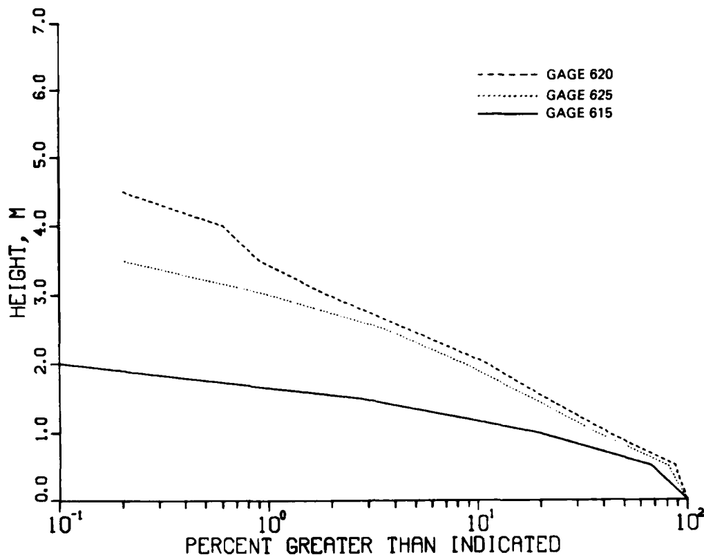
Figure 10. Annual wave height distributions for 1983
