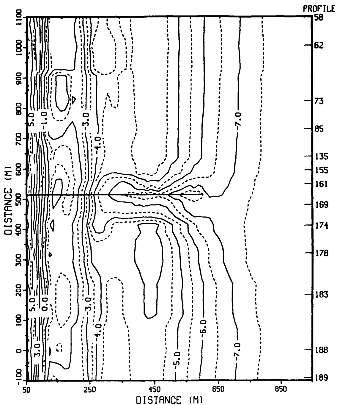
Figure C3. FRF bathymetry, 28 March 1983 (contours in metres)
