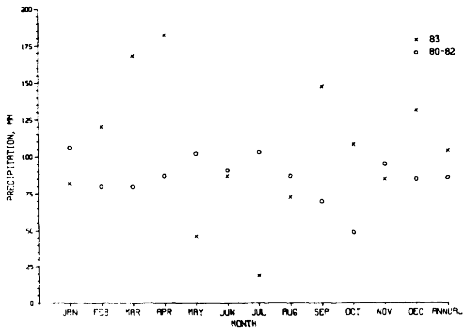
Figure 6. Precipitation, 1983
