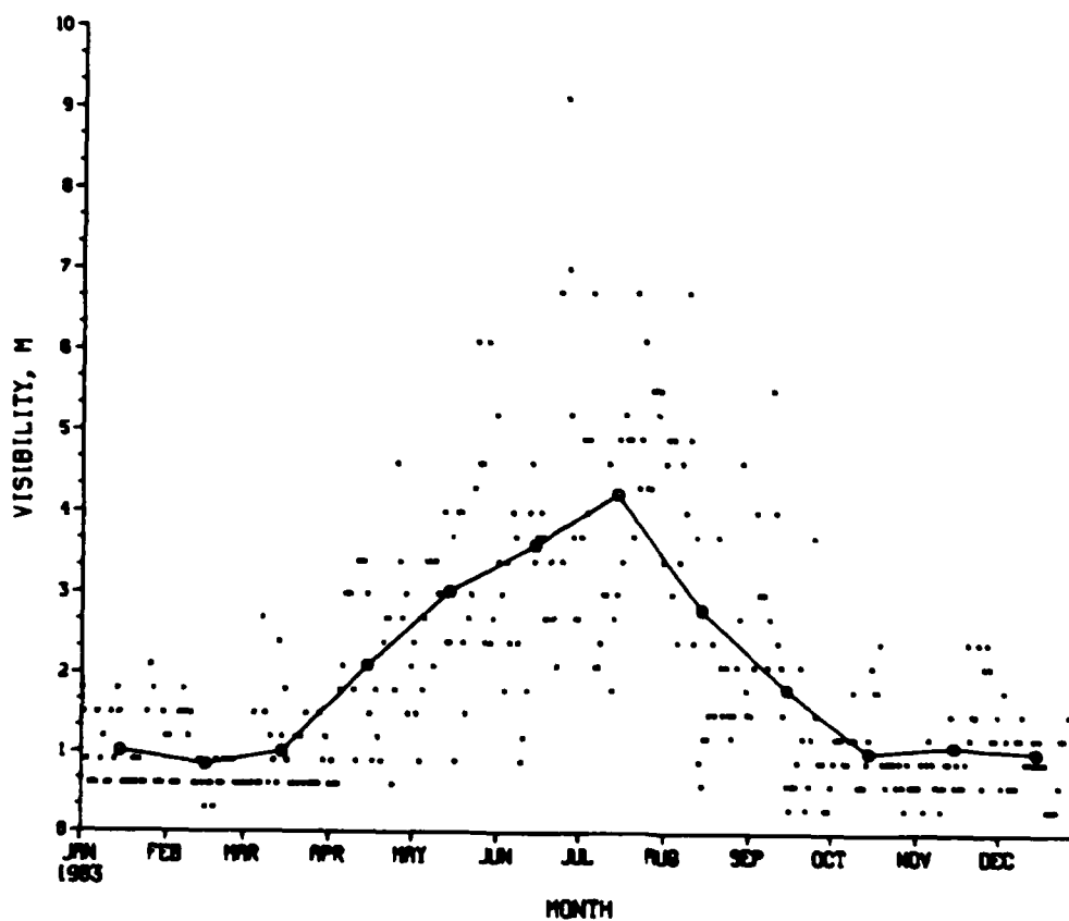
Figure 36. Daily sea-surface water visibility for 1983
