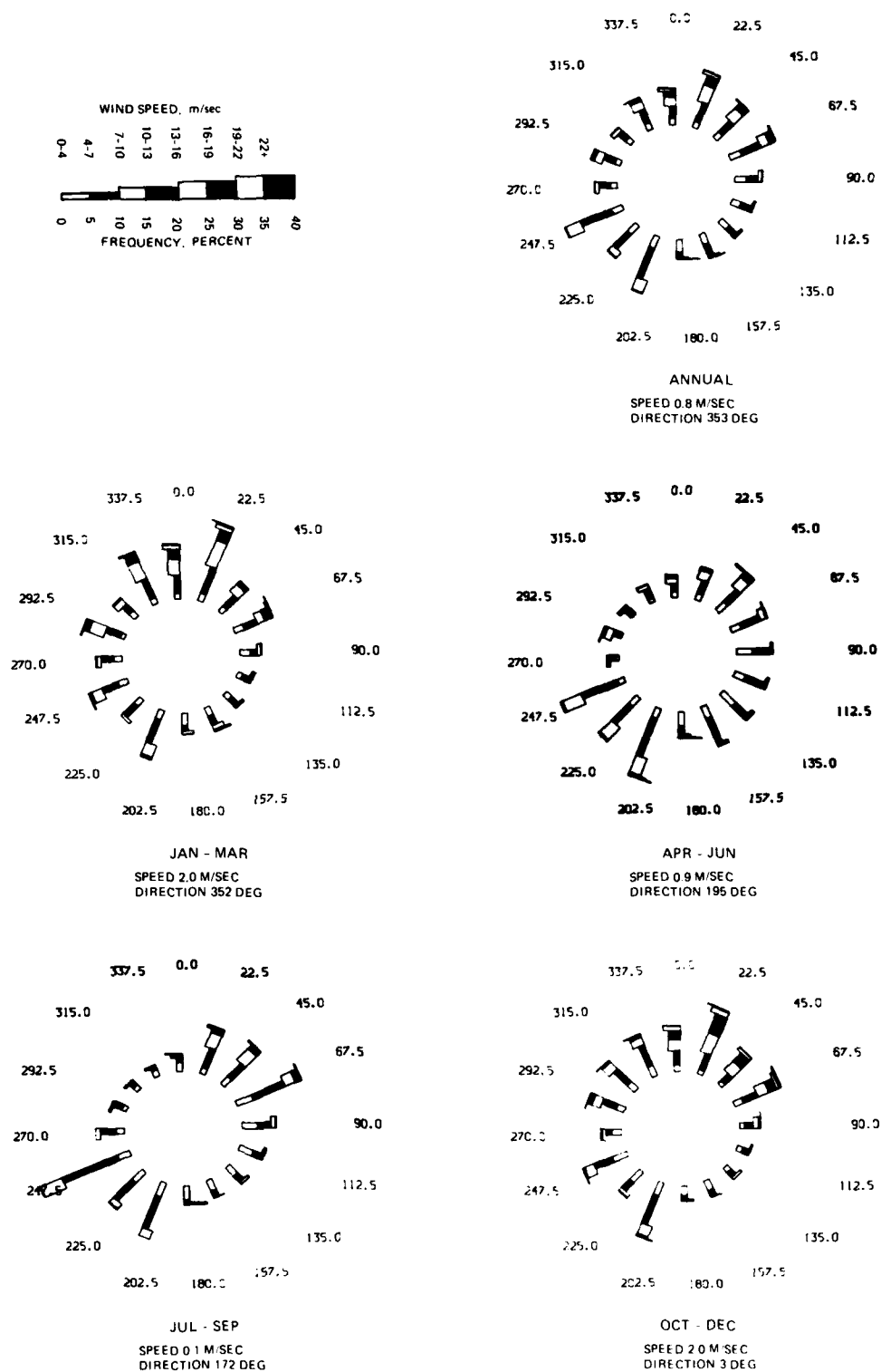
Figure 9. Annual and seasonal wind roses for 1980 through 1983
