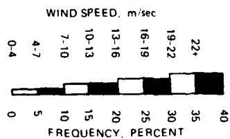
Figure 7. Comparison of annual wind roses for 1983 versus 1980-1982
