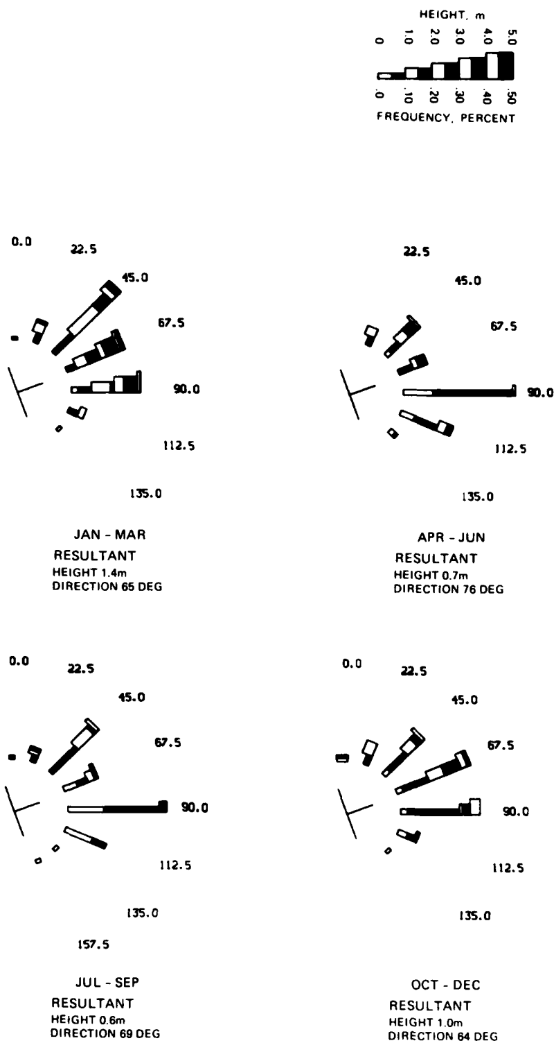
Figure B9. 1983 annual and seasonal wave roses
