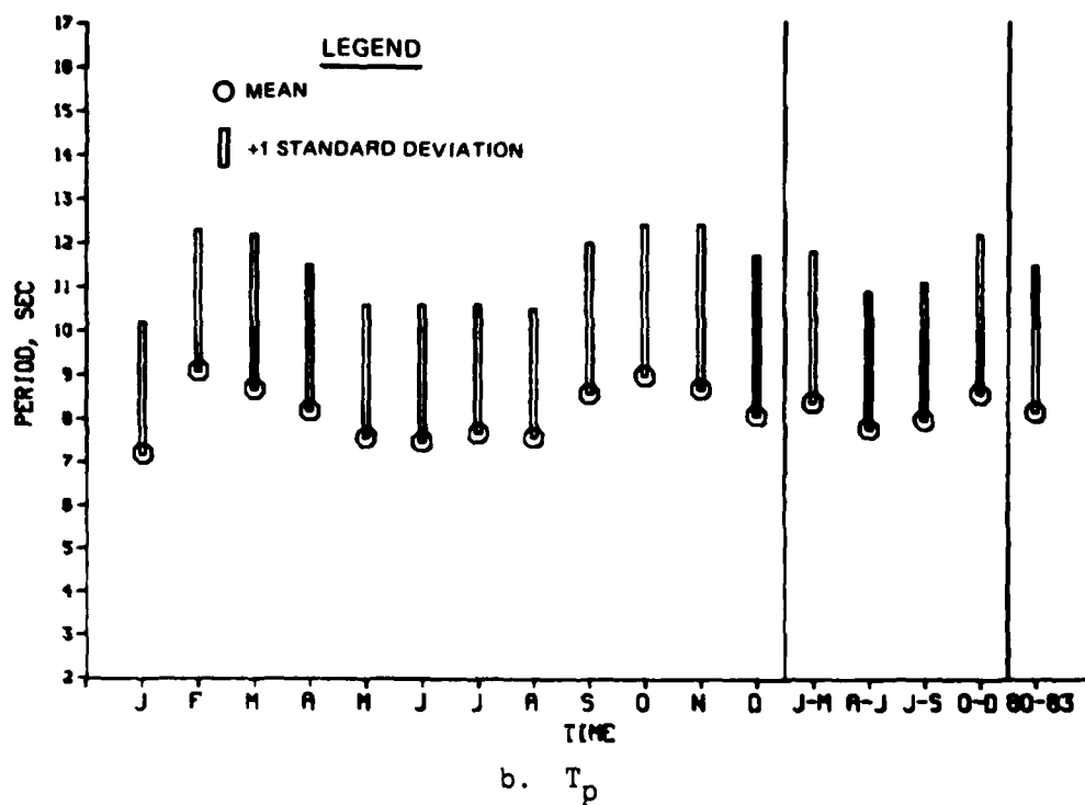
Figure B40. 1980 through 1983 mean, standard deviation, and extreme H_{m0} and T_p for gage 615
