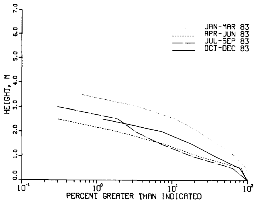
Figure 14. 1983 seasonal wave height distributions for gage 625
