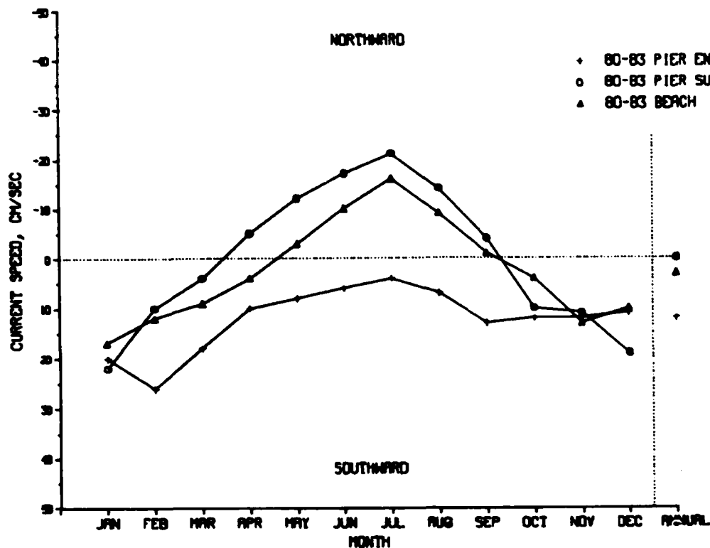
Figure 29. Comparison of surface currents at the FRF pier
