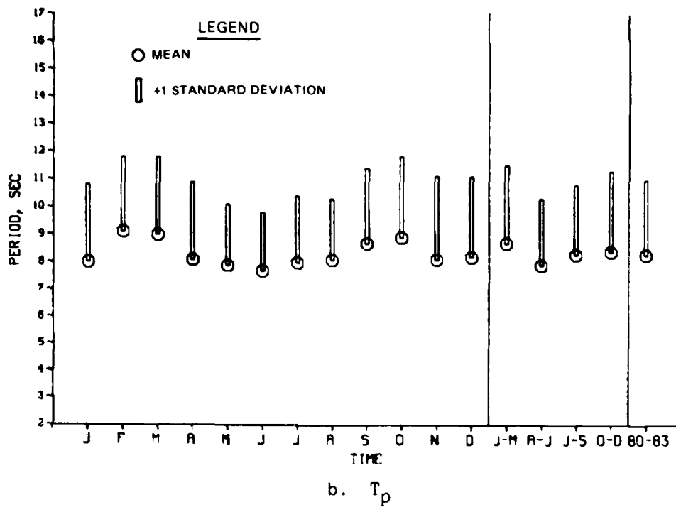
Figure B27. 1980 through 1983 mean, standard deviation, and extreme H_{m0} and T_p for gage 620
