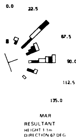
Figure B19. 1980 through 1983 monthly wave roses (Continued)
