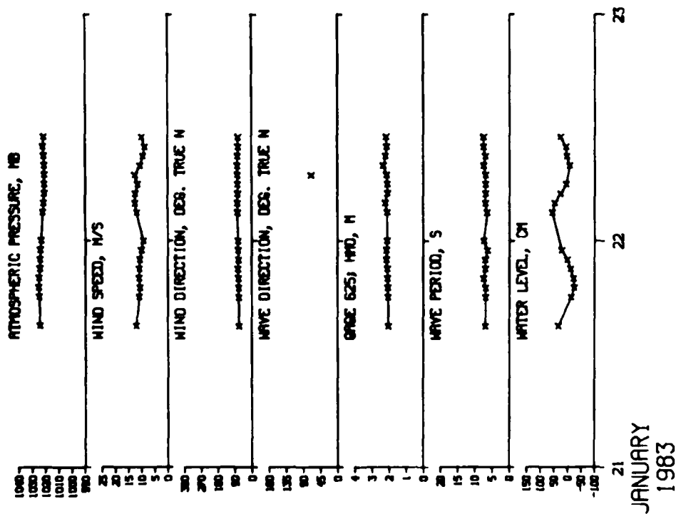
Figure D3. Storm data for 21 and 22 January 1983
