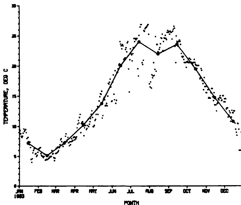
Figure 33. Daily sea-surface water temperature for 1983
