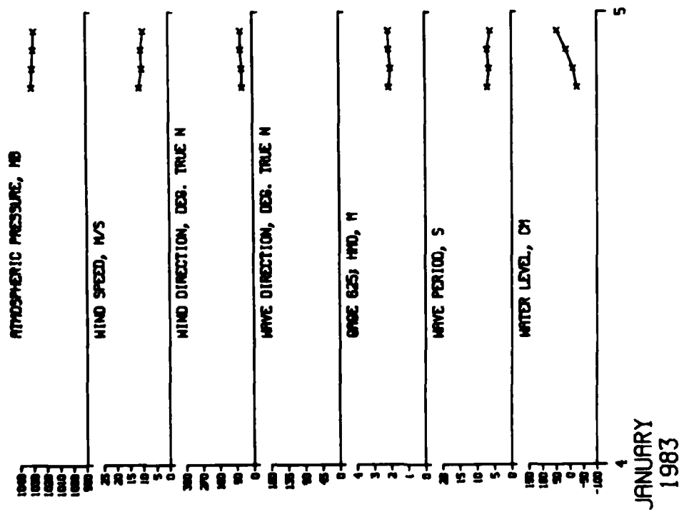
Figure D1. Storm data for 4 January 1983
