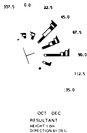
Figure 24. Annual and seasonal wave direction distributions, 1980 through 1983
