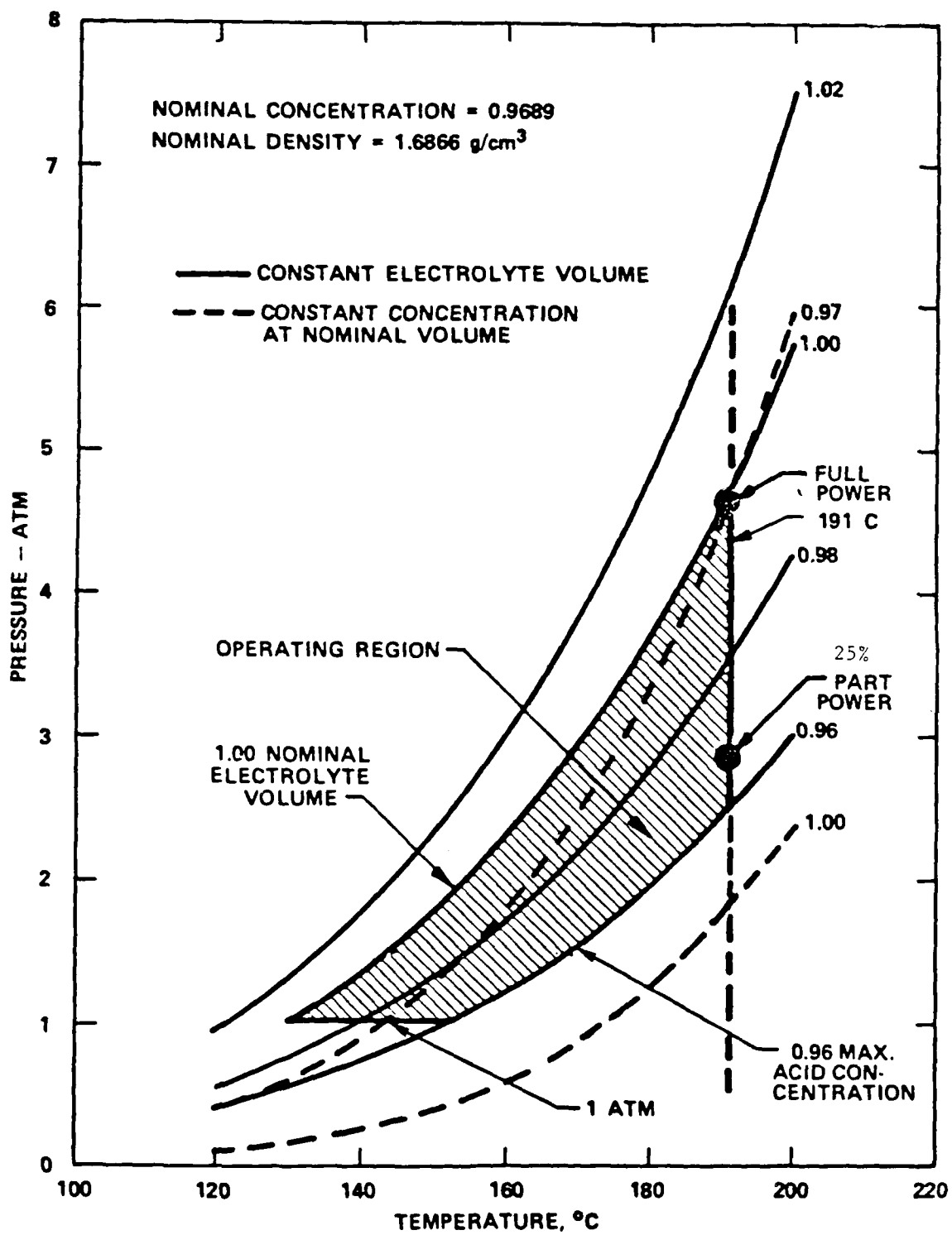
FIGURE 6.4-2 FUEL CELL OPERATING REGION FOR 50% AIR UTILIZATION
