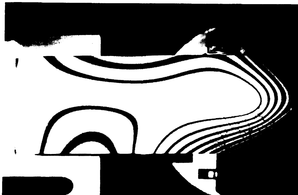
FIG.13 HOLOGRAM AT 1125 Hz FOR UNDAMAGED SPECIMEN
