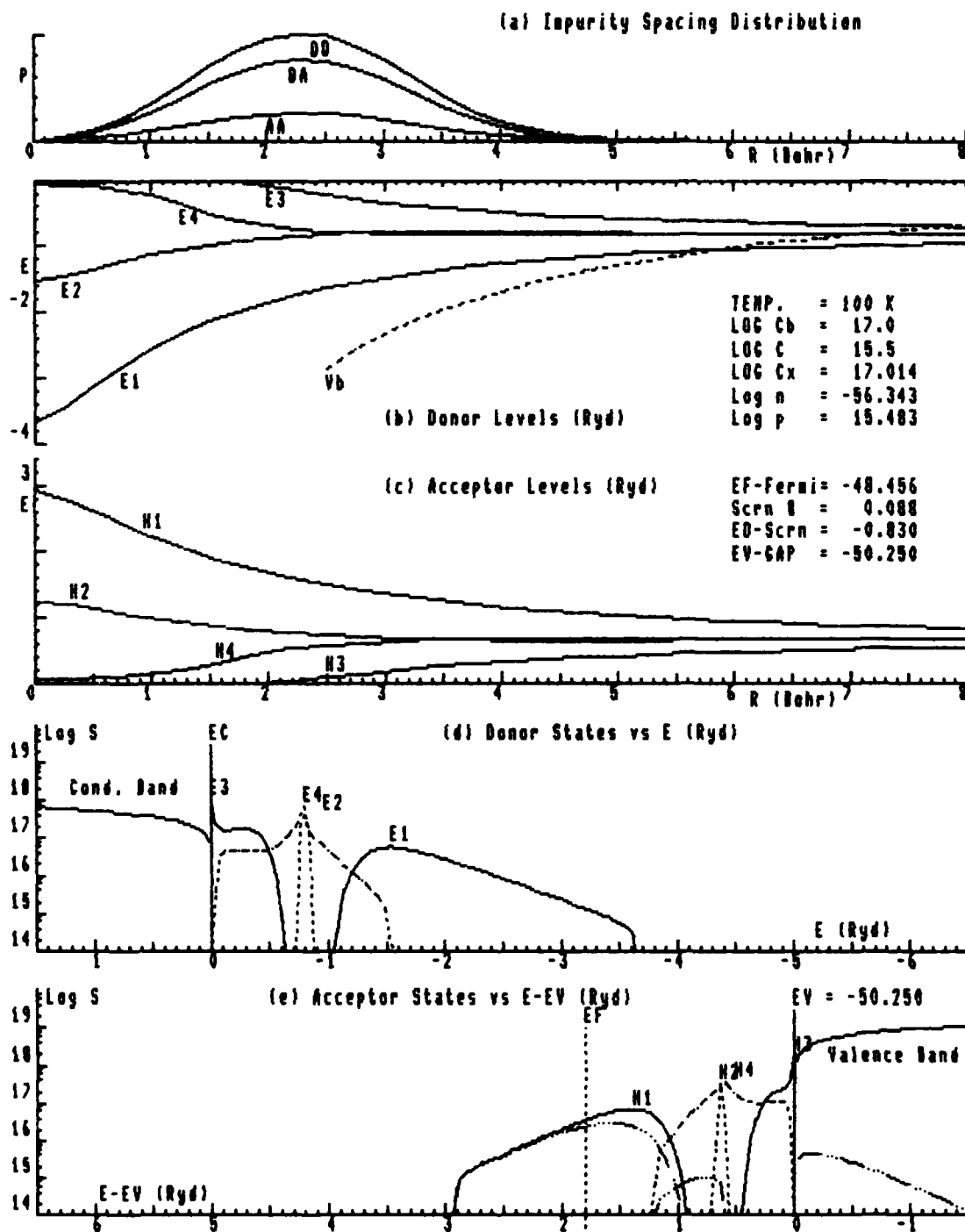
Fig. A 133. (a) Probability, AA + DA + DD, of Pairs vs R (b) Donor Energy E1; (DD)-, E2; (DD)-, E3; (DA)-, E4 (DA)- vs R (c) Acceptor En. H1; (AA)+, H2; (AA)+, H3; (AD)+, H4 (AD)+ vs R (d) Densities of Donor States, E1, E2, E3, & E4, vs E (e) Densities of Acceptor States, H1, H2, H3, & H4 vs E-EV.
