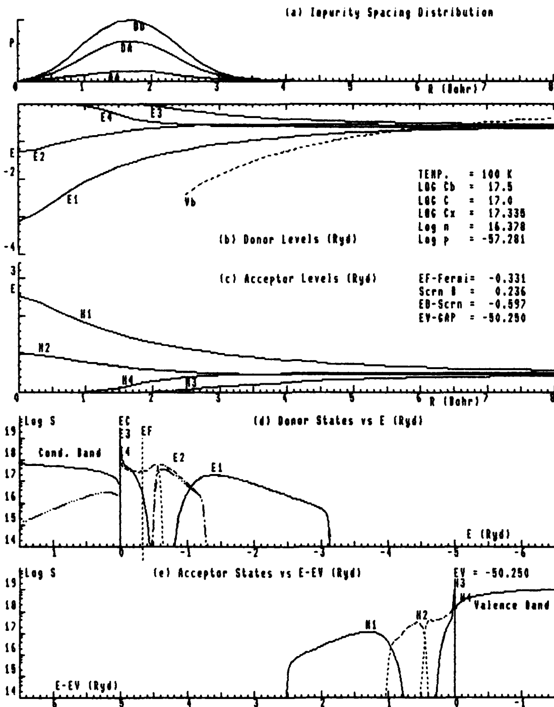
Fig. A 147. (a) Probability, AA + DA + DD, of Pairs vs R (b) Donor Energy E1; (DD)-, E2; (DD-)-, E3; (DA)-, E4 (DA+)- vs R (c) Acceptor En. H1; (AA)+, H2; (AA+)+, H3; (AD)+, H4 (AD-)+ vs R (d) Densities of Donor States, E1, E2, E3, & E4, vs E (e) Densities of Acceptor States, H1, H2, H3, & H4 vs E-EV.
