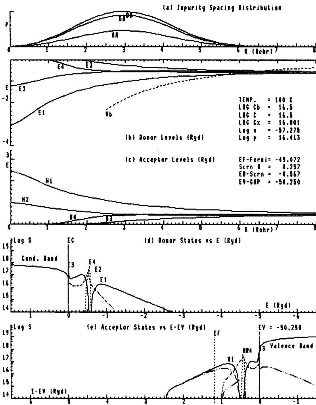
Fig. A 120. (a) Probability, AA + DA + DD, of Pairs vs R (b) Donor Energy E1;(DD)-, E2;(DD)-, E3;(DA)-, E4(DA+)- vs R (c) Acceptor En. H1;(AA)+, H2;(AA)+, H3;(AD)+, H4(AD)+ vs R (d) Densities of Donor States, E1, E2, E3, & E4, vs E (e) Densities of Acceptor States, H1, H2, H3, & H4 vs E-EV.
