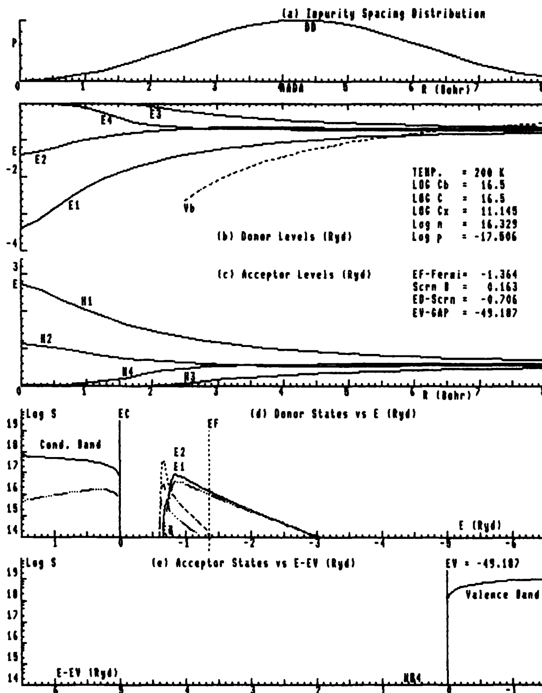
Fig. A 228. (a) Probability, AA + DA + DD, of Pairs vs R (b) Donor Energy E1;(DD)-, E2;(DD)-, E3;(DA)-, E4(DA+)- vs R (c) Acceptor En. H1;(AA)+, H2;(AA)+, H3;(AD)+, H4(AD-)+ vs R (d) Densities of Donor States, E1, E2, E3, & E4, vs E (e) Densities of Acceptor States, H1, H2, H3, & H4 vs E-EV.
