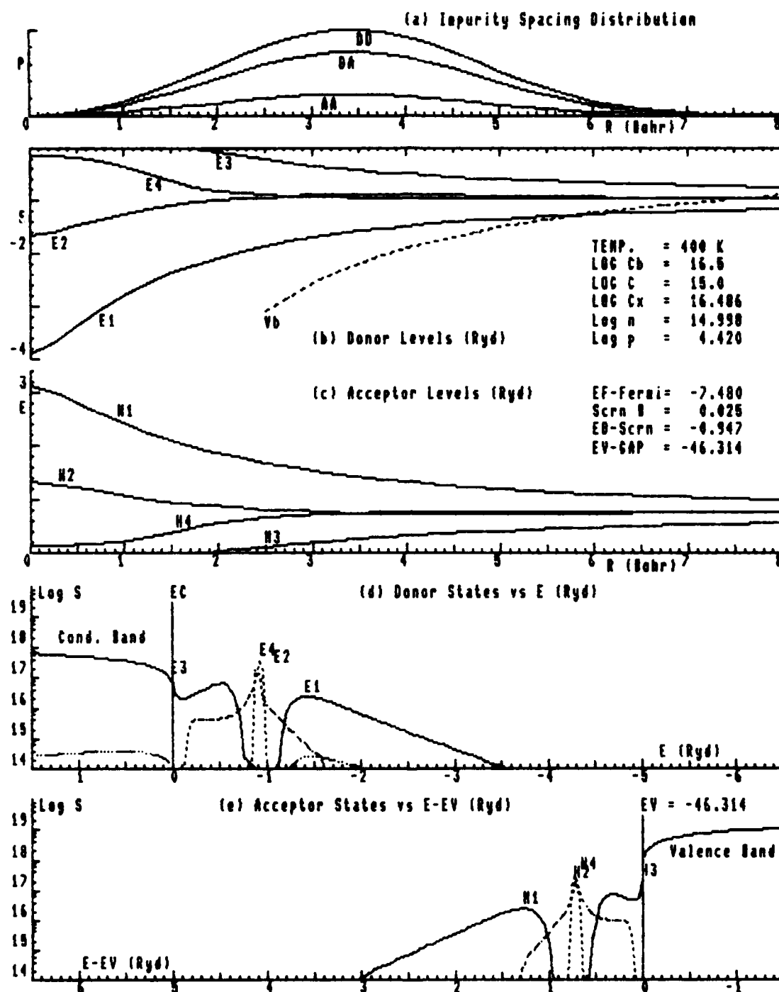
Fig. A 425. (a) Probability, AA + DA + DD, of Pairs vs R (b) Donor Energy E1;(DD)-, E2;(DD)-, E3;(DA)-, E4(DA+)- vs R (c) Acceptor En. H1;(AA)+, H2;(AA)+, H3;(AD)+, H4(AD)-+ vs R (d) Densities of Donor States, E1, E2, E3, & E4, vs E (e) Densities of Acceptor States, H1, H2, H3, & H4 vs E-EV.
