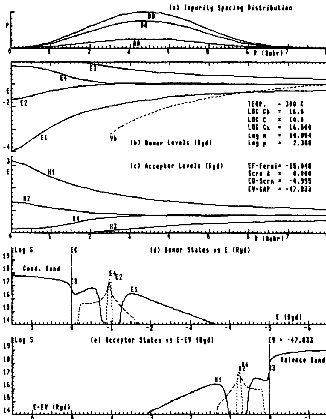
Fig. A 324. (a) Probability, AA + DA + DD, of Pairs vs R (b) Donor Energy E1;(DD)-, E2;(DD)-, E3;(DA)-, E4(DA+)- vs R (c) Acceptor En. H1;(AA)+, H2;(AA)+, H3;(AD)+, H4(AD-)+ vs R (d) Densities of Donor States, E1, E2, E3, & E4, vs E (e) Densities of Acceptor States, H1, H2, H3, & H4 vs E-EV.
