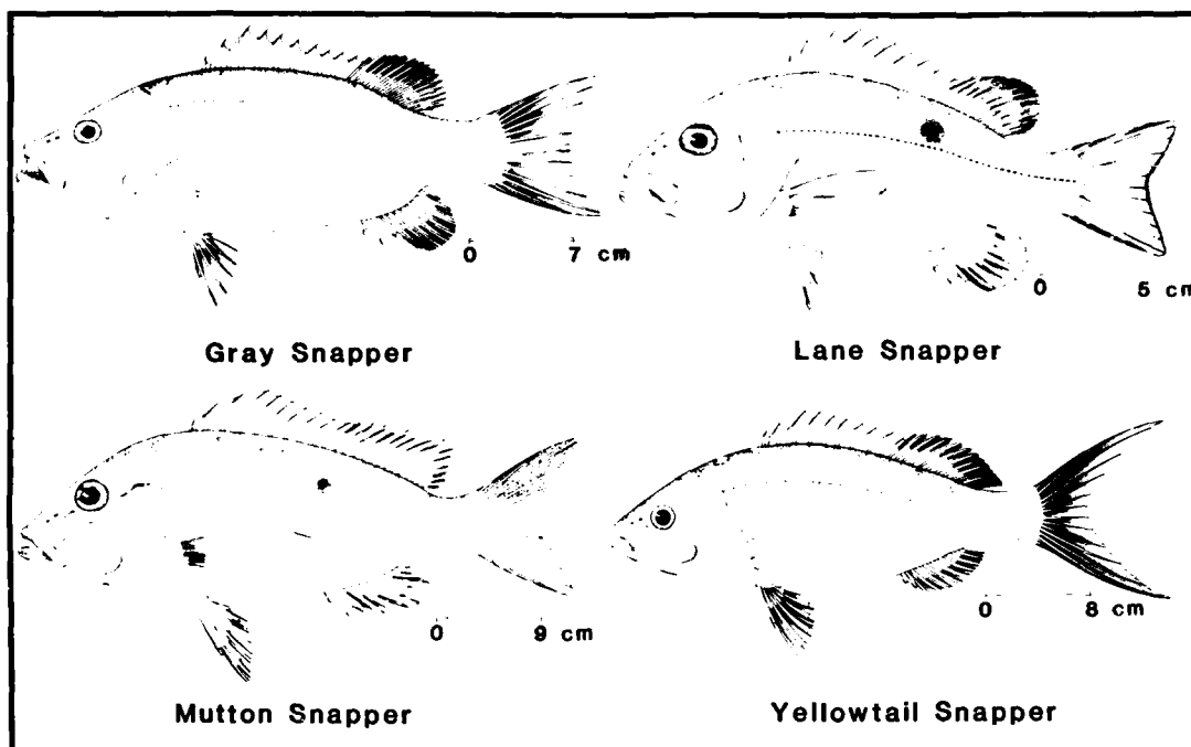
Figure 1. Gray, lane, mutton, and yellowtail snappers. Adapted from illustrations in Evermann and Marsh (1902).
