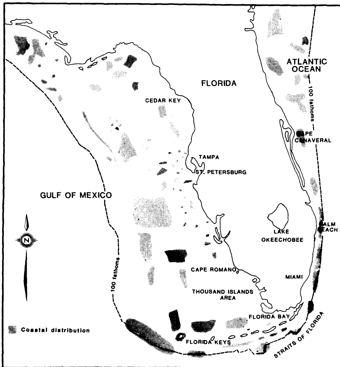
Figure 2. The distribution of the preferred habitat of adult snappers (hard bottoms including both natural and artificial reefs) off the south coast of Florida.
