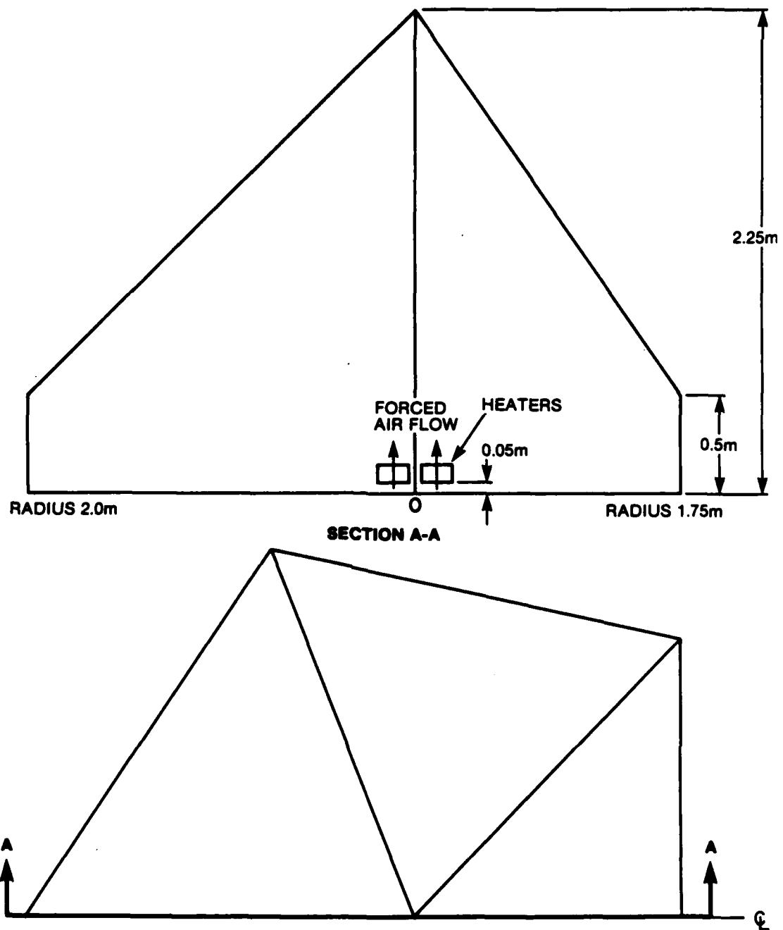
Figure 3: Schematic of the Canadian Forces, 5-Man, Arctic Tent used in the experimental portion of this study.
