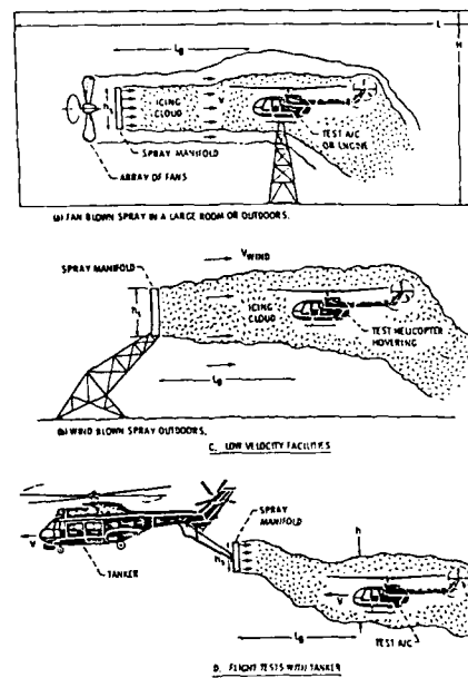
Fig. 30. Types of icing simulation facilities.
