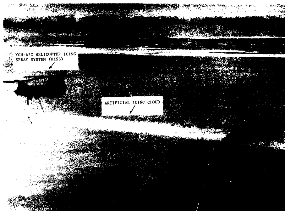
Fig. 33. UH-60A artificial icing test behind HISS.
