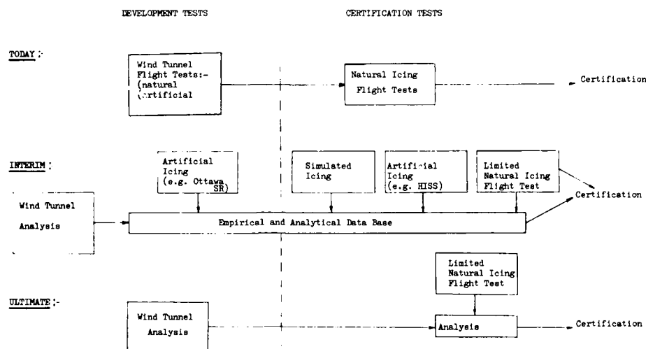
Fig. 31. Proposed certification procedures.
