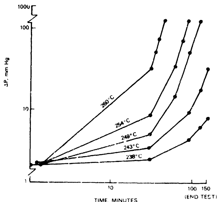
FIGURE 41. JFTOT ANALYSIS USING 5-MICROMETER TEST FILTERS IN CAT 1-H FUEL AT VARIOUS TEMPERATURES
