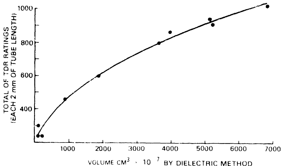
FIGURE 37. TOTAL OF TDR RATINGS VERSUS VOLUME BY DIELECTRIC METHOD
