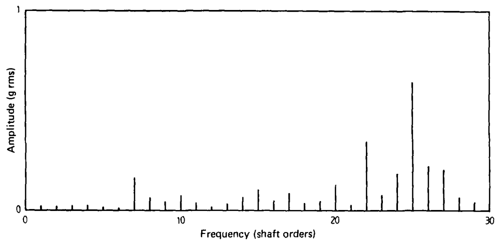
FIG. 35 LOW FREQUENCY SPECTRUM OF SIGNAL AVERAGE OF INPUT PINION OF GEARBOX WAK143 103 HOURS BEFORE FAILURE
