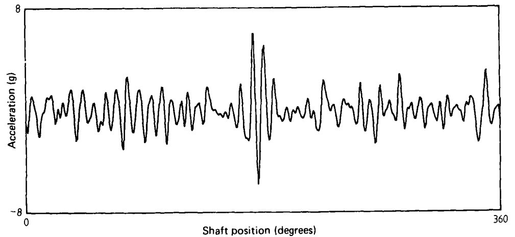
FIG. 24 SIGNAL AVERAGE OF INPUT PINION OF GEARBOX WAK143 103 HOURS BEFORE FAILURE MESHING HARMONICS AND GHOST ELIMINATED
