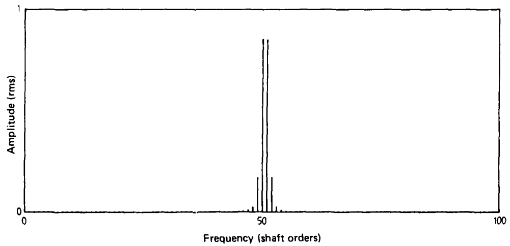
FIG. 9 SPECTRUM OF A SINUSOID BLOCK LENGTH = 50.5 PERIODS HANNING WEIGHTING
