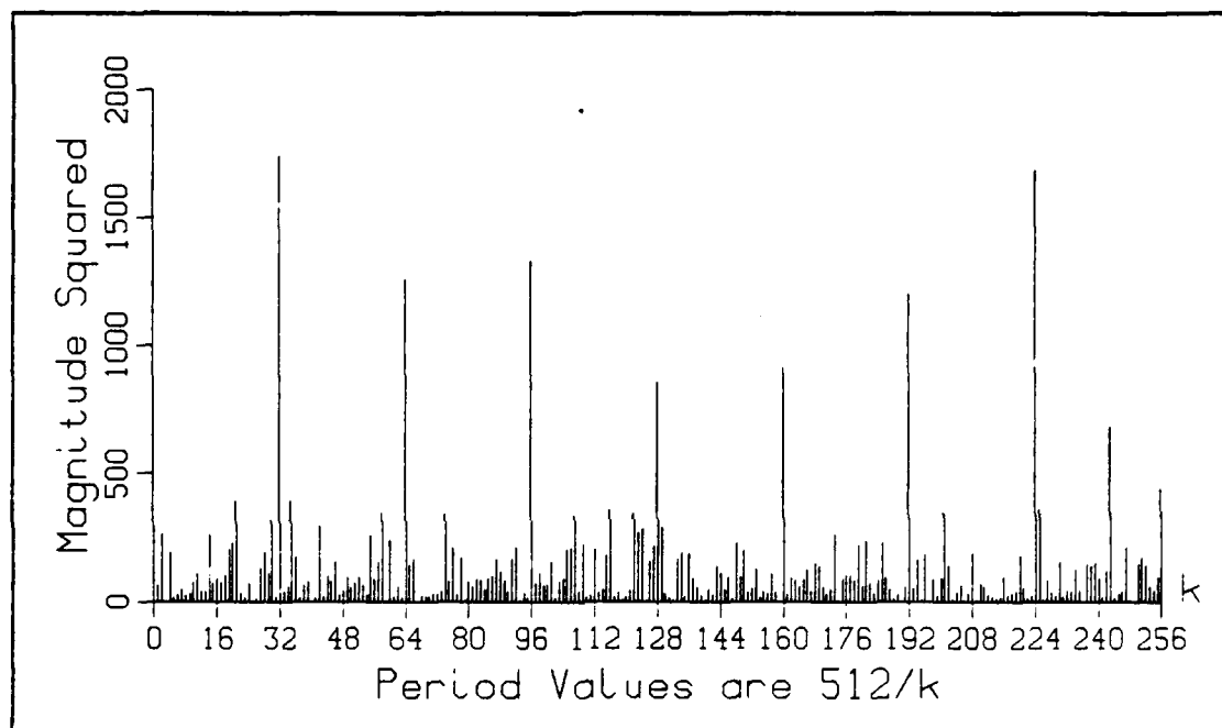
Figure 3.4 Burst Errors.
