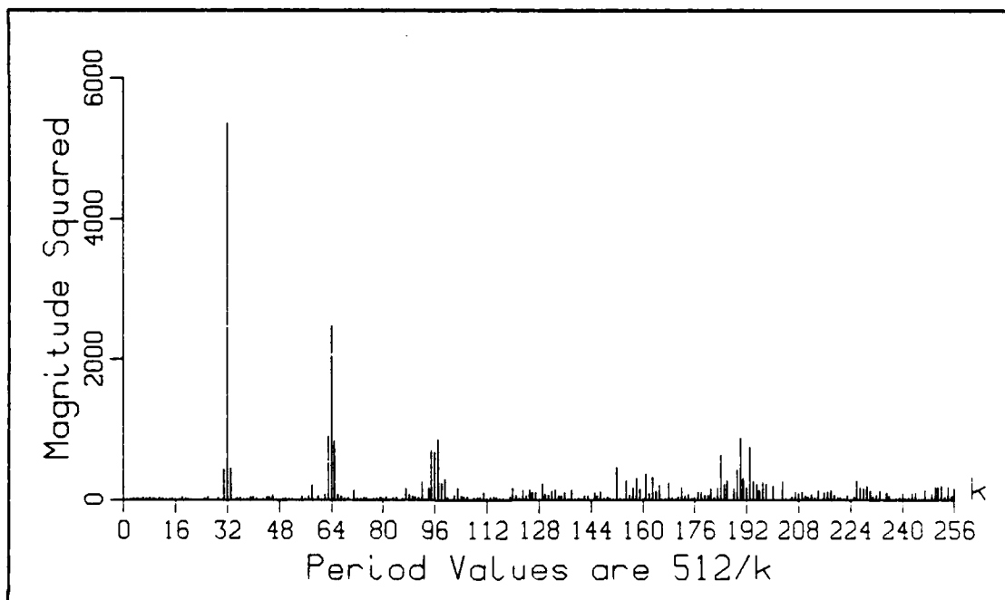
Figure 3.7 Timing Errors.
