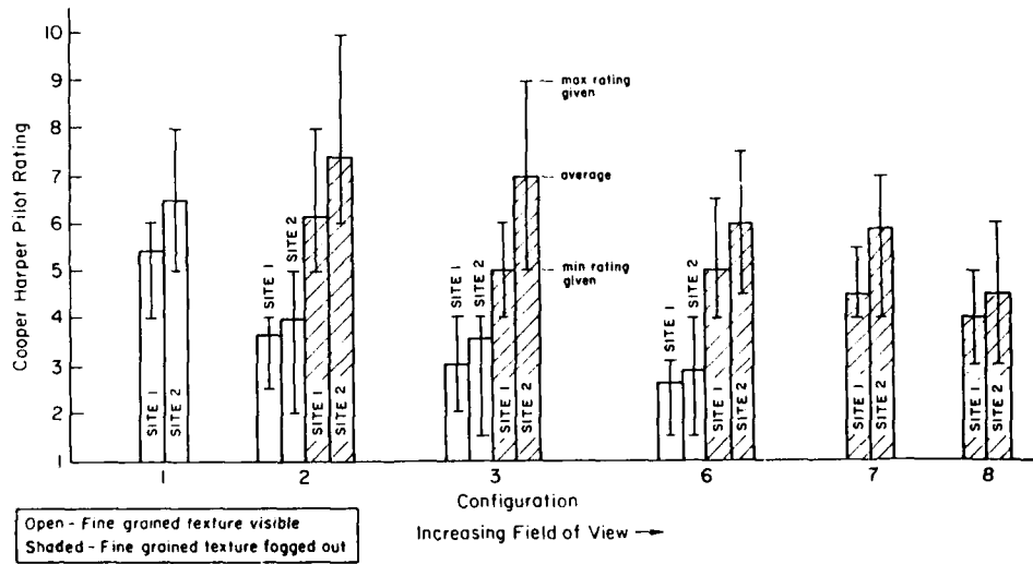
Figure 7. Cooper-Harper Pilot Ratings (Ref. 15)
