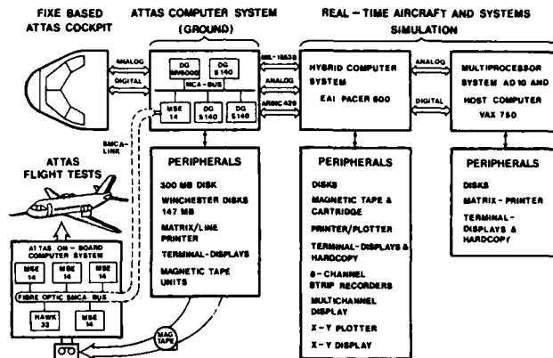
Fig.13 ATTAS real-time simulation facilities
