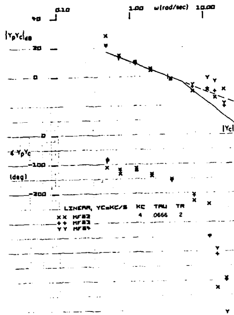
Figure 26. Y_p/Y_c Describing Function Amplitude and Phase Plot for Y_c = \frac{4e^{-0.067s}}{s(0.2s+1)} (Ref. 43)
