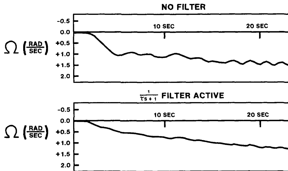
EFFECT OF 1/Ts+1 FILTER ON \Omega DURING A SPIN FIG. 5
