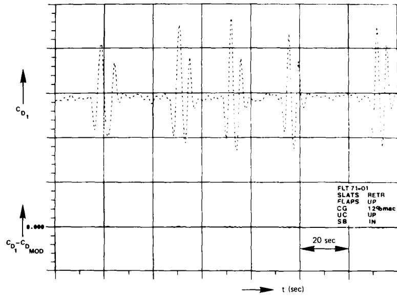
Fig. 8a Time history of C_{D1} and C_{D1} - C_{D1 model} as obtained from simulator test data
