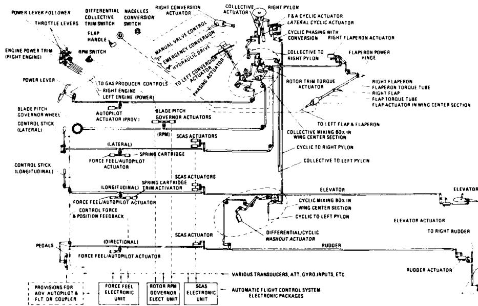
Fig. 6 Flight Control System Schematic
