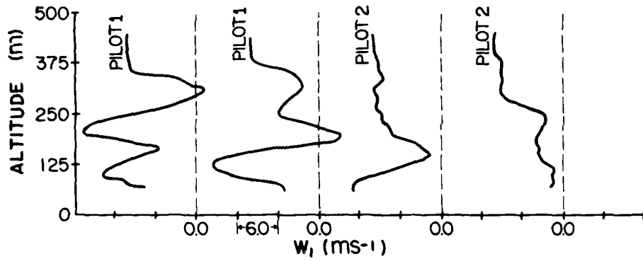
Figure 5. Winds Produced by the Direct Method Model.
