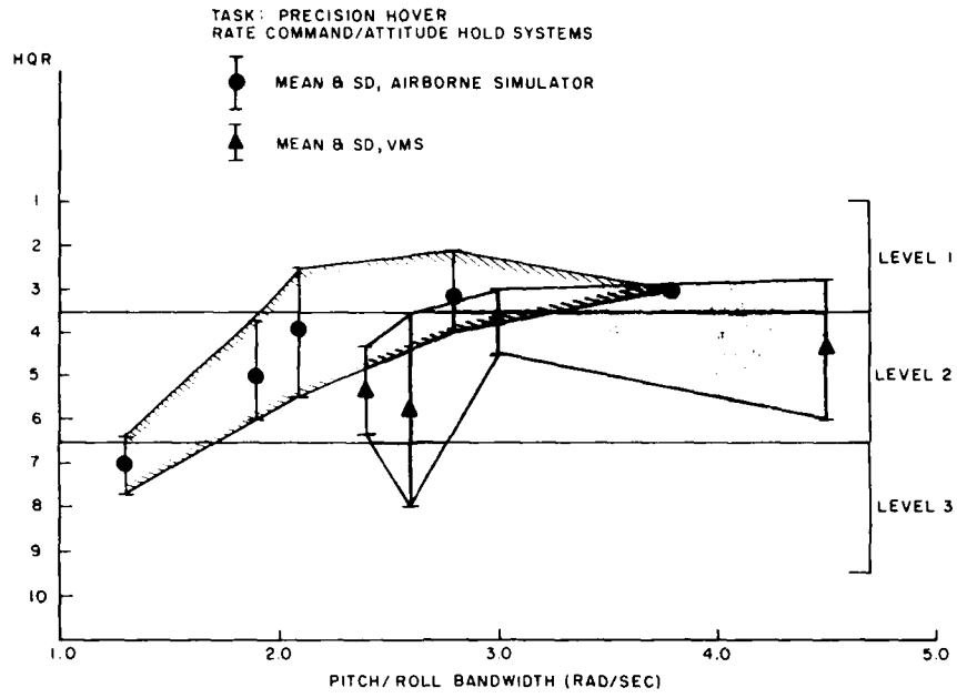
Fig.7 Data from rate command systems
