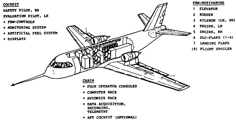
Fig.5 ATTAS modifications
