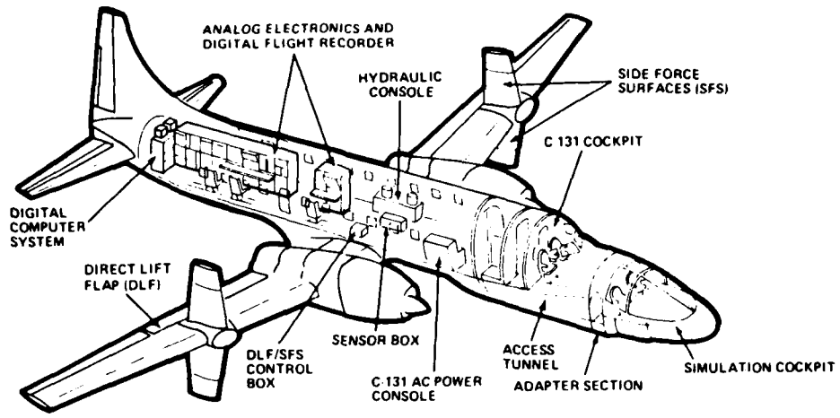
Fig. 1 TIFS General Arrangement
