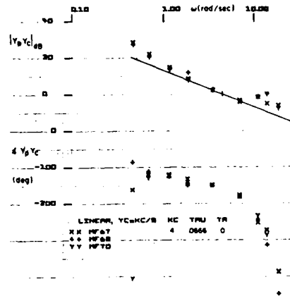
Figure 25. Y_p/Y_c Describing Function Amplitude and Phase Plot for Y_c = 4/s e^{-0.067s} (Ref. 43)
