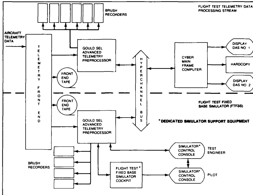
Fig. 3 Schematic of FTFS Integration into Existing Telemetry Processing/Ground Station Facilities
