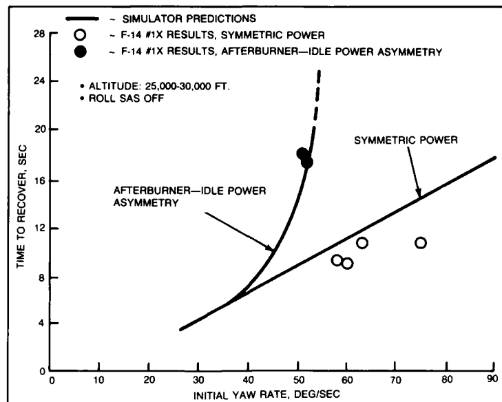
Fig. 11 F-14A Clean Configuration Recovery Boundary
