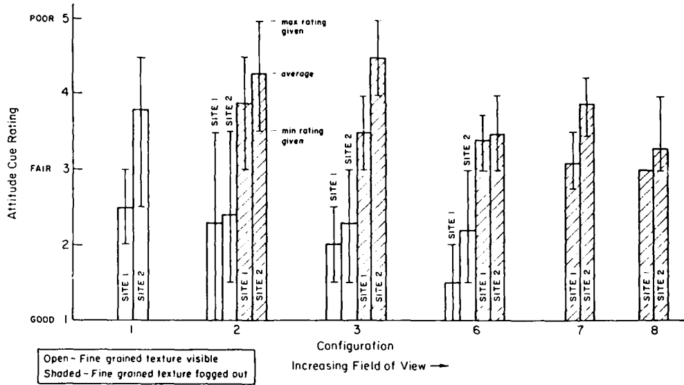
Figure 6. Attitude Cue Pilot Ratings (Ref. 15)
