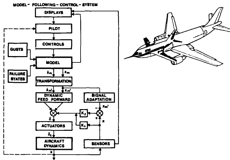
Fig.12 ATTAS model-following control scheme
