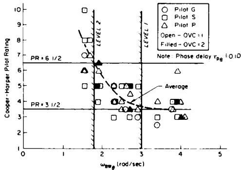
Figure 31. Pilot Rating vs. Pitch Attitude Bandwidth for ACAH Cases, Vertical Landing Task. Note: \omega_{wg} \approx \omega_{\psi} ; \tau_p \approx \tau_{\dot{\psi}} (Ref. 57)
