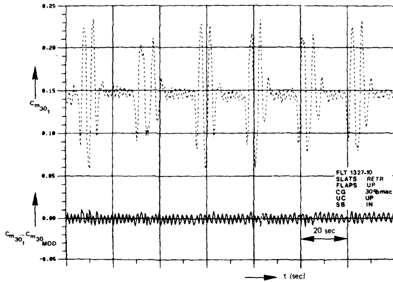
Fig. 9b Time history of C_{m_{30_1}} and C_{m_{30_1}} - C_{m_{30_1}} \text{ model} as obtained from flight test data
