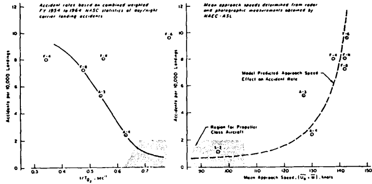
Figure 21. Implied Bivariate Dependency of Accident Rate on 1/T_{\theta_2} and Approach Speed (Ref. 39)
