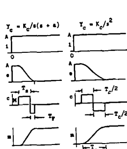
Figure 15. Ideal Time-Optimal Response Characteristics ( T_c is the time to complete the control program)
