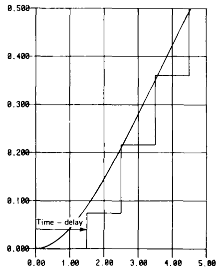
b: Second order Adams trapezoidal combination
