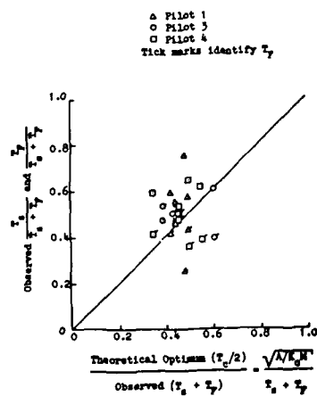
Figure 17. Control Pulse Intervals During the Rapid Response Interval in Bob-Up Maneuvers in the Simulator (Ref. 31)
