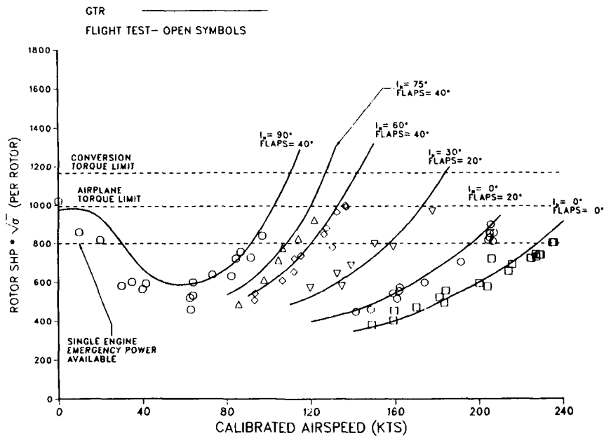
Fig. 14 XV-15 Level-Flight Performance
