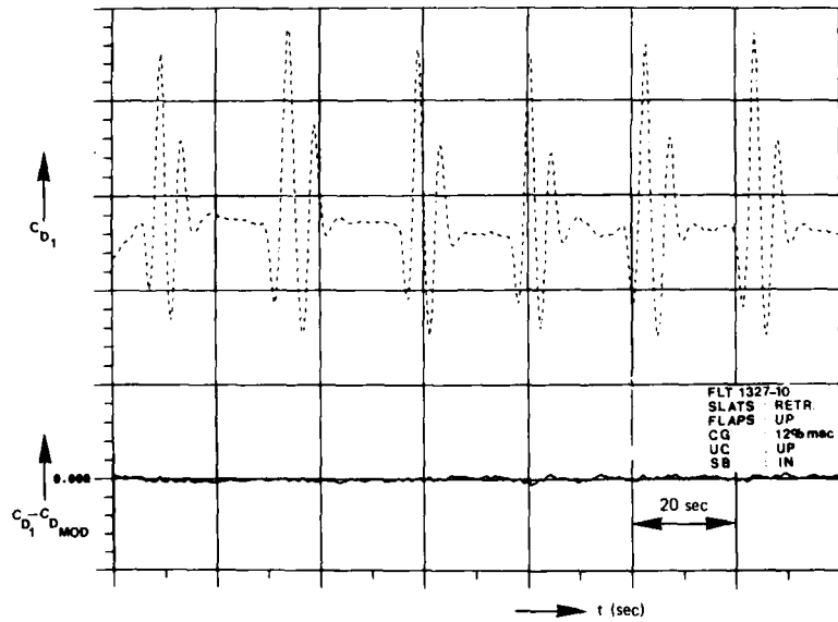
Fig. 8b Time history of C_{D1} and C_{D1} - C_{D1 model} as obtained from flight test data
