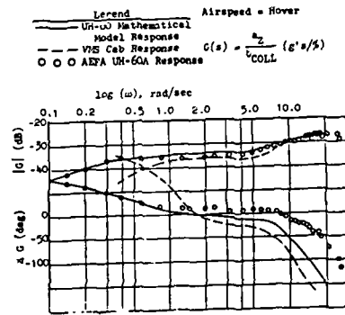
Figure 29. UH-60A Rotorcraft and Simulator Frequency Responses for the Transfer Function a_z/s_{COLL} at Hover (Ref. 31)
