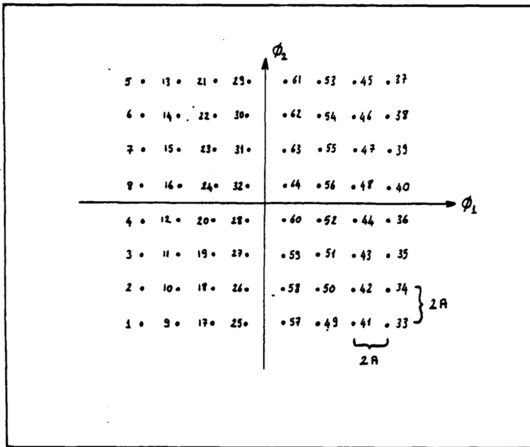
Figure 3.5. Signal Constellation for 64-QAM
