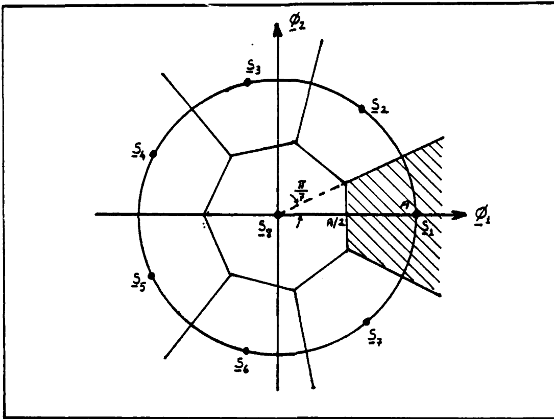
Figure 2.5. Signal-Space Diagram for (7+1) PSK Scheme
