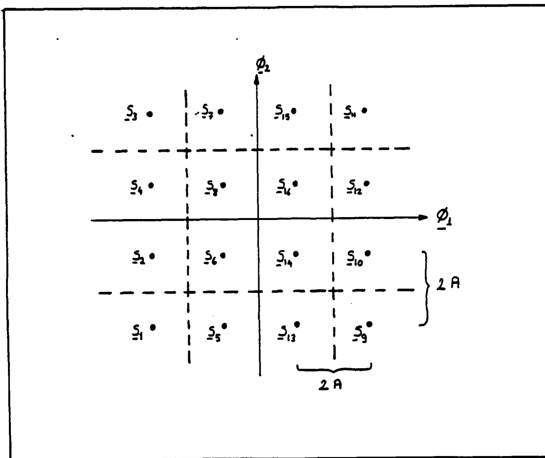
Figure 3.1. Signal Constellation and Decision Regions for 16-QAM
