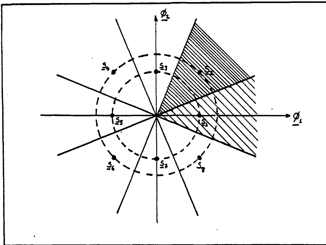
Figure 2.16. Signal-Space Diagram and Decision Region for MOD.1
