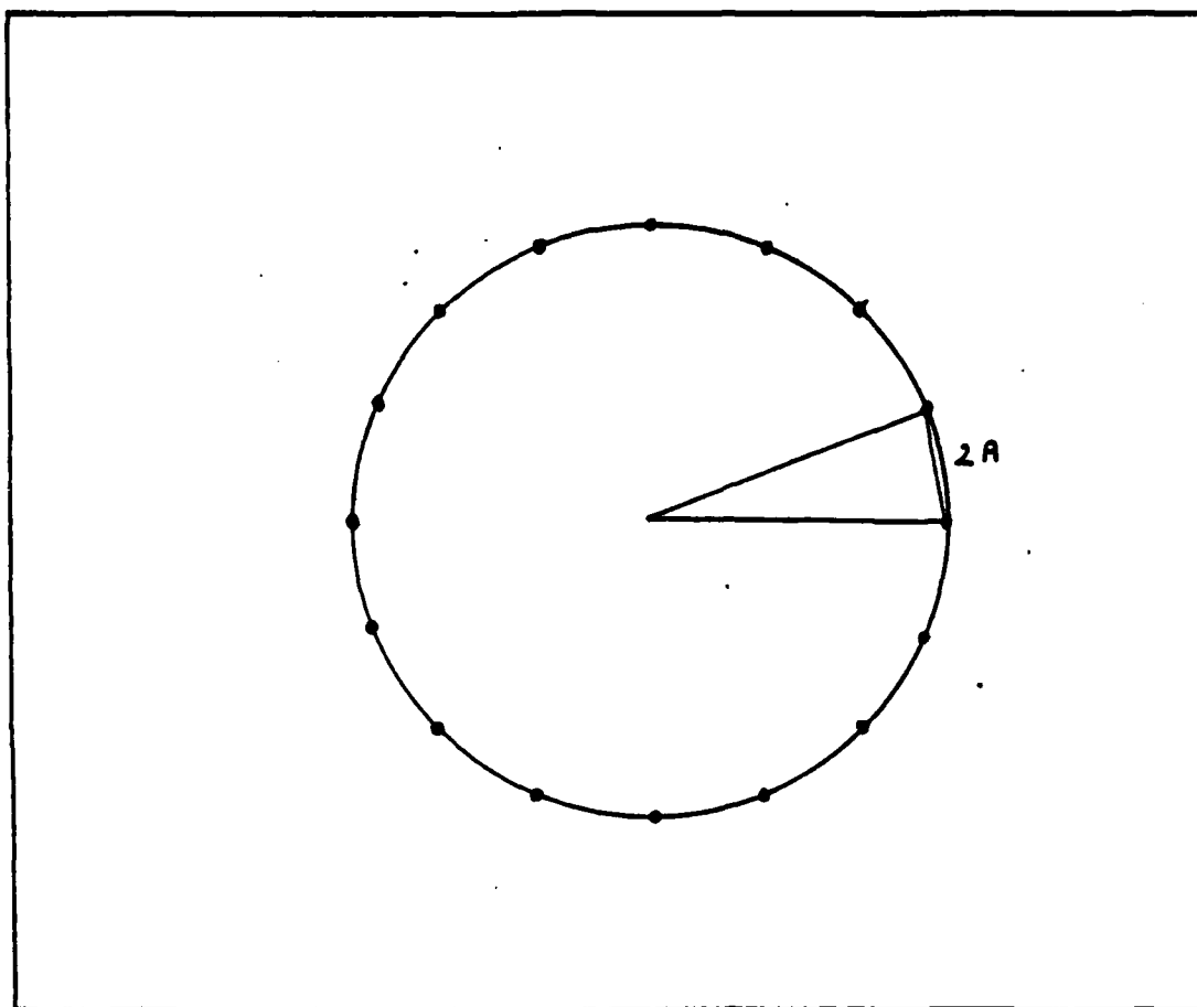
Figure 3.4. Signal Constellation for 16-PSK
