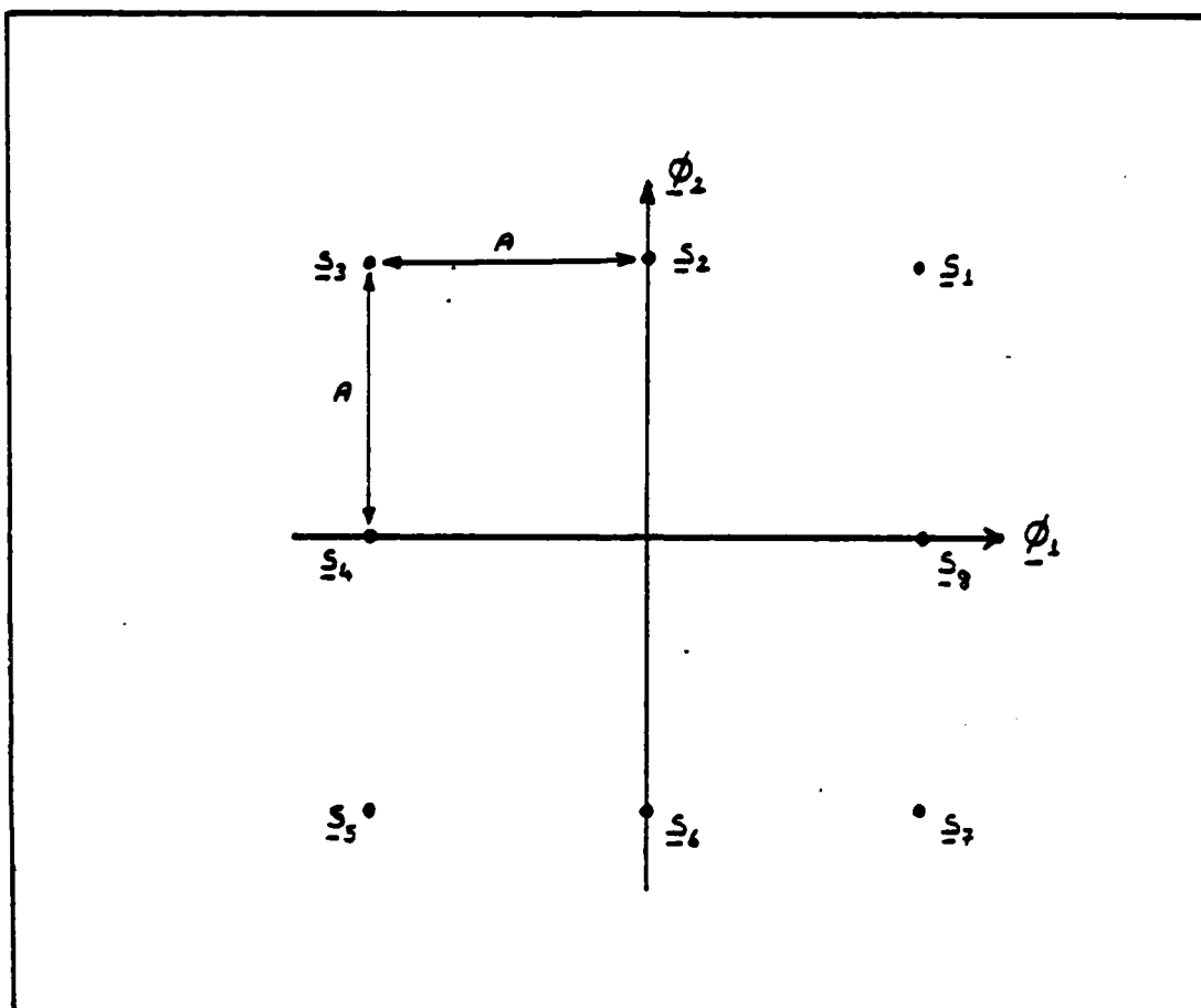
Figure 2.3. Signal-Space Diagram for Rectangular Signaling Scheme
