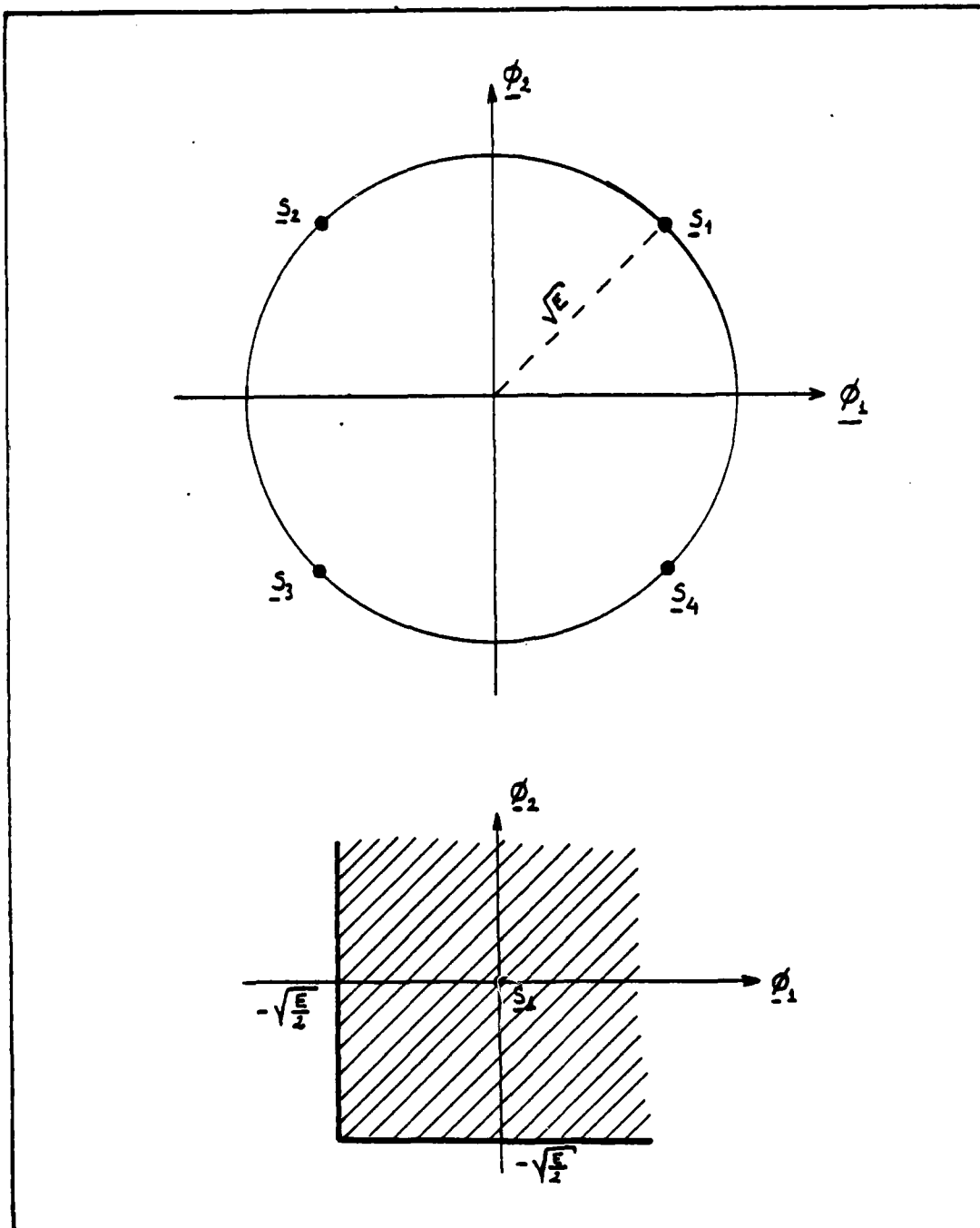
Figure 2.29. Signal-Space Diagram and Decision Regions for QPSK Modulation
