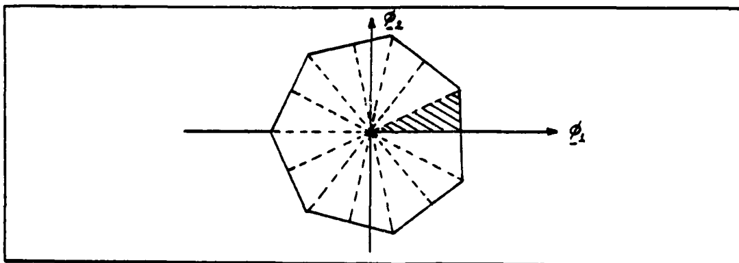
Figure 2.7. Transformed Decision Region for Calculating \Pr\{c/s_8(t)\}
