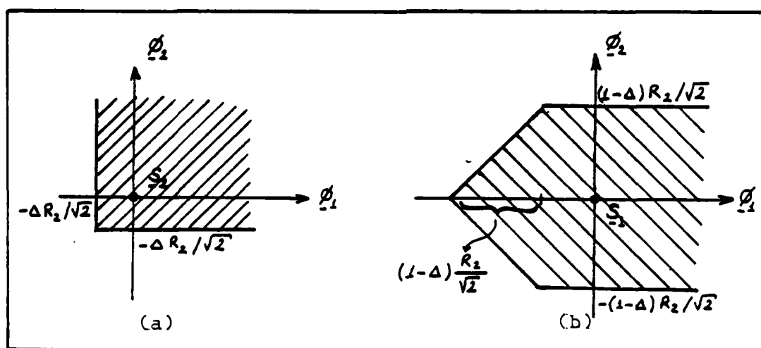
Figure 2.20. Transformed Decision Regions for MOD.2
