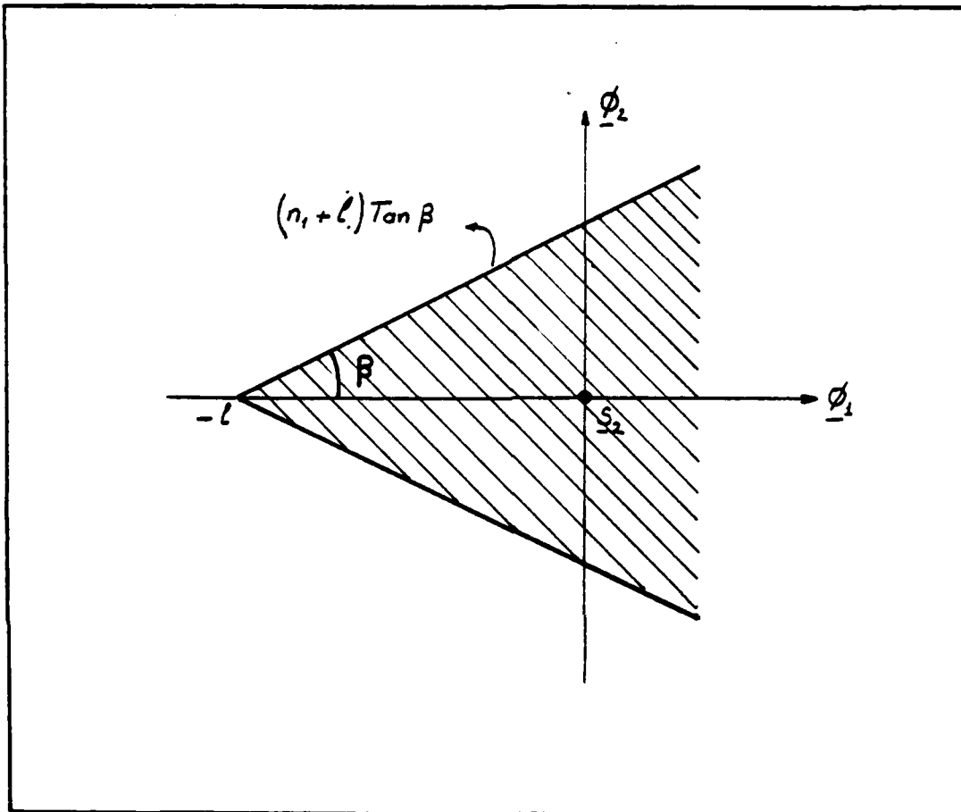
Figure 2.11. Transformed Decision Region for Calculating \text{Pr}\{c/s_2(t)\}
