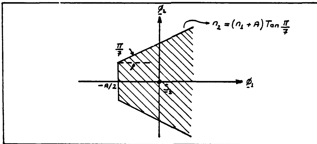
Figure 2.6. Transformed Decision Region for Calculating \Pr\{c/s_1(t)\}
