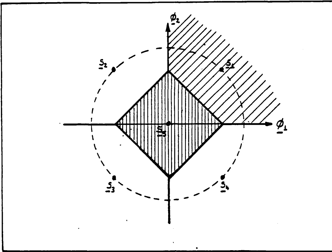
Figure 2.30. Signal-Space Diagram and Decision Regions for (4+1) PSK
