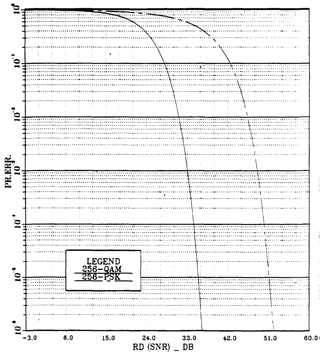
Figure 3.7. \Pr\{\epsilon\} Performance for 256-QAM and PSK
