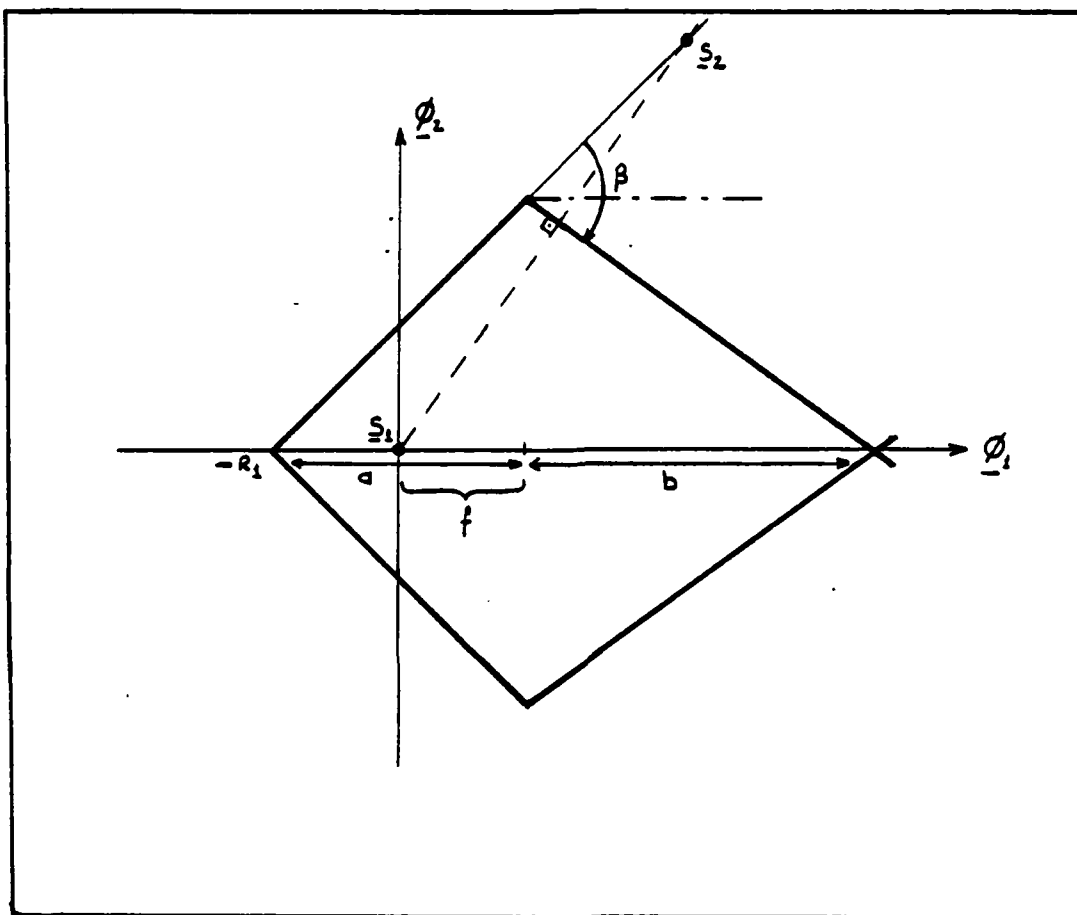
Figure 2.12. Transformed Decision Region for Calculating \Pr\{c/s_1(t)\} ( 45^\circ < \beta < 90^\circ )
