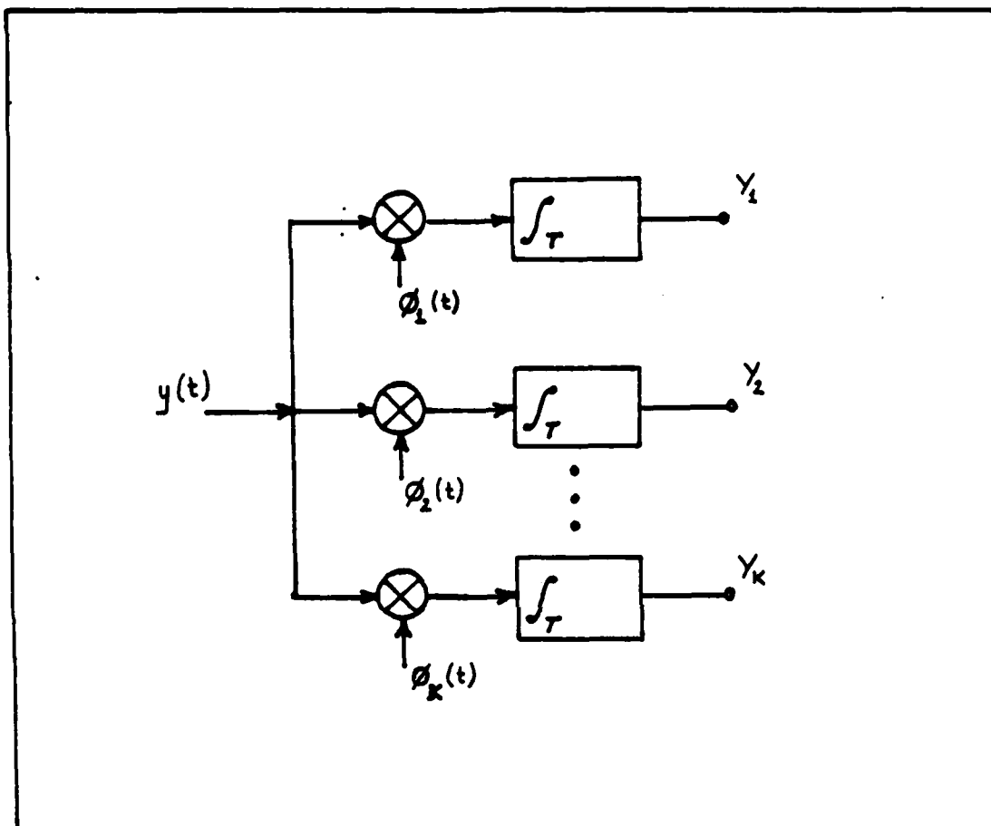
Figure 2.1. Correlator Front End Receiver Structure
