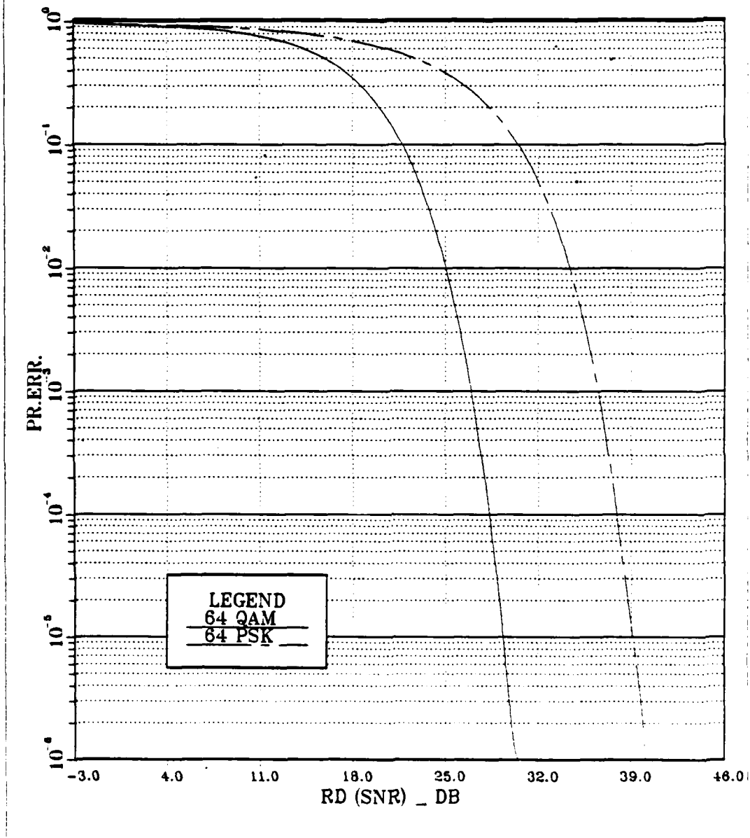
Figure 3.6. Pr\{\epsilon\} Performance for 64-QAM and PSK
