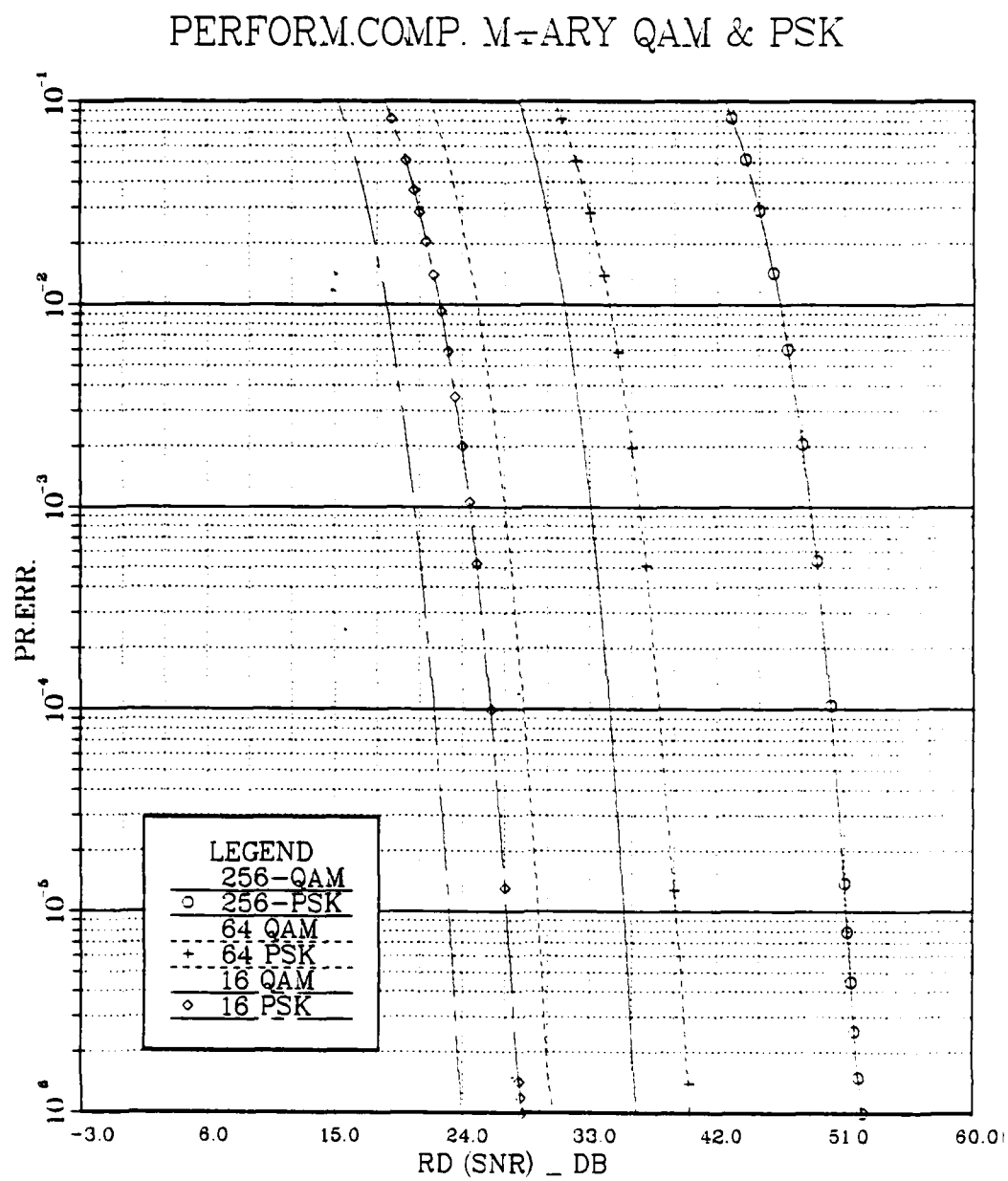
Figure 3.8. Comparison of \Pr(\epsilon) Performance for M-ary QAM and PSK
