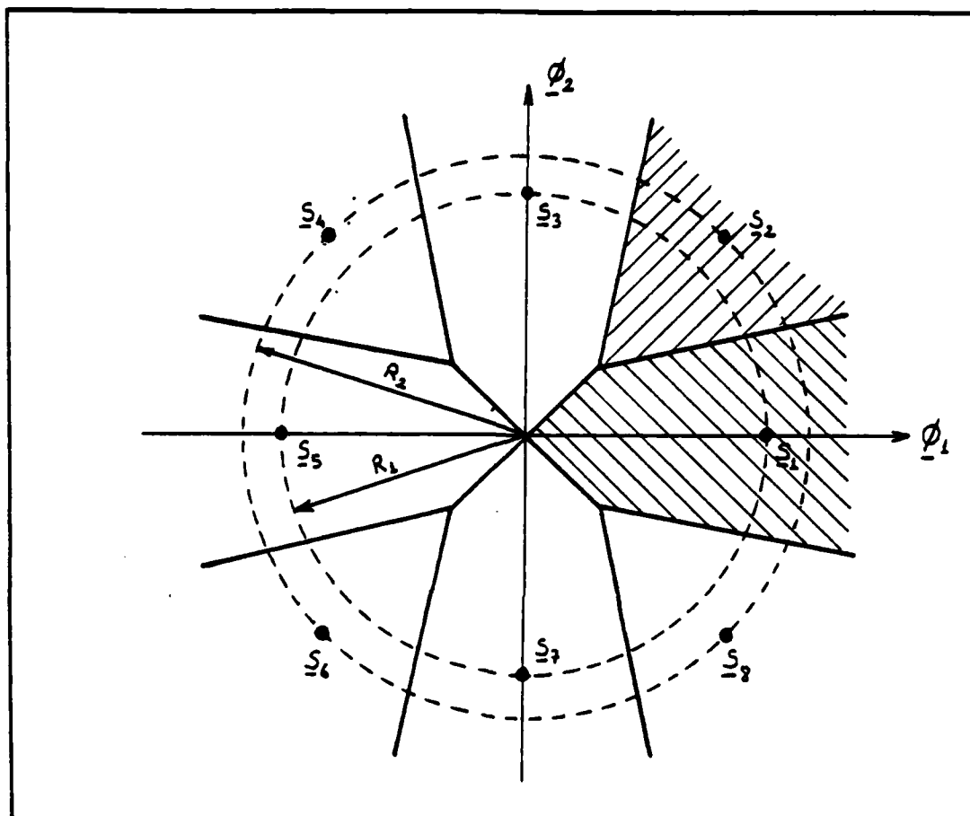
Figure 2.9. Signal-Space Diagram and Optimum Decision Regions for Multi Amplitude MPSK Modulation Systems
