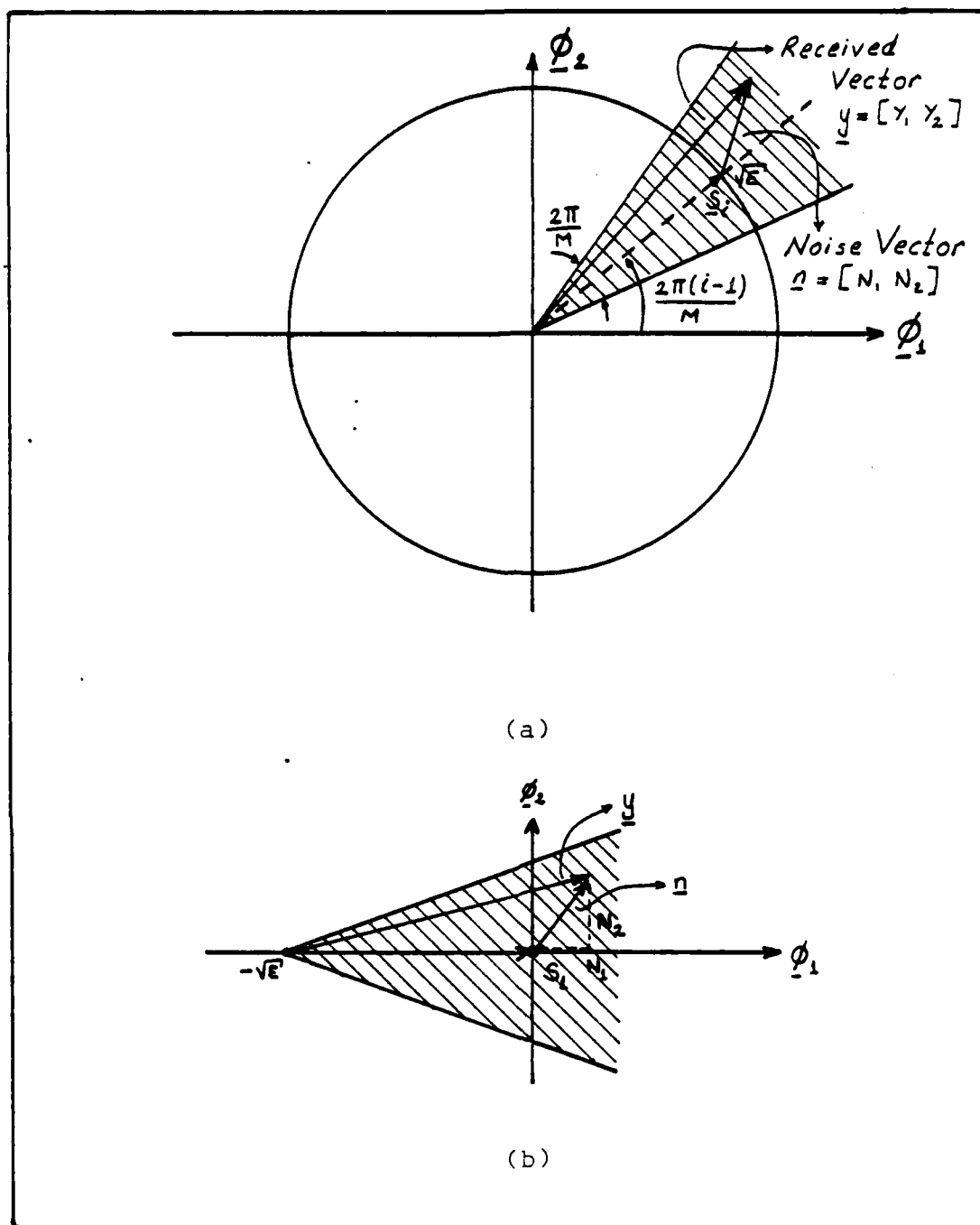
Figure 2.2. a) Signal-Space Diagram for MPSK Modulation b) Decision Region for i th Transmitted Phase
