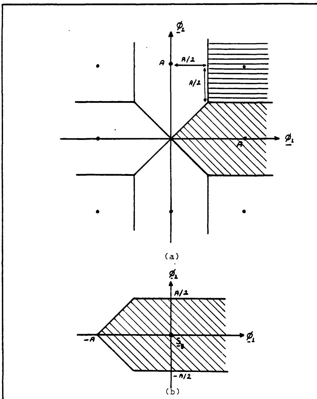
Figure 2.4. a) Decision Regions for Rectangular Signaling Scheme b) Decision Region for Signal s_3(t)
