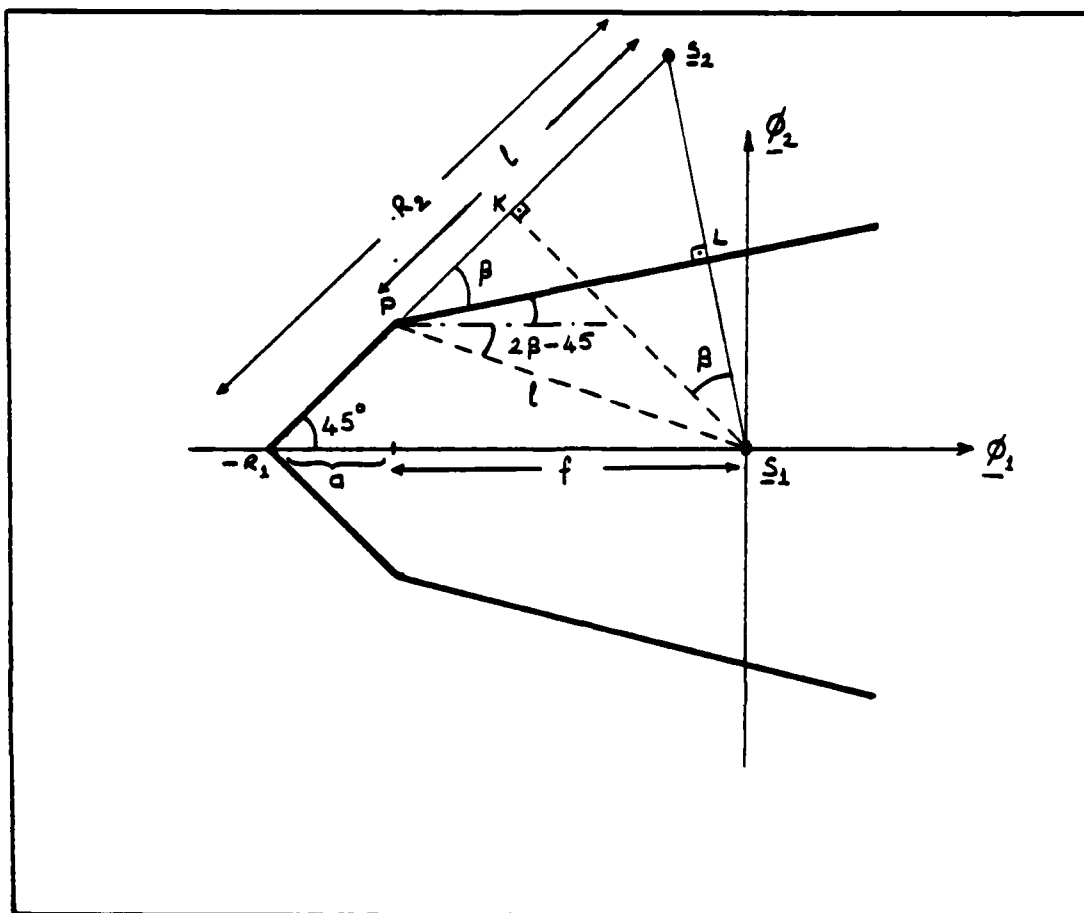
Figure 2.10. Transformed Decision Region for Calculating \Pr(c/s_1(t))
