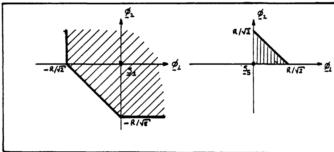
Figure 2.31. Transformed Decision Regions for (4+1) PSK
