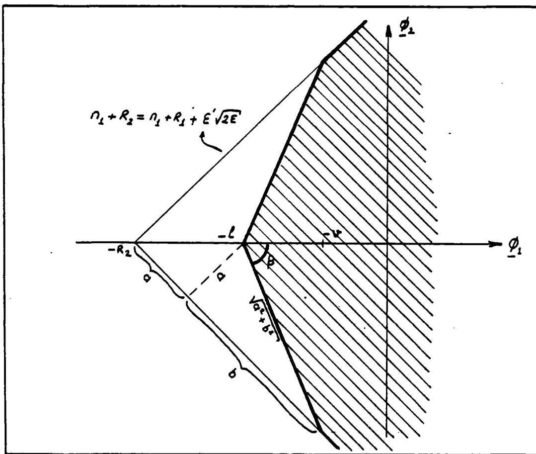
Figure 2.13. Transformed Decision Region for Calculating \Pr(c/s_2(t)) ( 45^\circ < \beta < 90^\circ )
