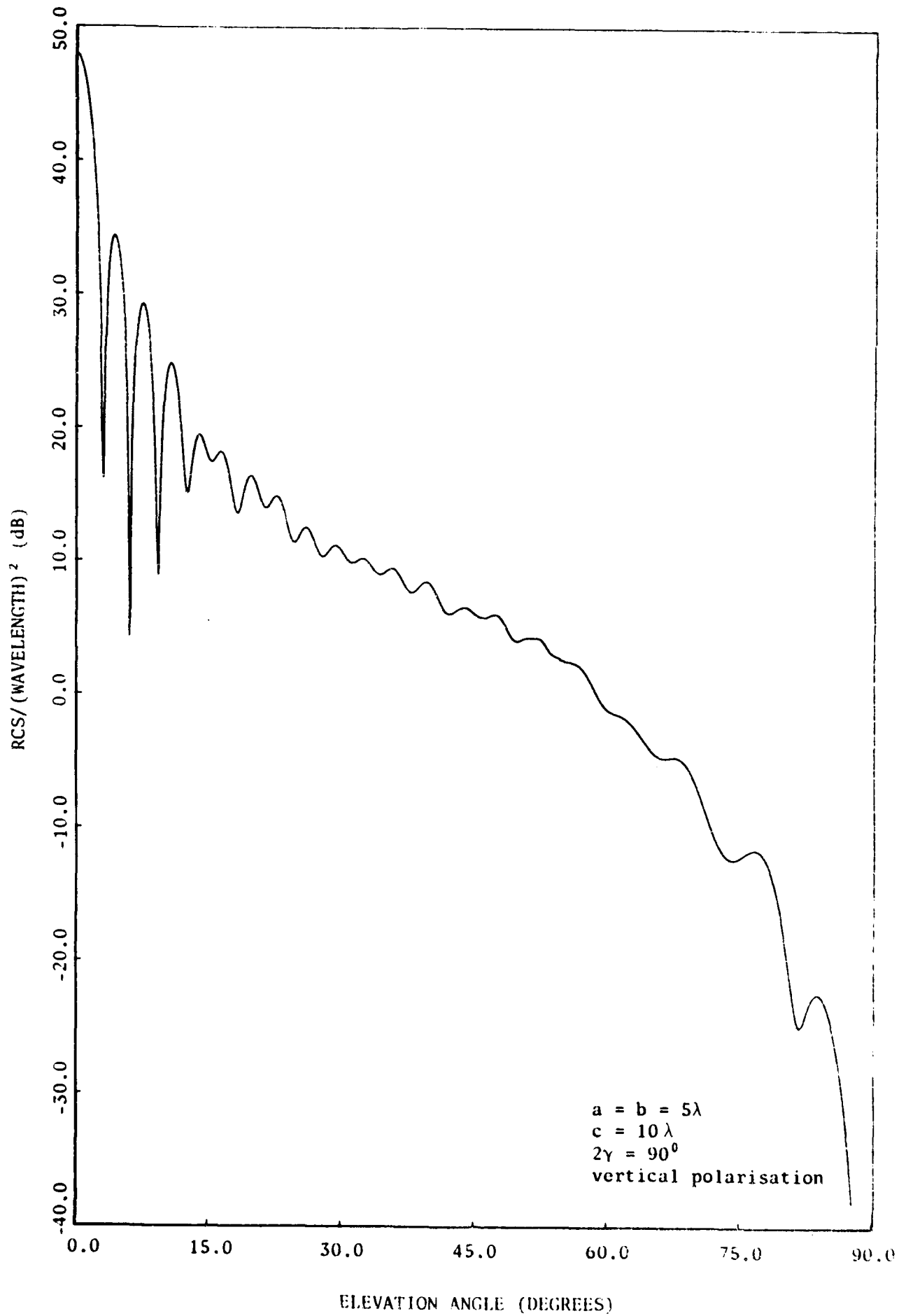
Figure 3. Elevation RCS for \phi = 0^\circ
