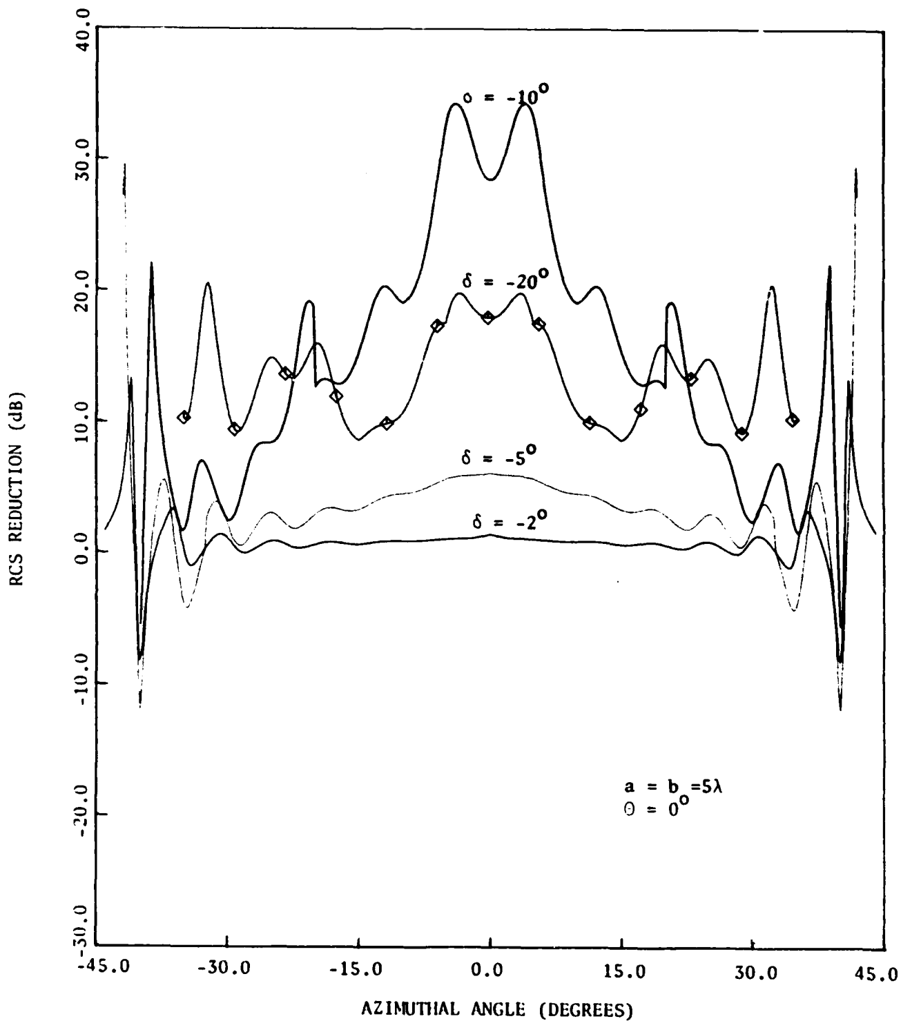
Figure 7. Reduction in RCS for \delta = -2^\circ , -5^\circ , -10^\circ and -20^\circ (horizontal polarisation)
