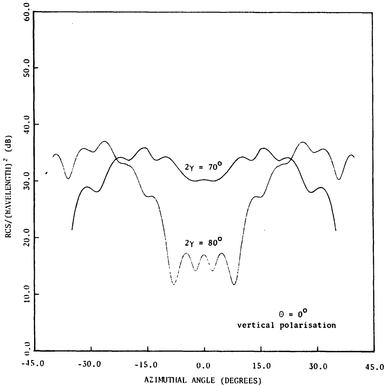
Figure 9. RCS of 70° and 80° reflectors, a = b = 5\lambda , c = 10\lambda
