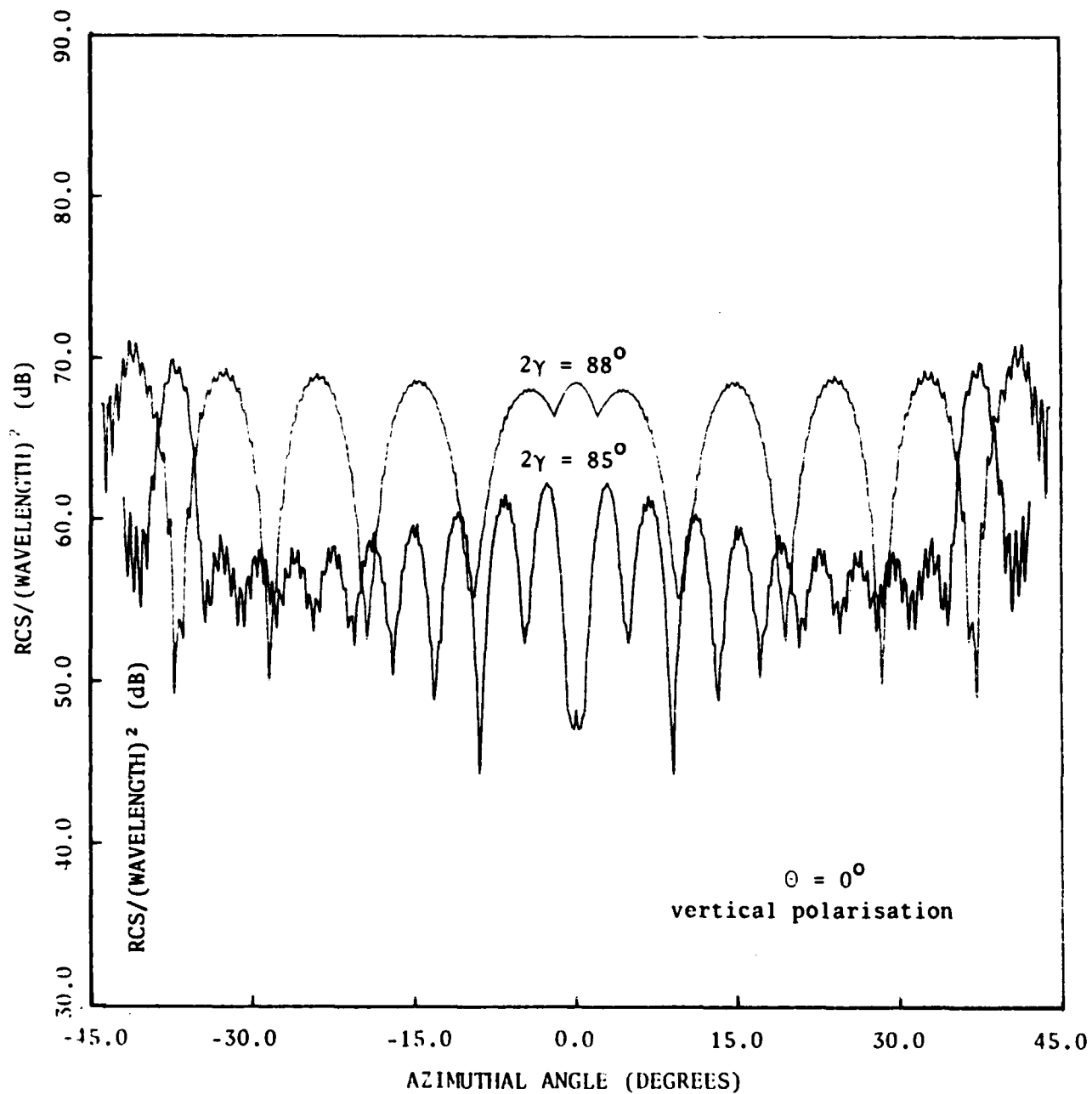
Figure 10. RCS of 85^\circ and 88^\circ reflectors, a = b = c = 100\lambda
