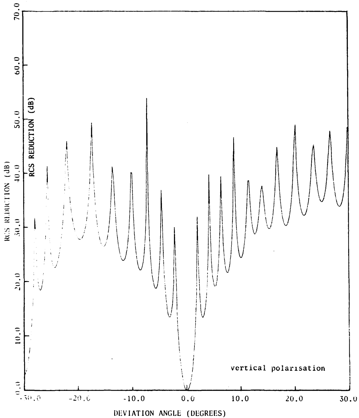
Figure 16. RCS reduction as a function of \delta at \phi = \theta = 0^\circ for a = b = 20\lambda
