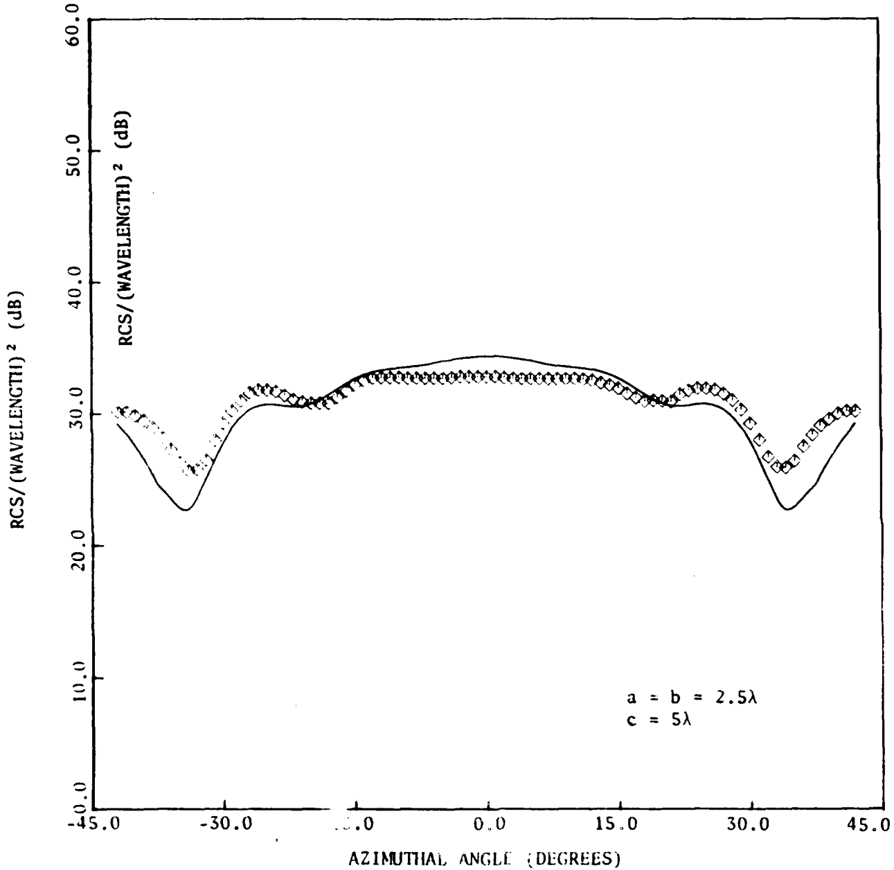
Figure 38. Comparison of theory with experiment for a/\lambda = 2.5 , \theta = 0^\circ , 2\gamma = 85^\circ (vertical polarisation)
