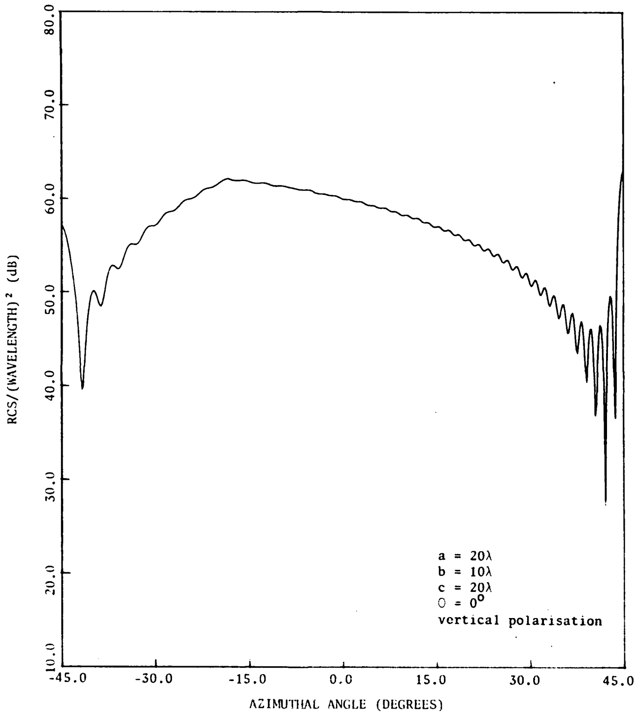
Figure 34. RCS for an asymmetric reflector with reflector angle 90°
