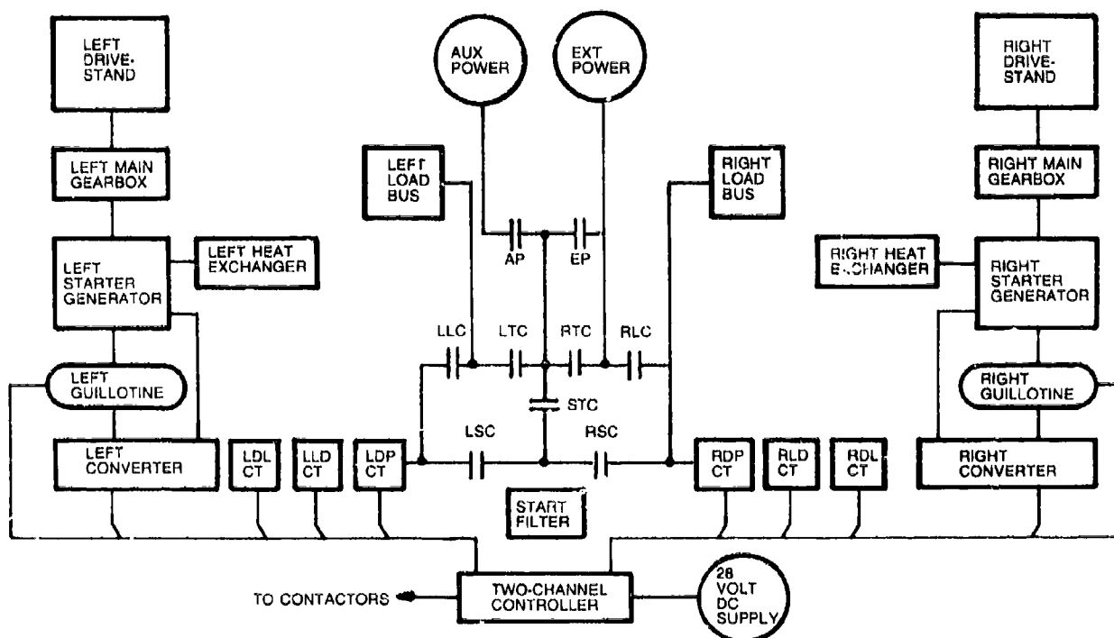
Figure 14. Laboratory Layout
