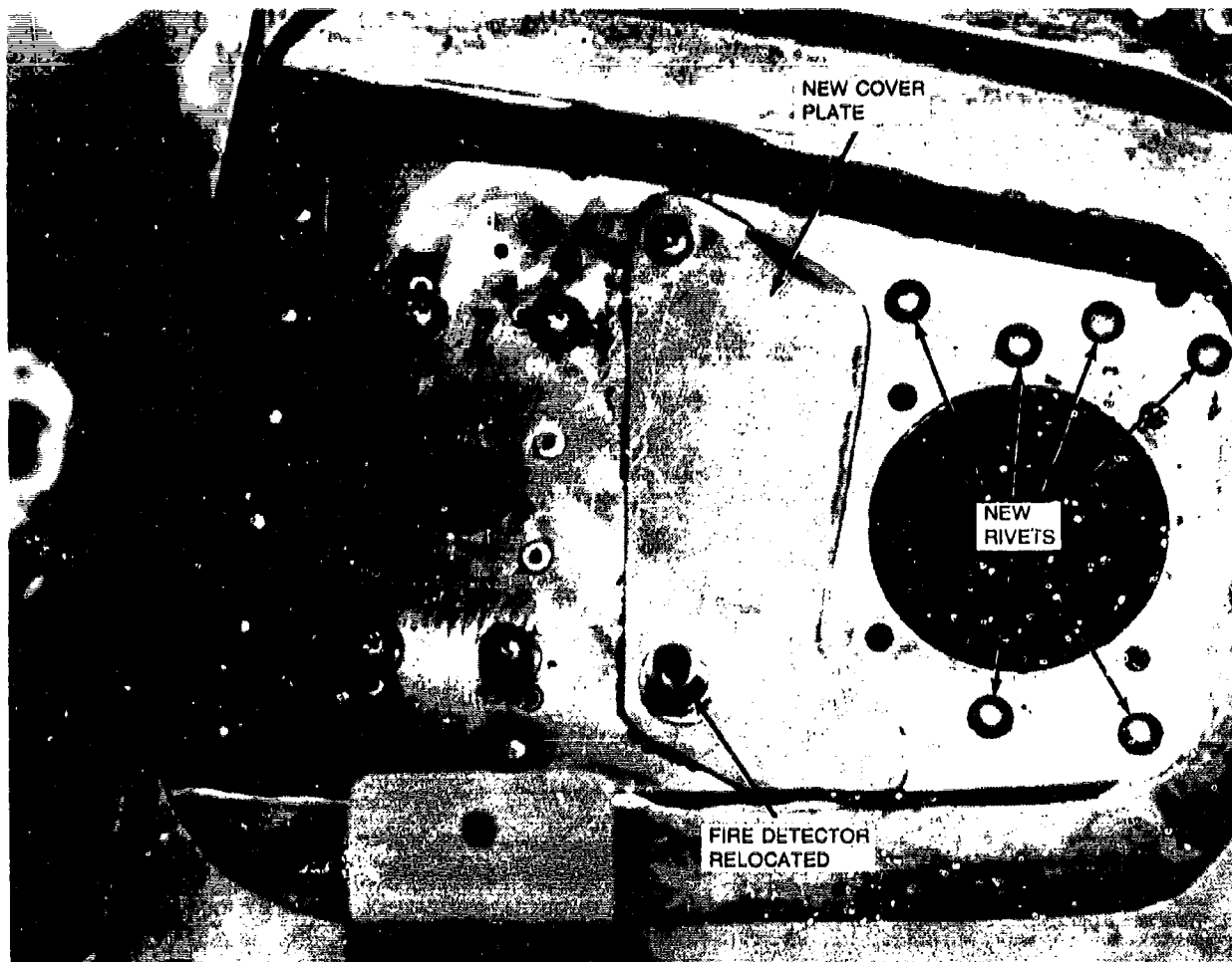
Figure 125. Pylon Floor After GE Modification
