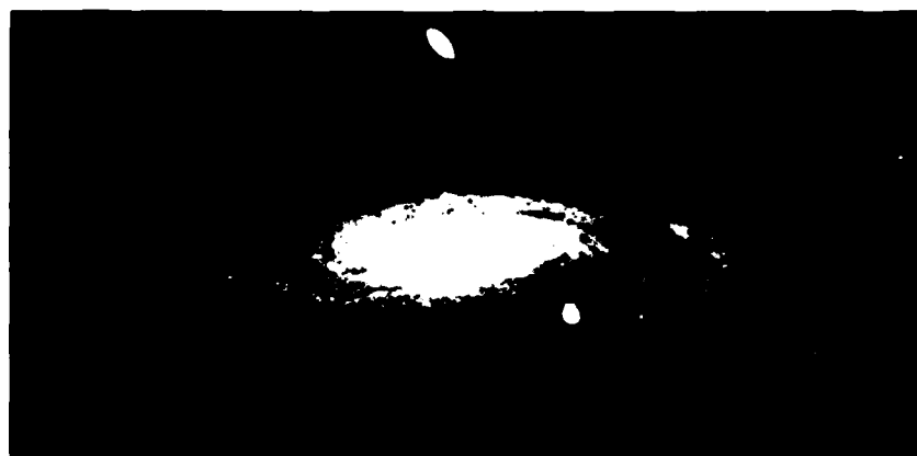
Fig. 20 — IRAS map of M31 at 60 \mu m (top) with the corresponding optical image (bottom). (From Habing et al. , 1984; p. L6 of "IRAS Observations of Radio-Quiet and Radio-Loud Quasars," by G. Neugebauer, published by the University of Chicago Press, copyright (c) 1984, used by permission.)
