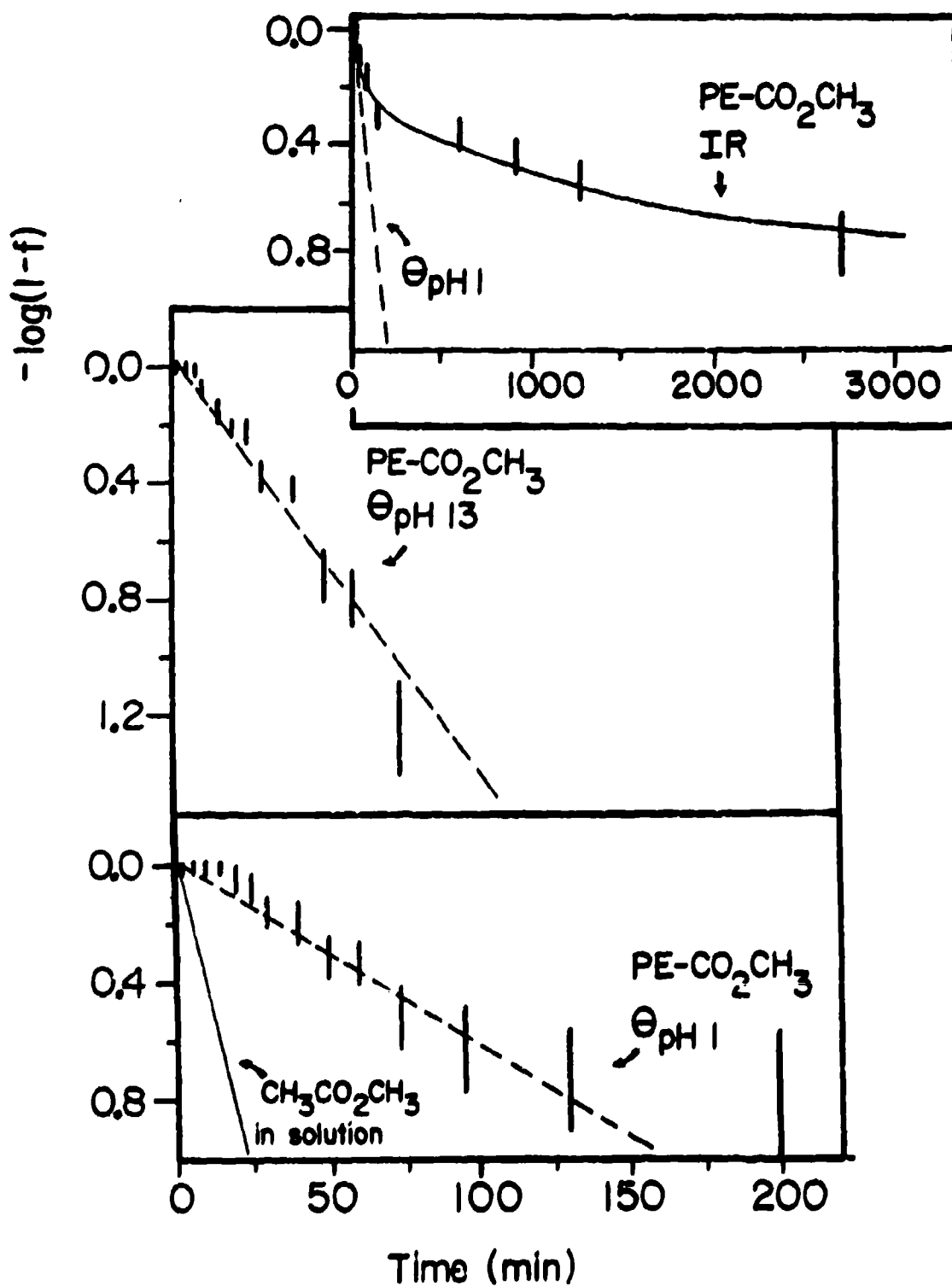
Figure 10. Kinetic plots for f_{\Theta, \text{pH} 1} , f_{\Theta, \text{pH} 13} and f_{\text{IR}} from the data on Figure 8. For comparison, the plot includes data for homogeneous hydrolysis of \text{CH}_3\text{CO}_2\text{CH}_3 under the same conditions. 26
