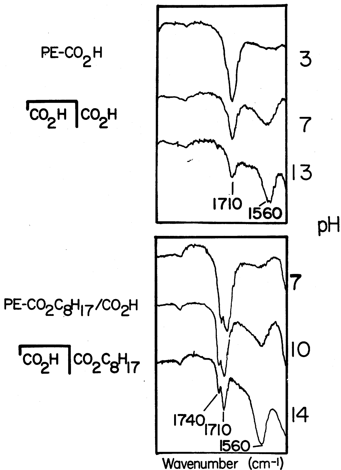
Figure 19. Types of curves used in ATR-IR determinations of \alpha_i vs pH for \text{PE-CO}_2\text{H} and the sub- \theta interphase of partially esterified \text{PE-CO}_2\text{H} using octanol (Figure 12, lot t = 3.2).
