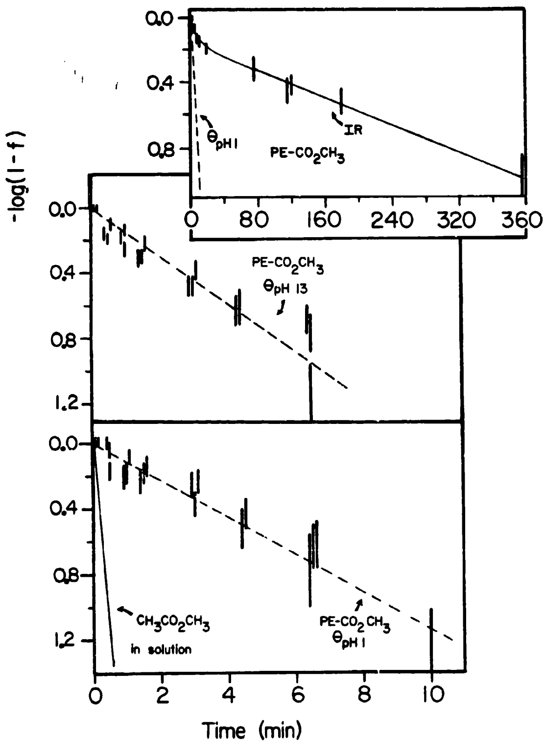
Figure 9. First-order kinetic plots for f_{\theta, \text{pH } 1} , f_{\theta, \text{pH } 13} and f_{\text{IR}} from the data of Figure 7. For comparison, the plot includes data for homogeneous hydrolysis of \text{CH}_3\text{CO}_2\text{CH}_3 under the same conditions. 25
