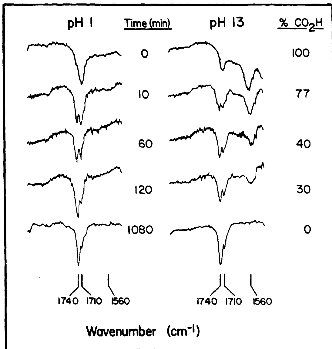
Figure 3. Representative ATR-IR spectra of PE-CO 2 H taken after treatment of the film with acid (pH 1) or base (pH 13) obtained during acid-catalyzed esterification of the carboxylic acid groups in methanol. The absorption at 1560 cm -1 is due to the CO 2 - group, and was the peak followed in determining the extent of reaction. The ester absorption occurs at 1740; the peak at 1710 includes both carboxylic acid and ketone groups.
