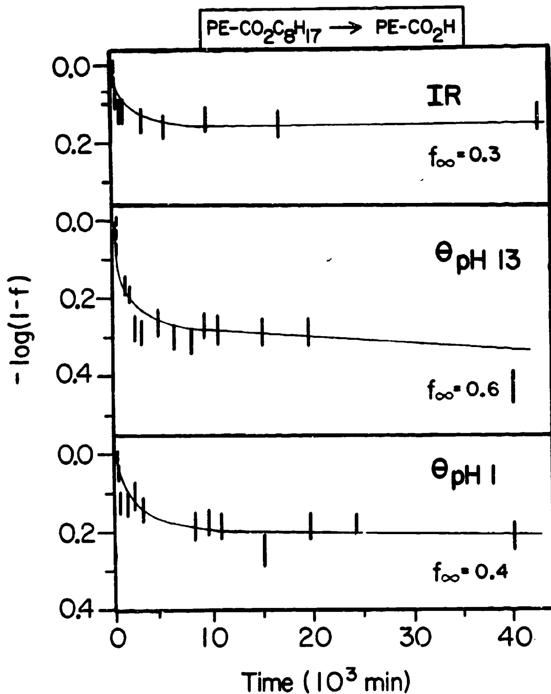
Figure 15. First-order kinetic plots for f_\theta and f_{\text{IR}} for the base-catalyzed hydrolysis of \text{PE-CO}_2\text{C}_8\text{H}_{17} using the data in Figure 13. The values of f reached after 3 weeks in base (30,000 min) are indicated on the figure. Beyond this point, little reaction takes place up to >80,000 min.
