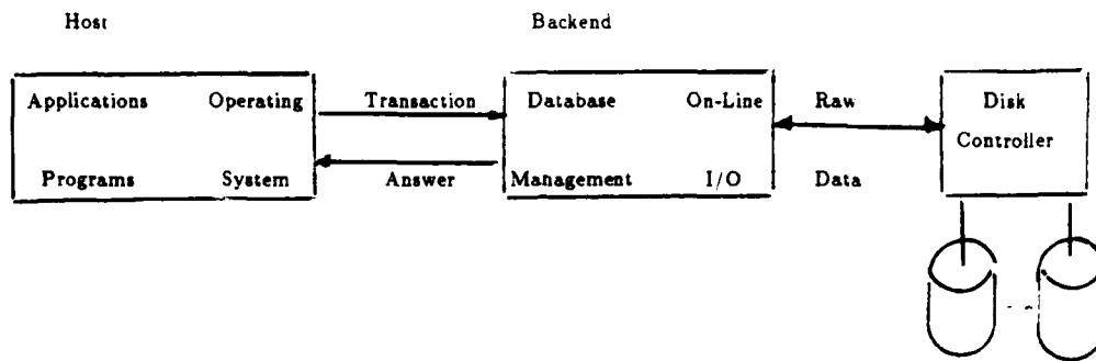
Figure 2. The Software Single-Backend Approach to Database Management
