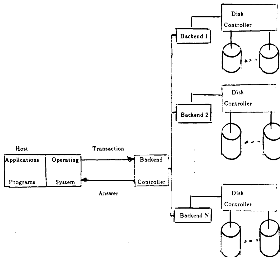
Figure 3. The Software Multiple-Backend Approach to Database Management
