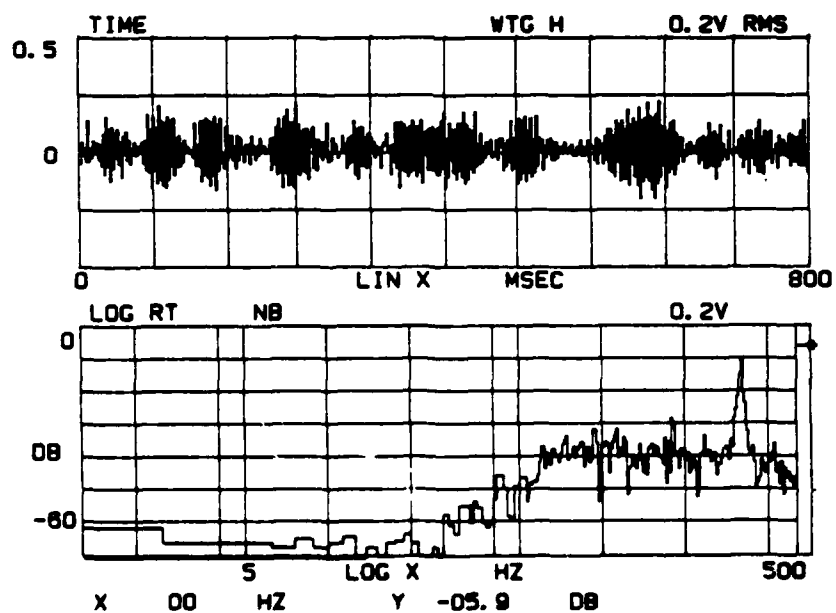
Figure 5.9f. FM Channel 10
