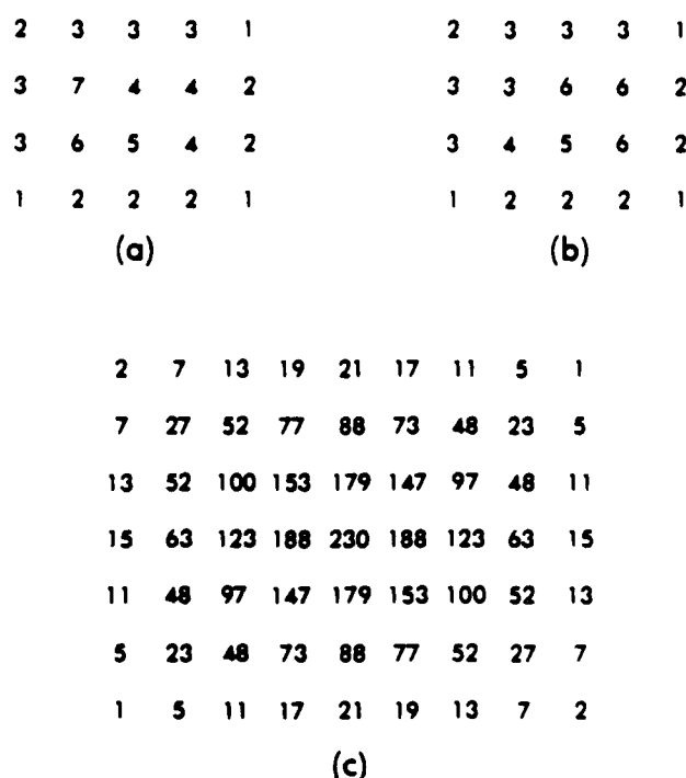
Fig. 1. Example 1. Two different objects, (a) and (b), have the same boundary values and also have the same Fourier modulus (not shown) and the same autocorrelation (c).
